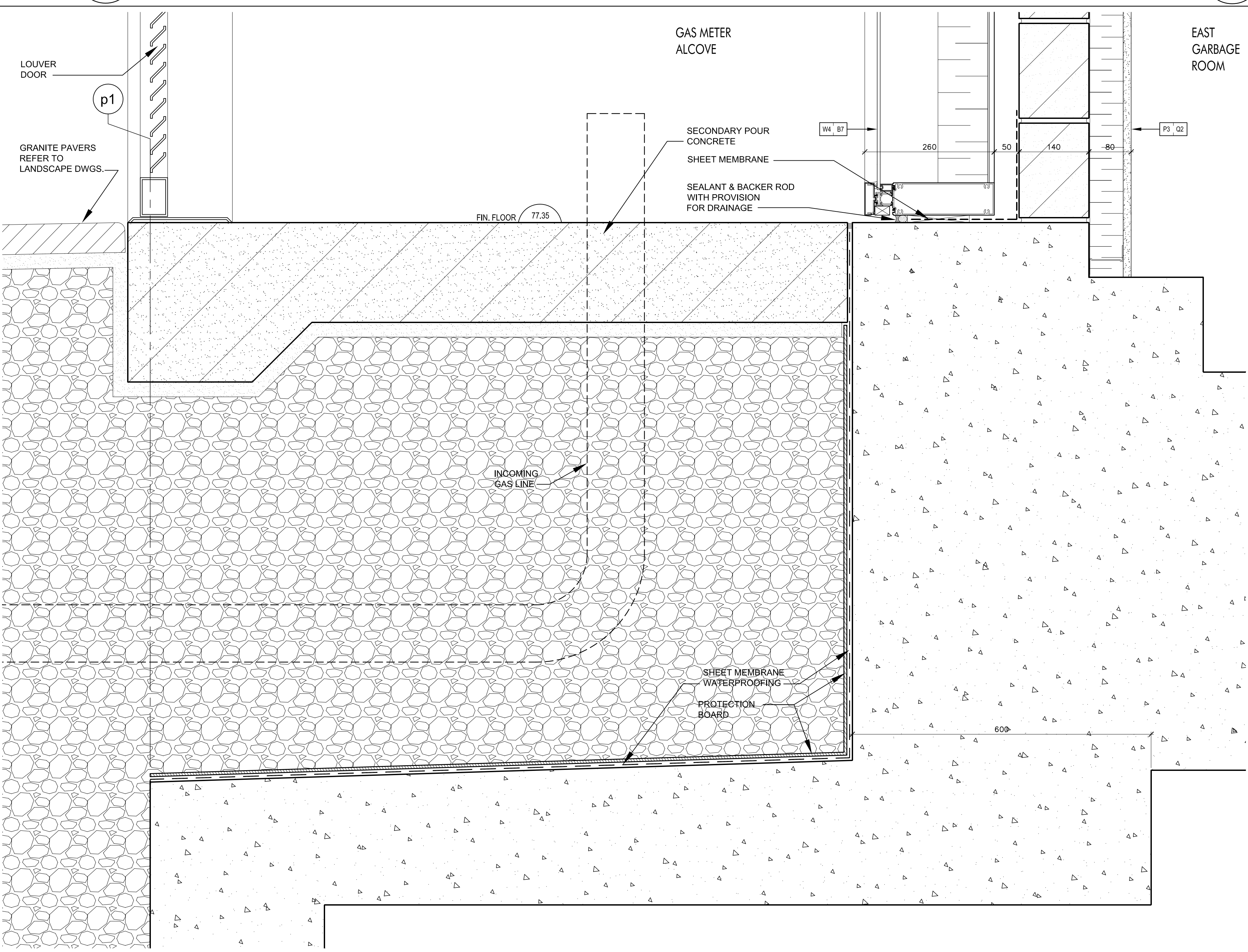
Curtain Wall Sill @ Gas Meter Alcove 9 SCALE 1:5 A7-02
