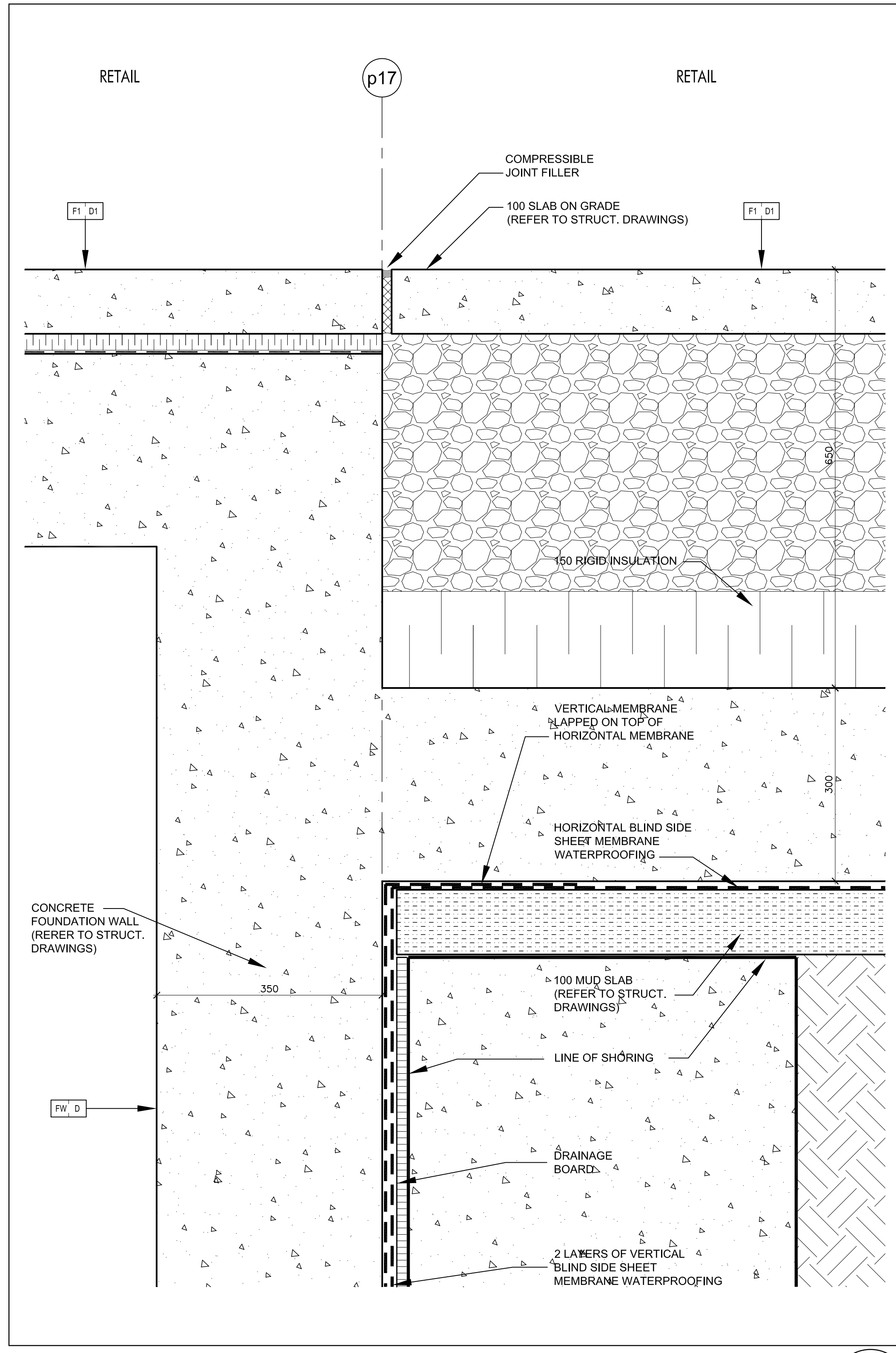
Foundation Wall @ Caisson Wall 8 SCALE 1:5 A7-08
