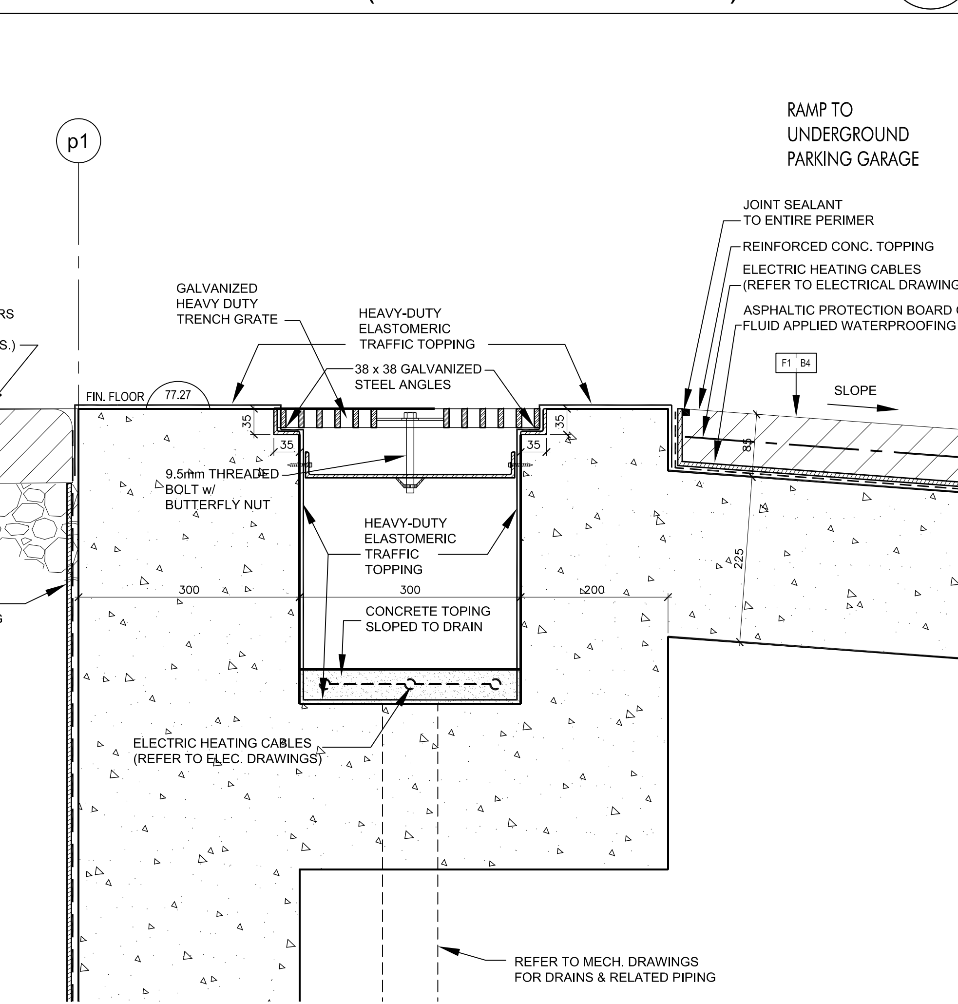
Entrance to Residential Parking 1 SCALE 1:5 A7-08
