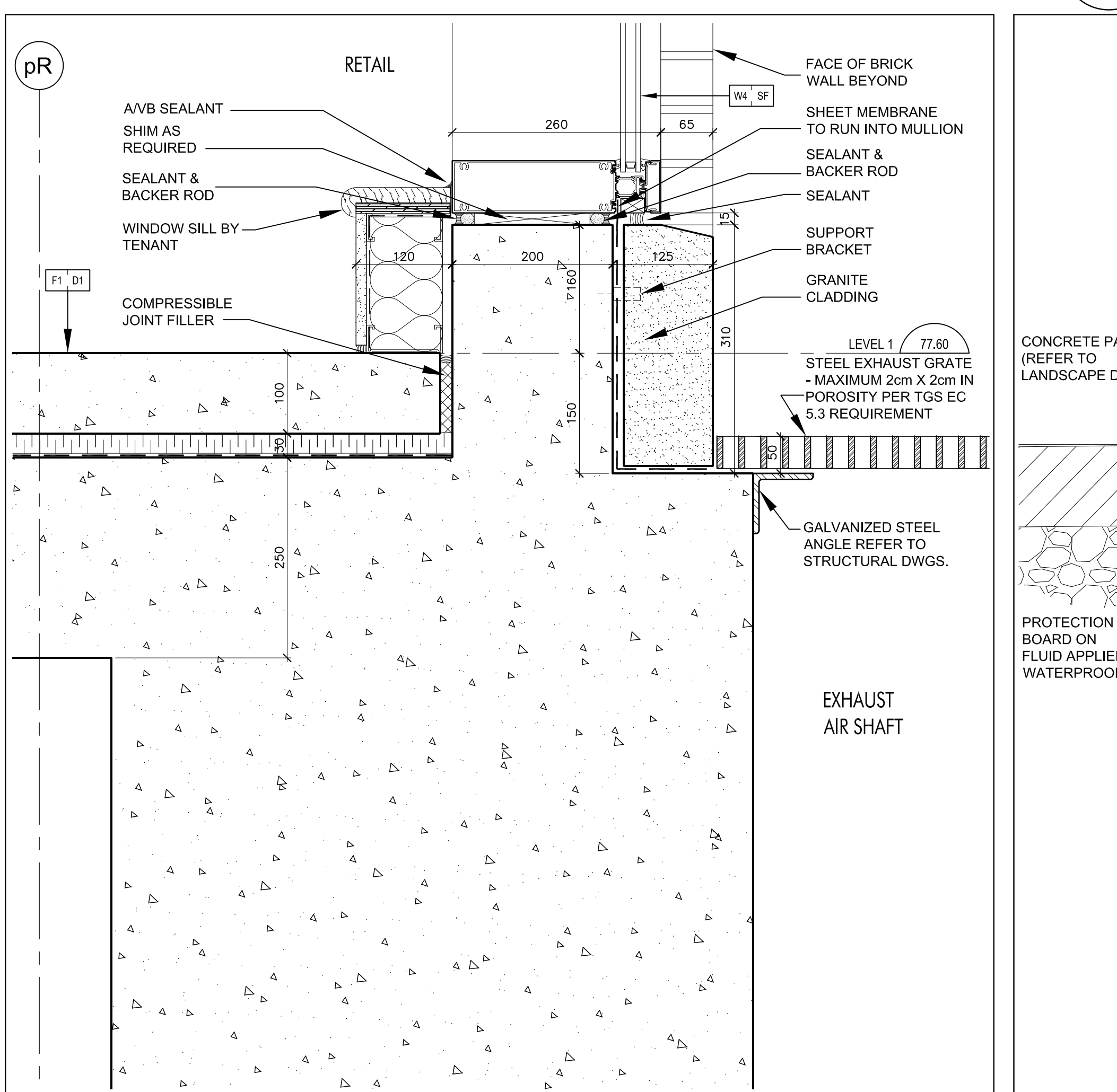
Curtain Wall Sill @ Retail & Steel Grate 4 SCALE 1:5 A7-08
