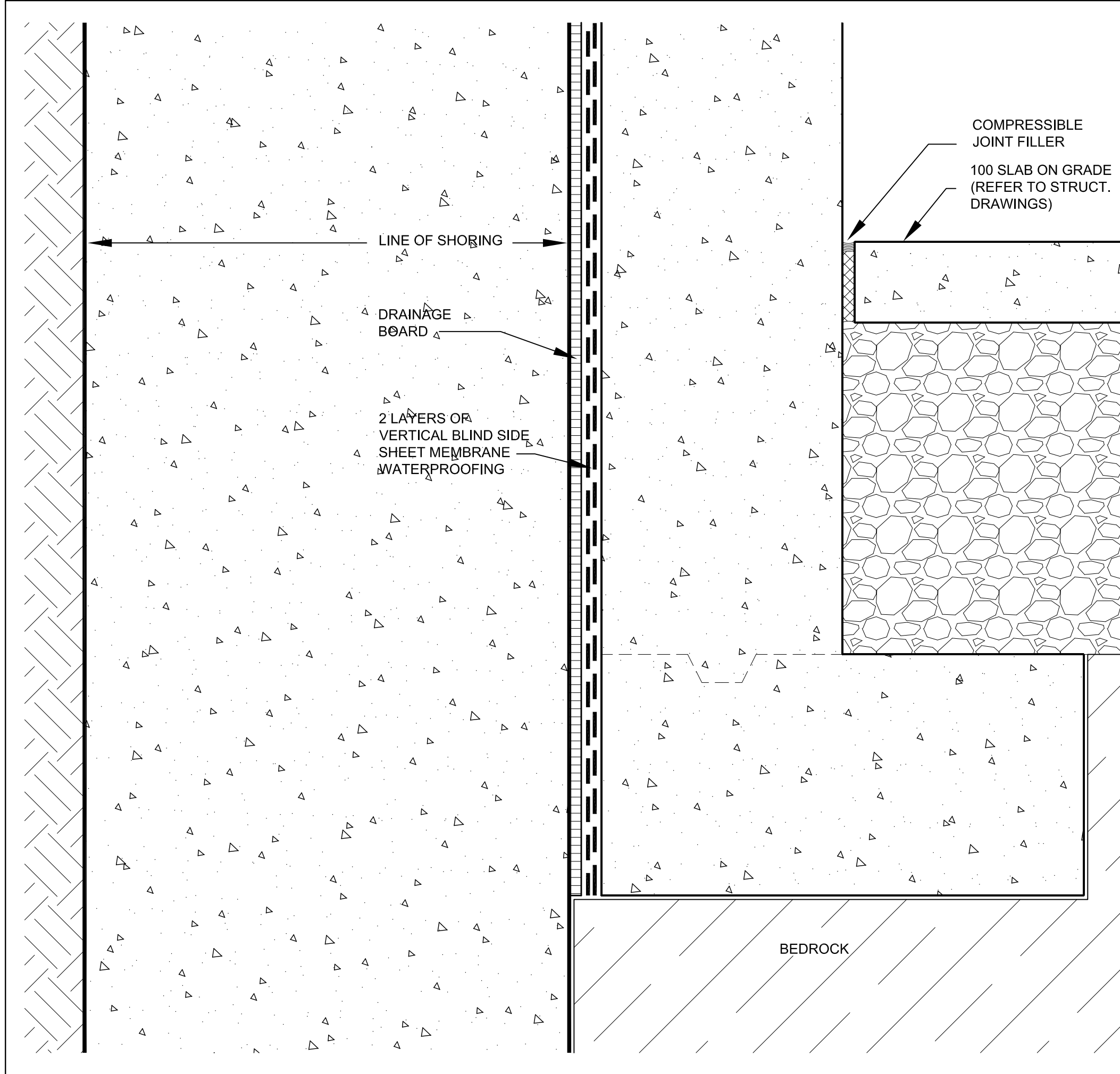
Foundation Wall @ Caisson Wall 5 SCALE 1:5 A7-08
