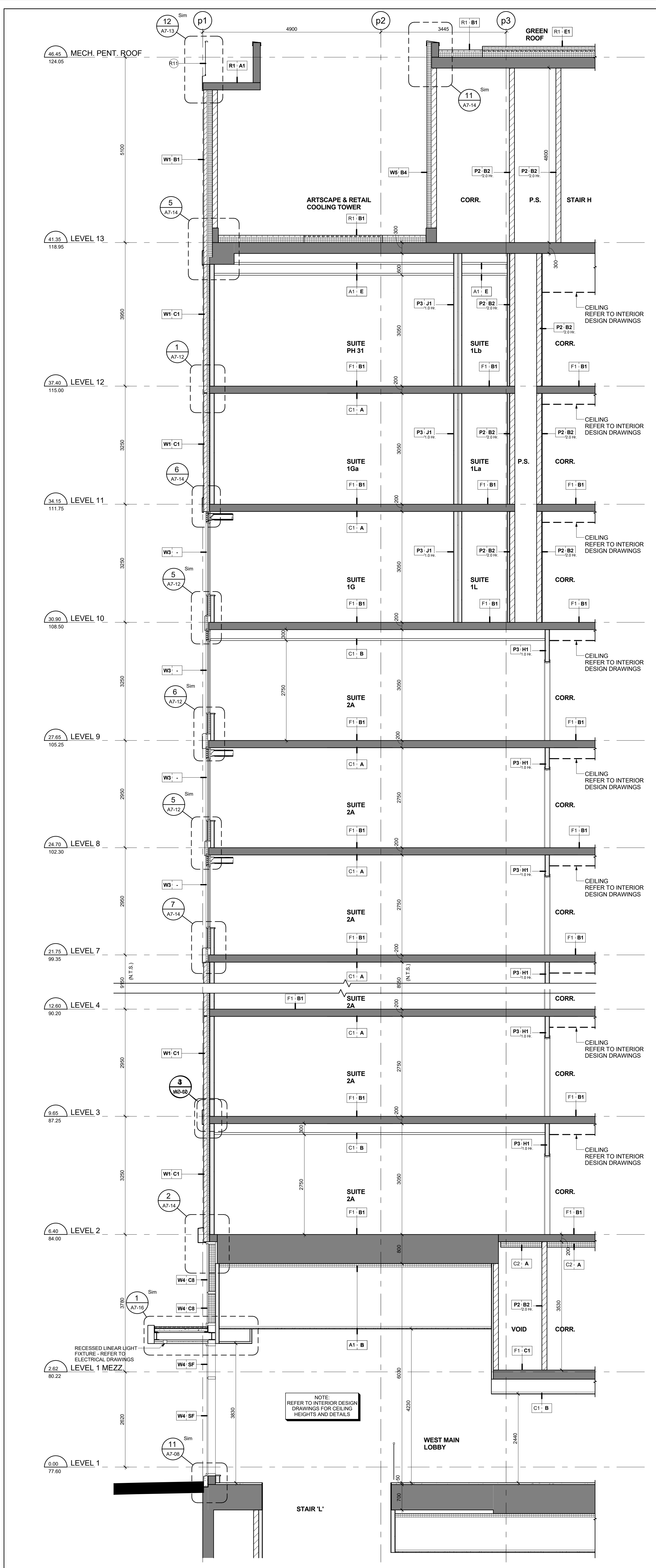
Section between Grids C & D North Side Scale: 1 : 50 A7-01
