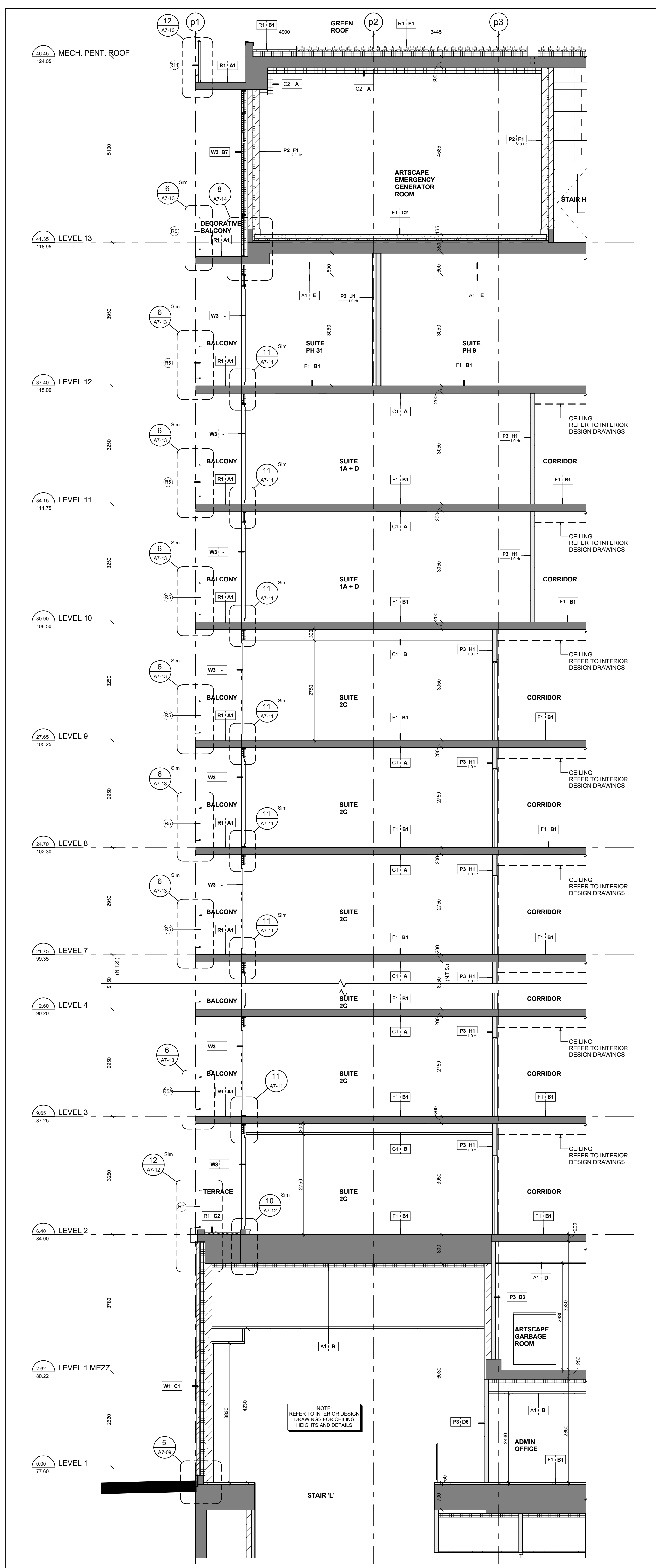
Section between Grids E & F North Side Scale: 1 : 50 A7-01
