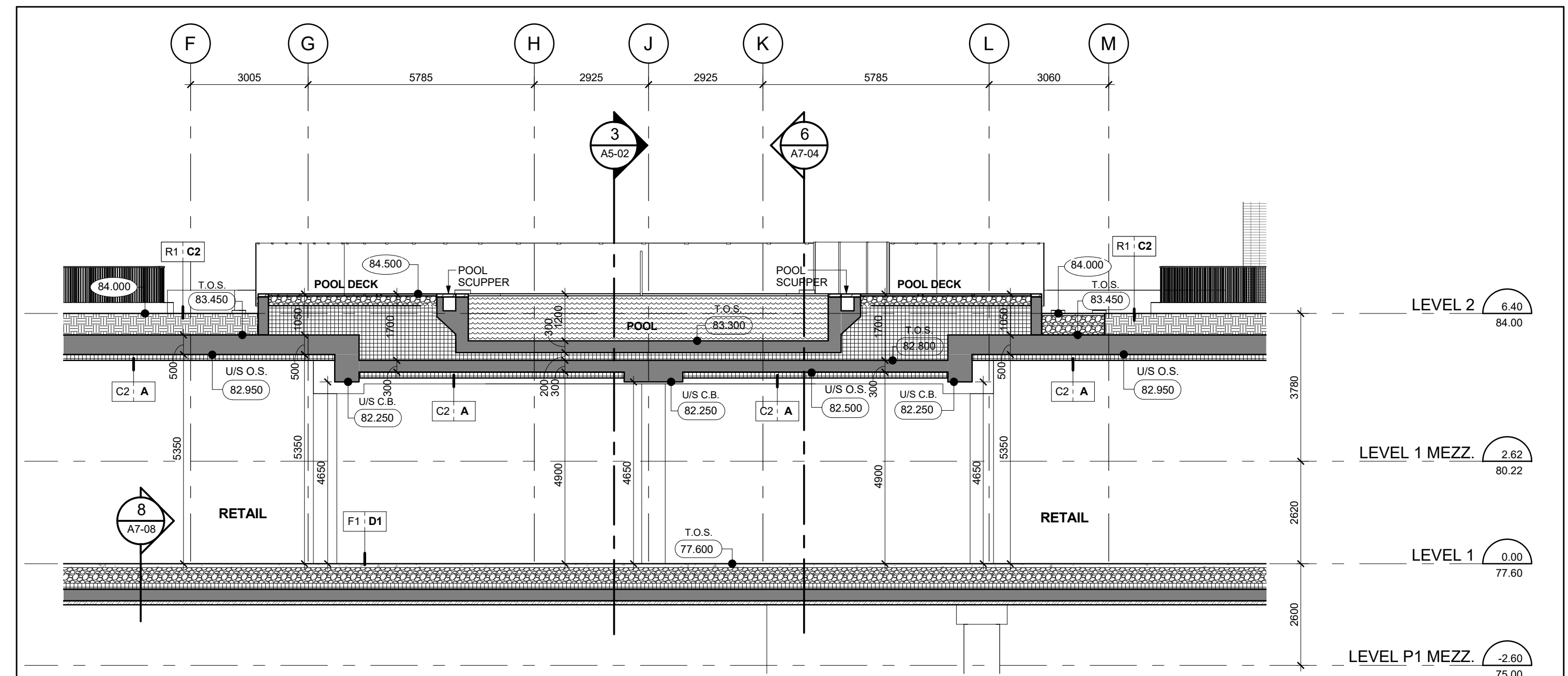
East - West Pool Section Along Gridline p17 4 A5-02 Scale: 1 : 100
