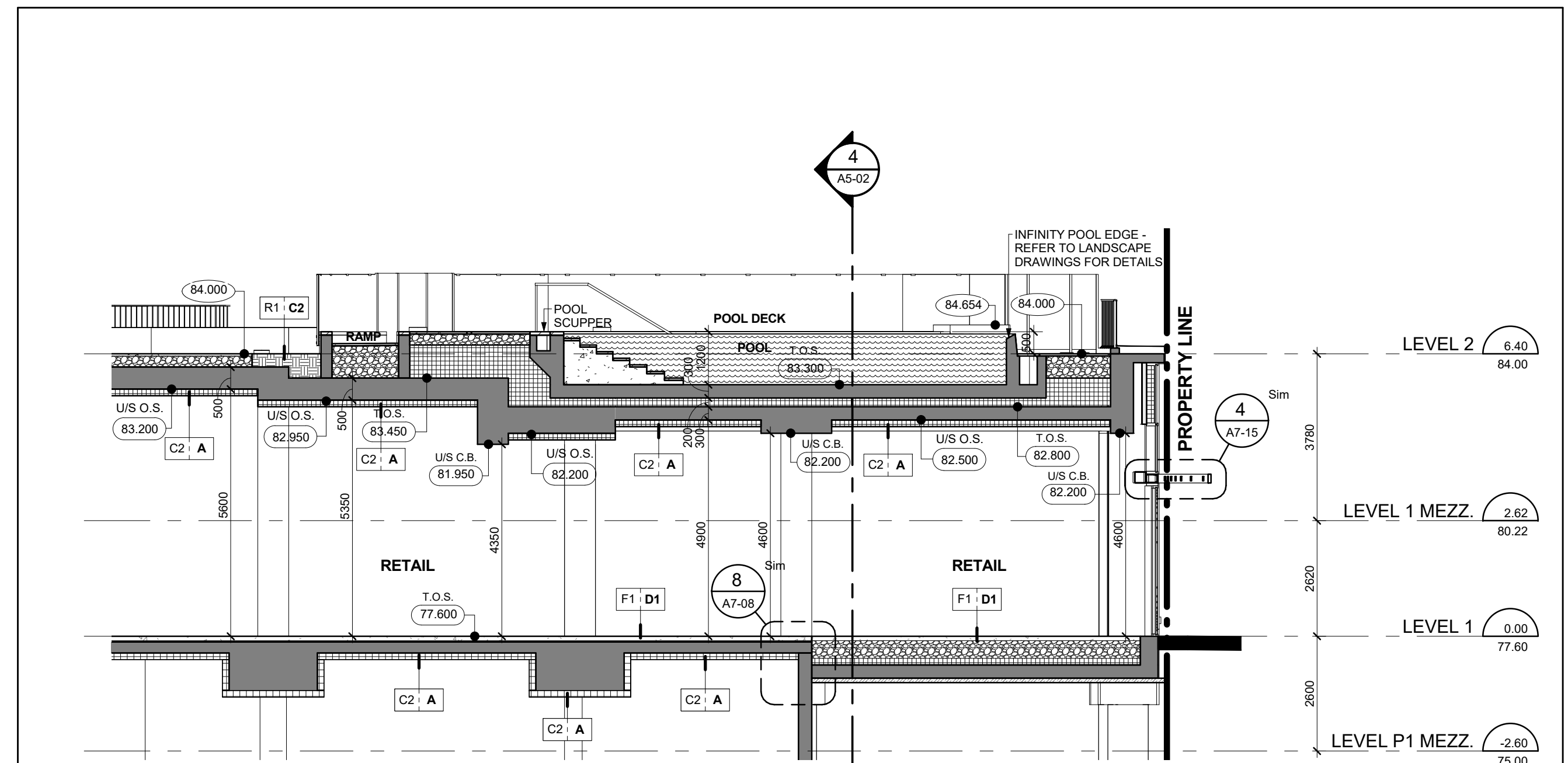
North - South Pool Section Along Gridline J 3 A5-02 Scale: 1 : 100
