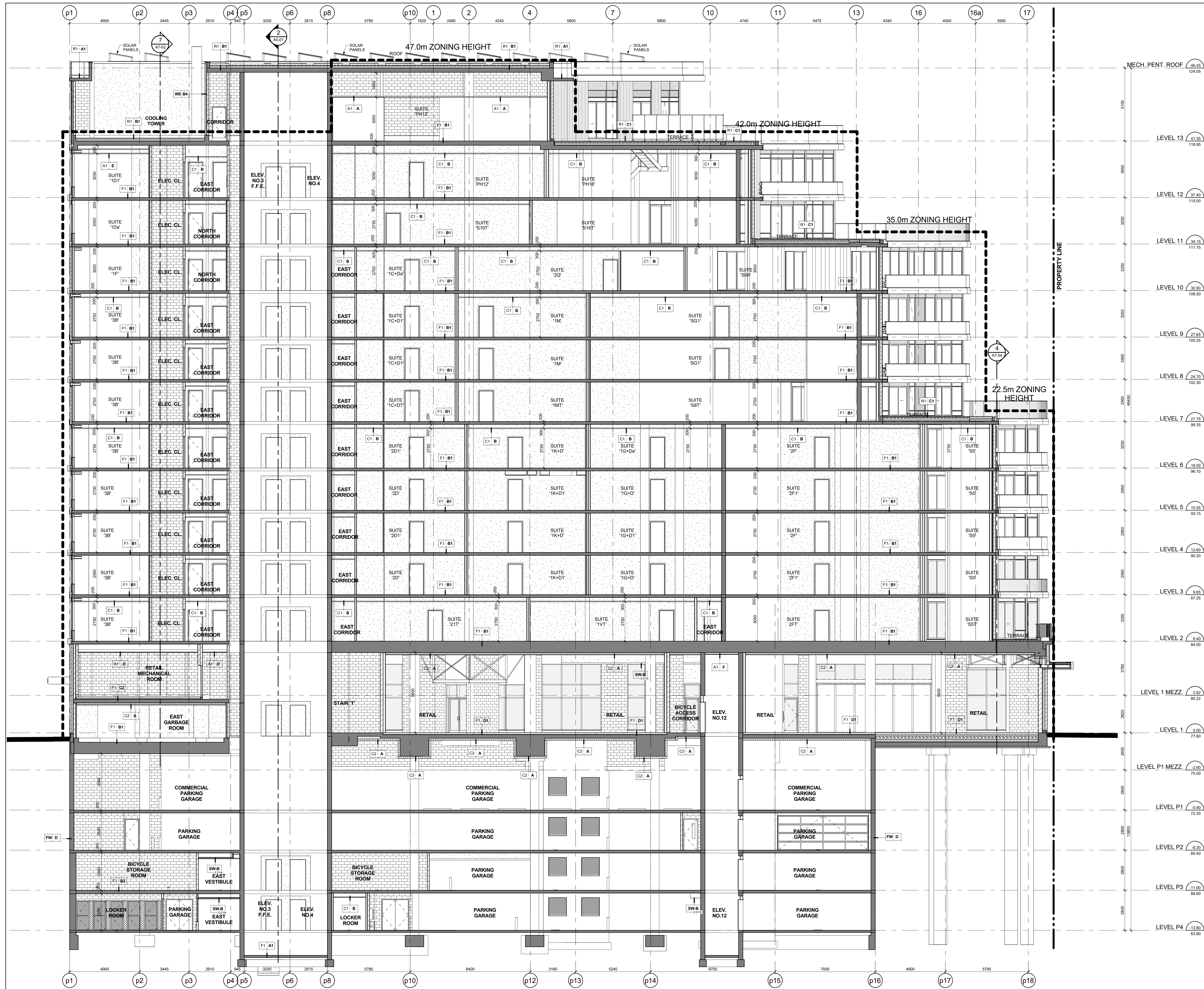
North - South Building Section Along Gridline pP 1 A5-02 Scale: 1 : 100
