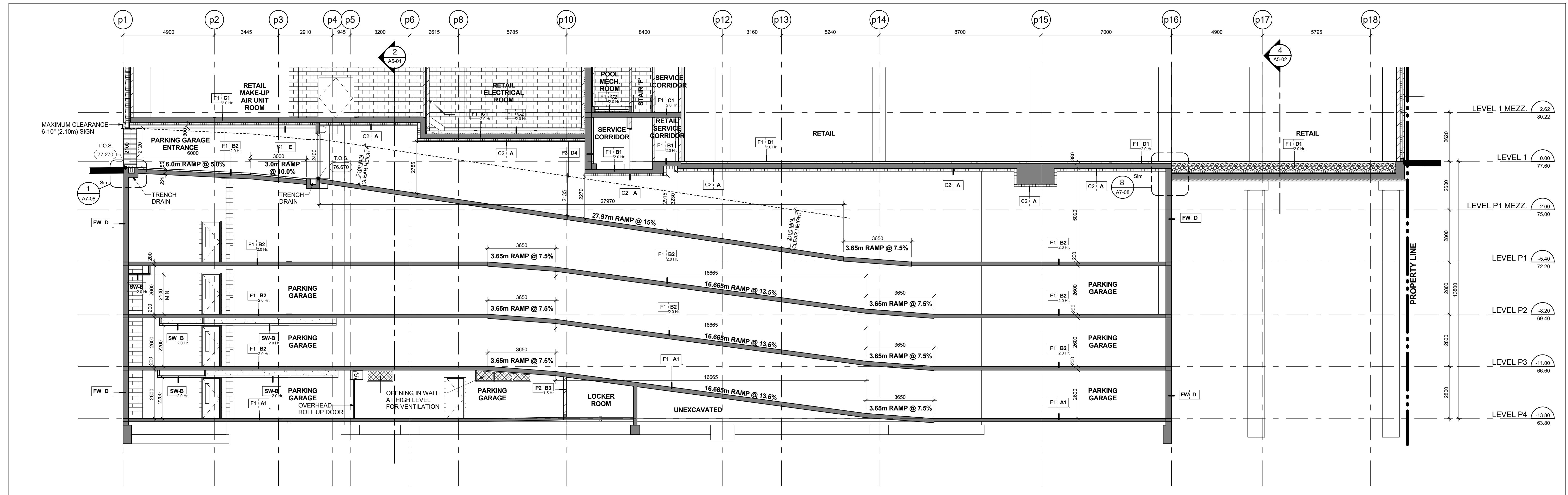
North - South Ramp Section Along Gridline pL 2 A5-02 Scale: 1 : 100
