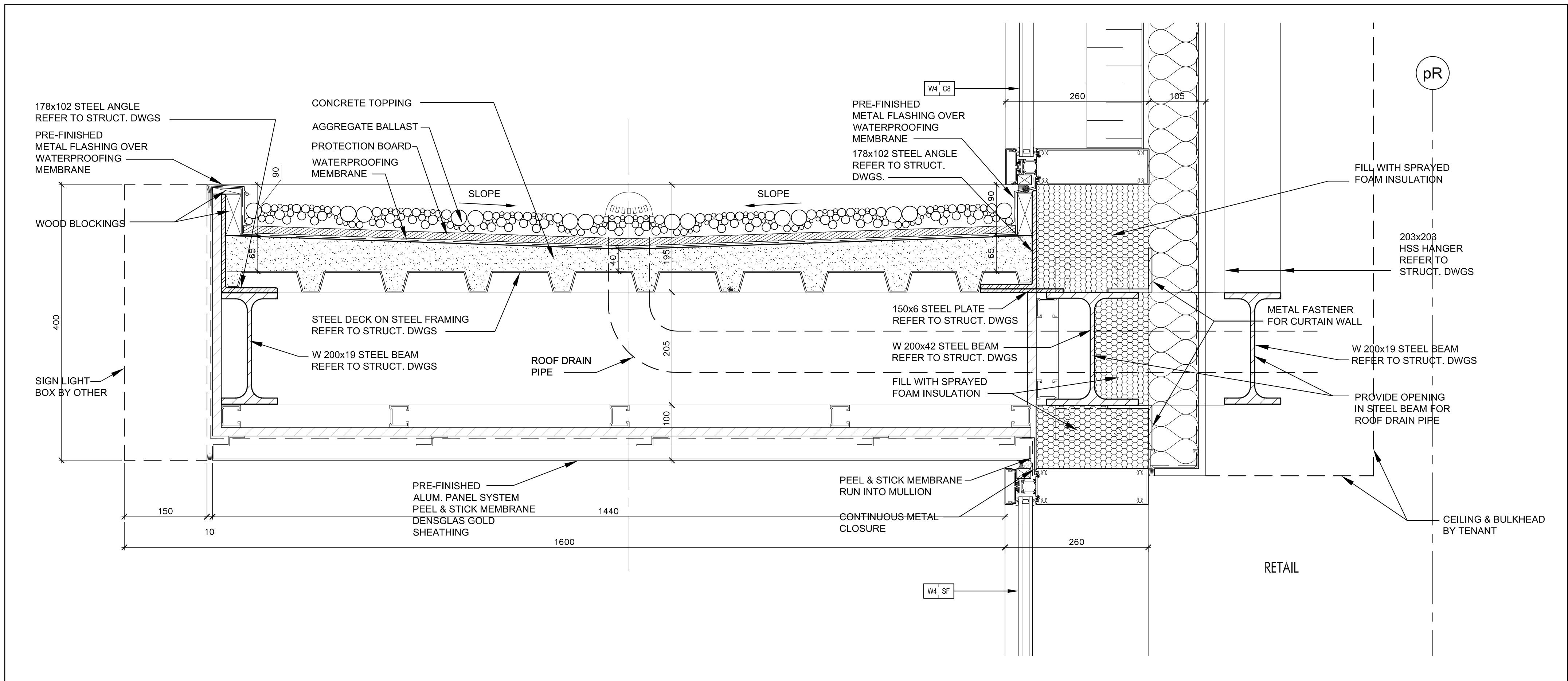
Pre-Finished Aluminum Canopy @ Retail @ Level 1 SCALE 1:5 A7-16
