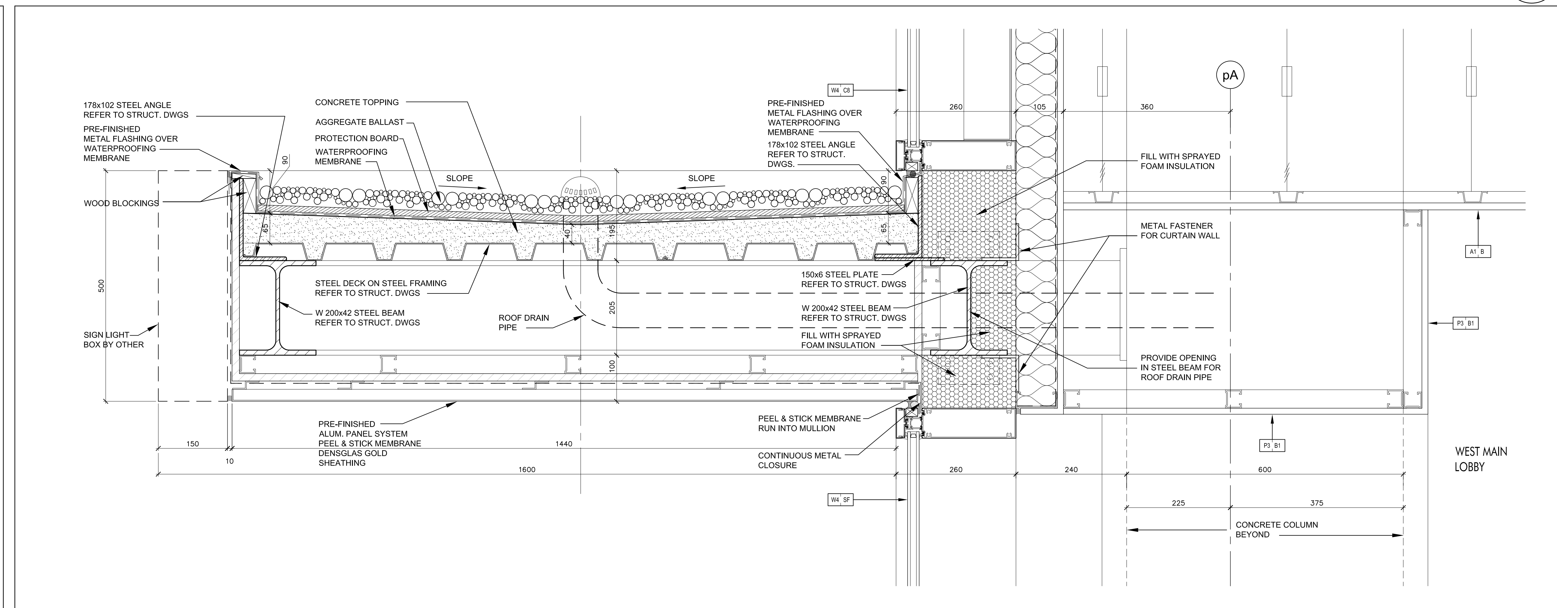
Pre-Finished Aluminum Canopy @ West Main Lobby @ Level 1 SCALE 1:5 A7-16
