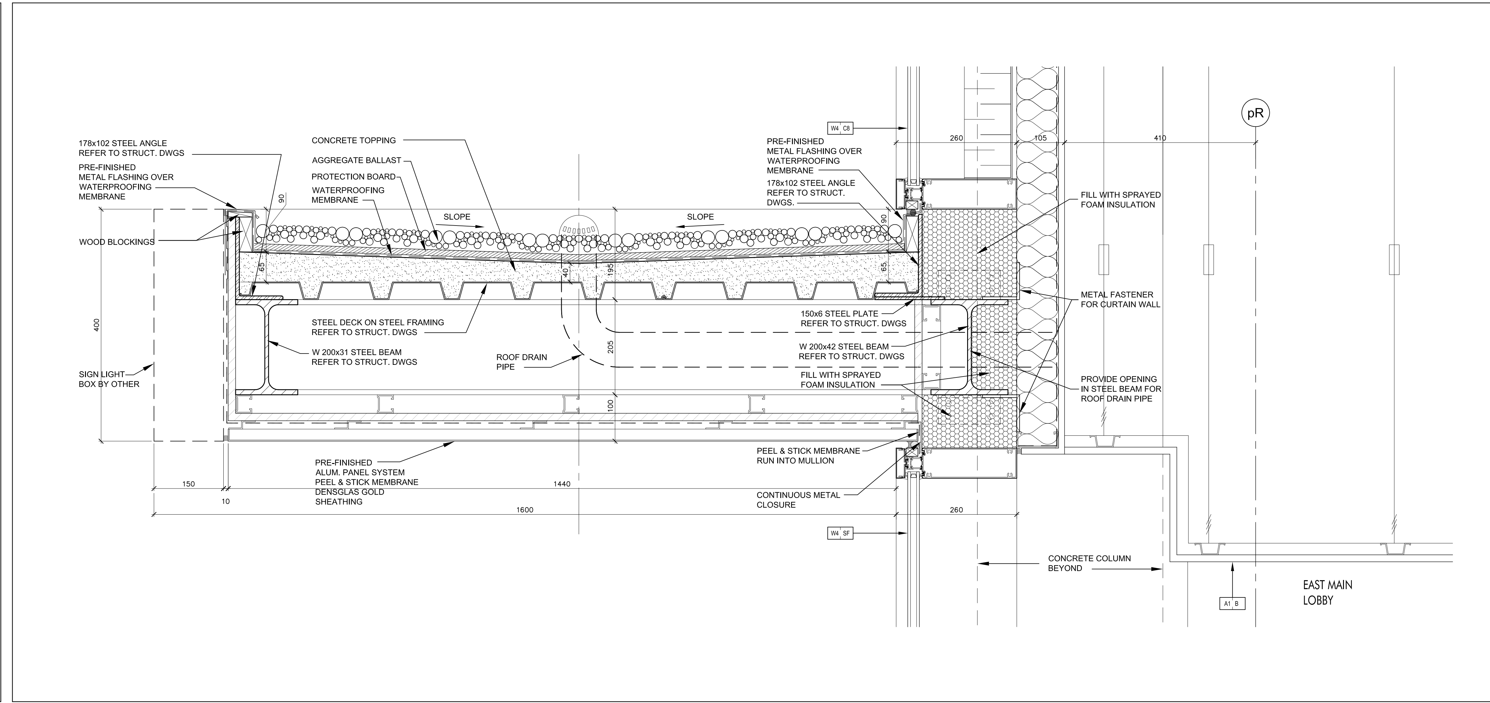
Pre-Finished Aluminum Canopy @ East Main Lobby @ Level 1 SCALE 1:5 A7-16
