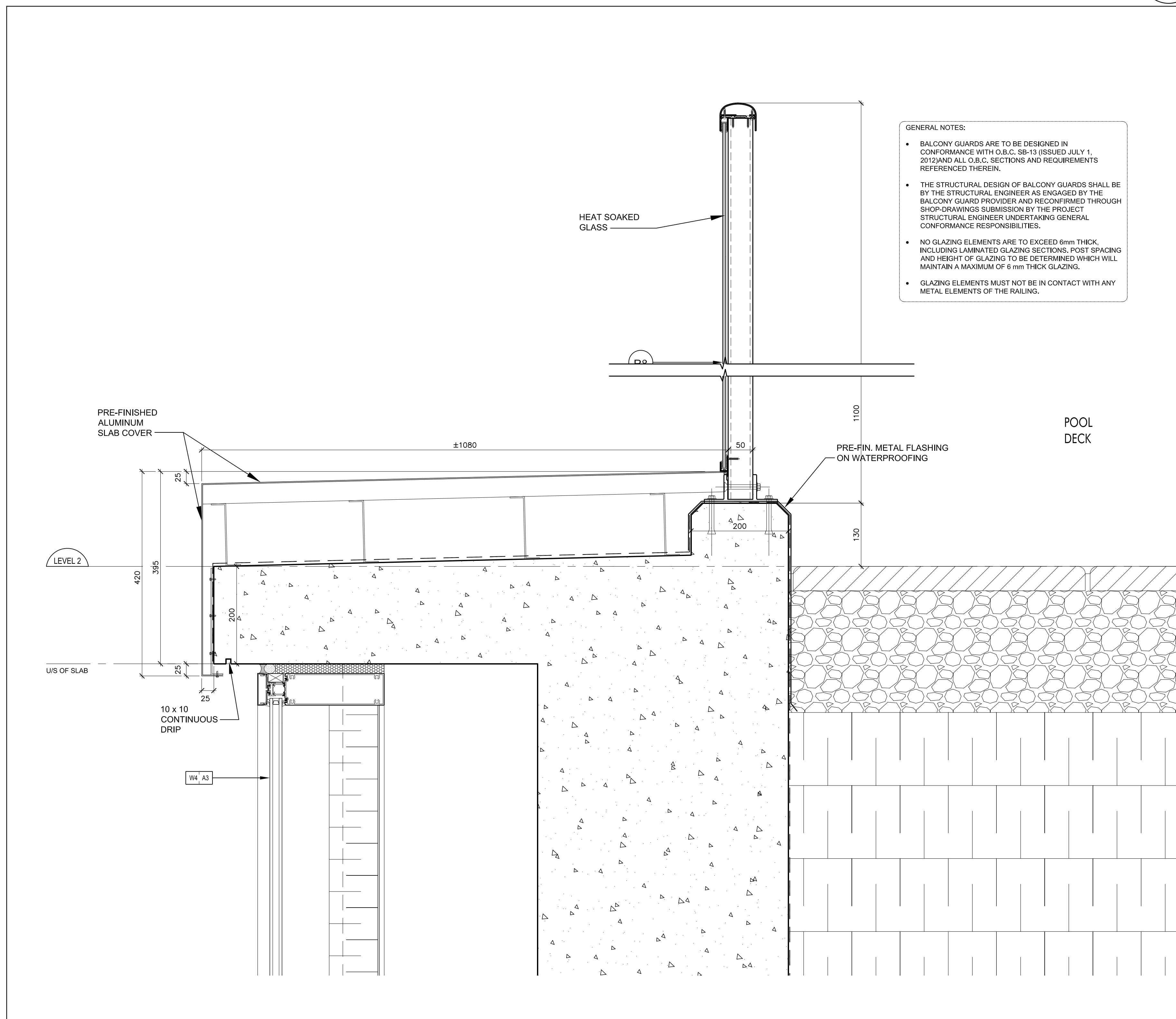
Slab Cover Detail @ Pool Deck @ Level 2 (Ref. Wall Section 6/A7-04) SCALE: 1:5
