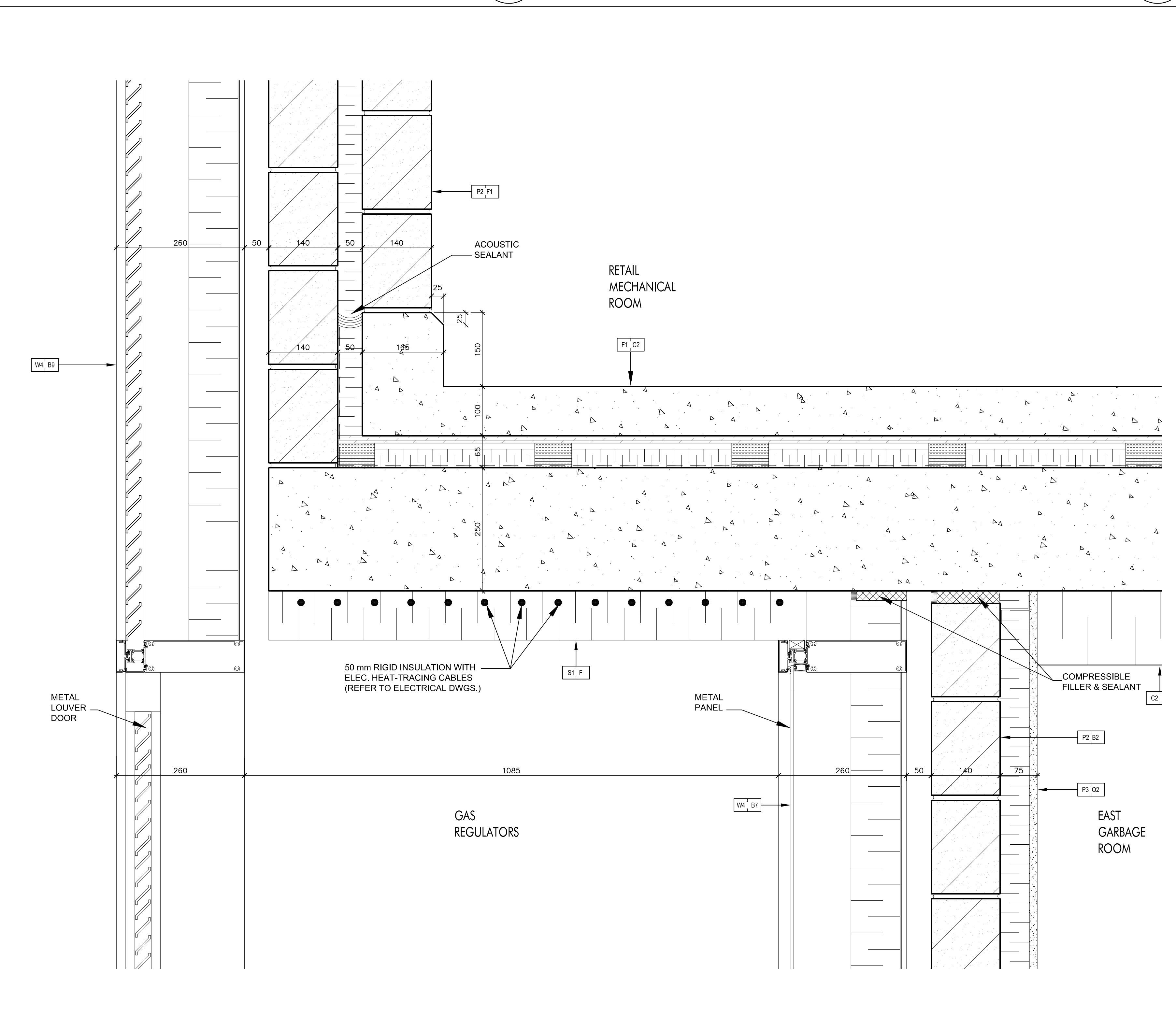
Wall Detail @ Gas Regulators Alcove @ Level 1 (Ref. Wall Section 6/A7-02) SCALE: 1:5
