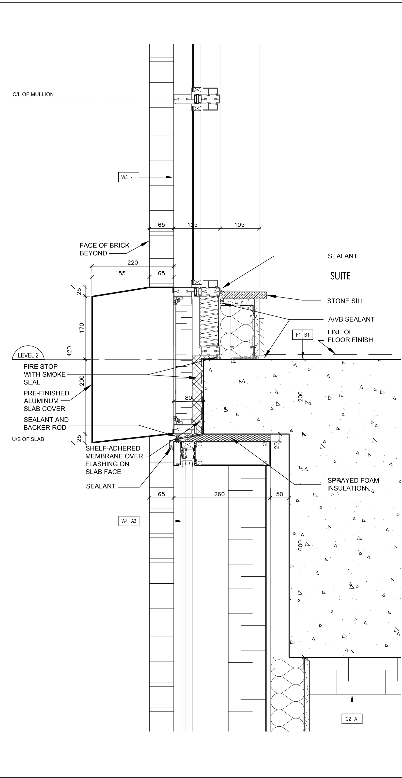
Pre-Fin. Alum. Slab Cover @ E/ Main Lobby @ L 1 (Ref. Wall Section 7/A7-02) SCALE: 1:5
