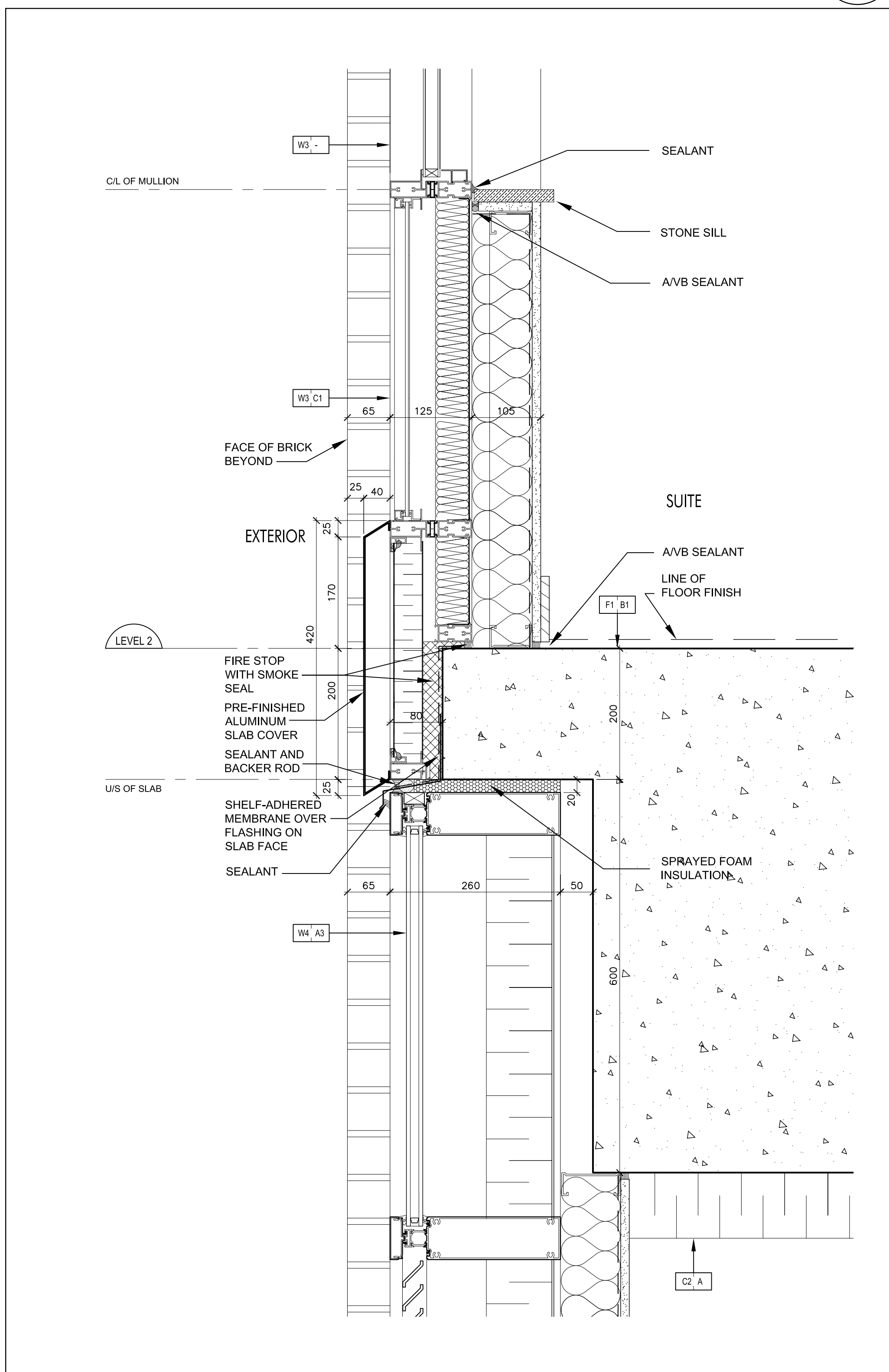
Pre-Finished Aluminum Slab Cover @ Retail @ Level 1 (Ref. Wall Section 4/A7-03) SCALE: 1:5
