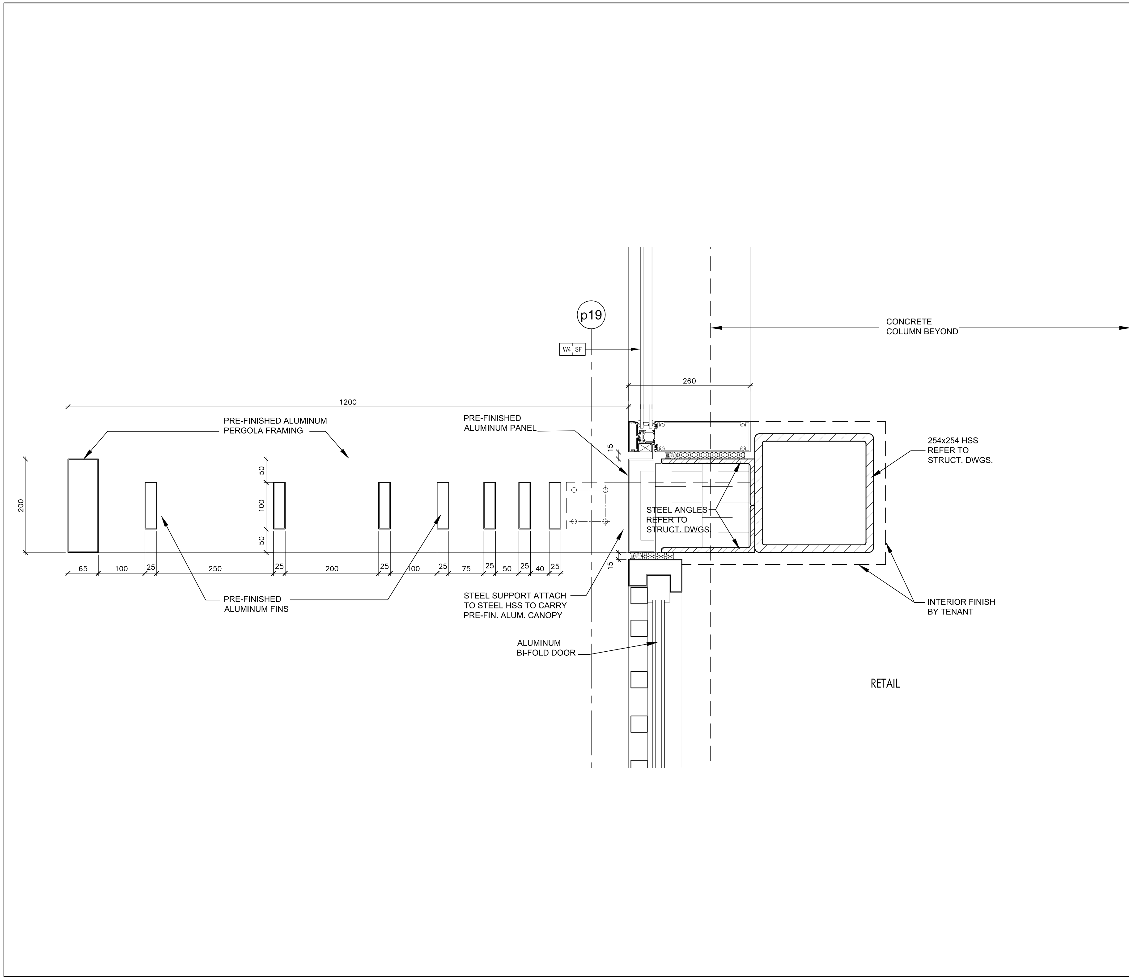
Pre-Finished Aluminum Trellis Canopy @ Retail @ Level 1 (Ref. Wall Section 6/A7-04) SCALE: 1:5
