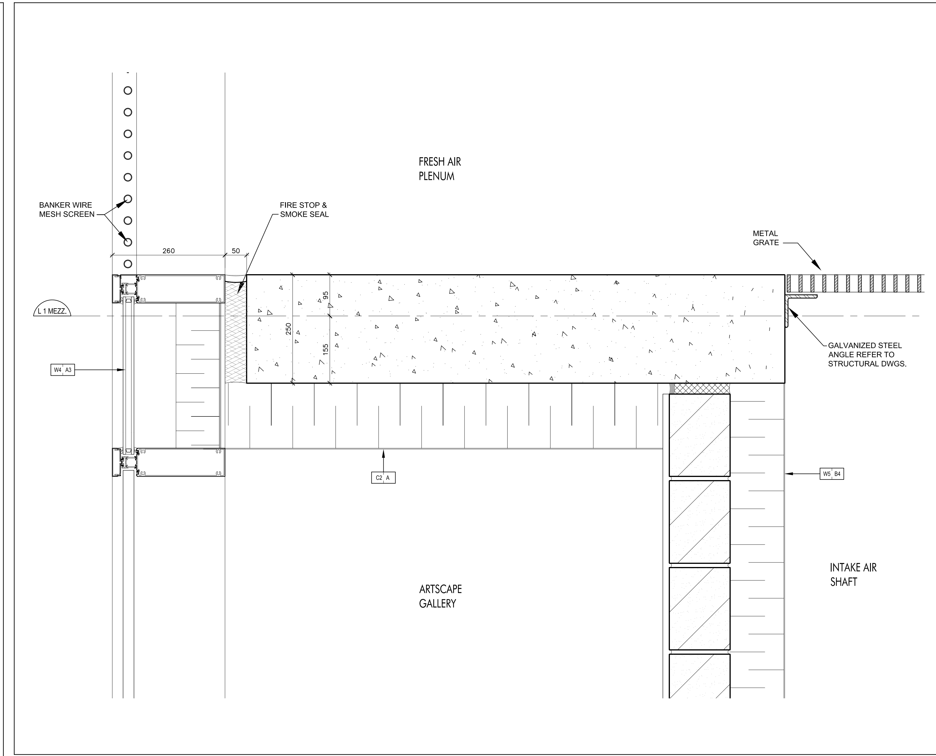
Detail @ Intake Air Shaft @ Level 1 Mezzanine (Ref. Wall Section 9/A7-04) SCALE: 1:5
