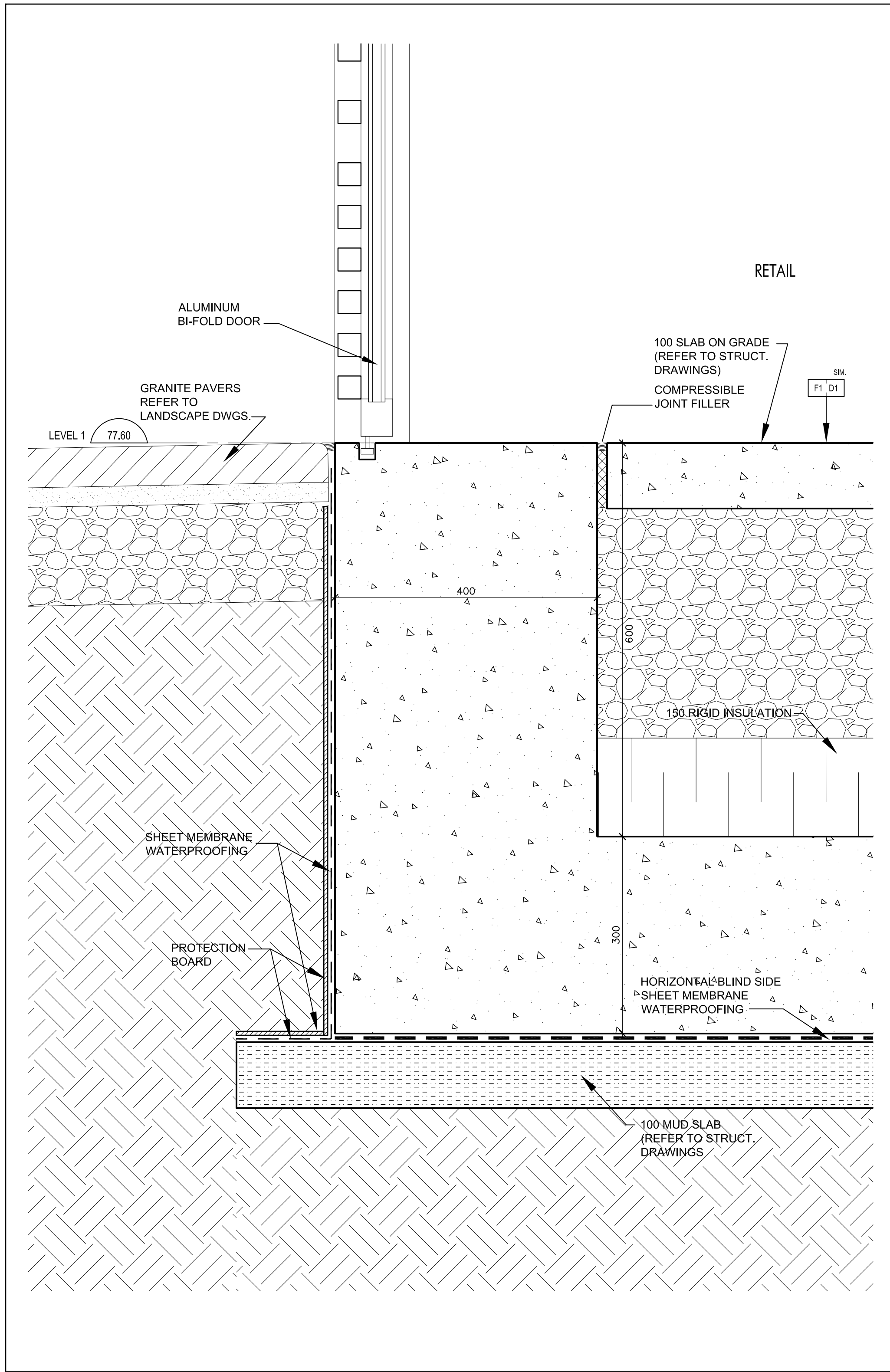
Bi-Fold Door Sill @ Retail @ Level 1 (Ref. Wall Section 6/A7-04) SCALE: 1:5
