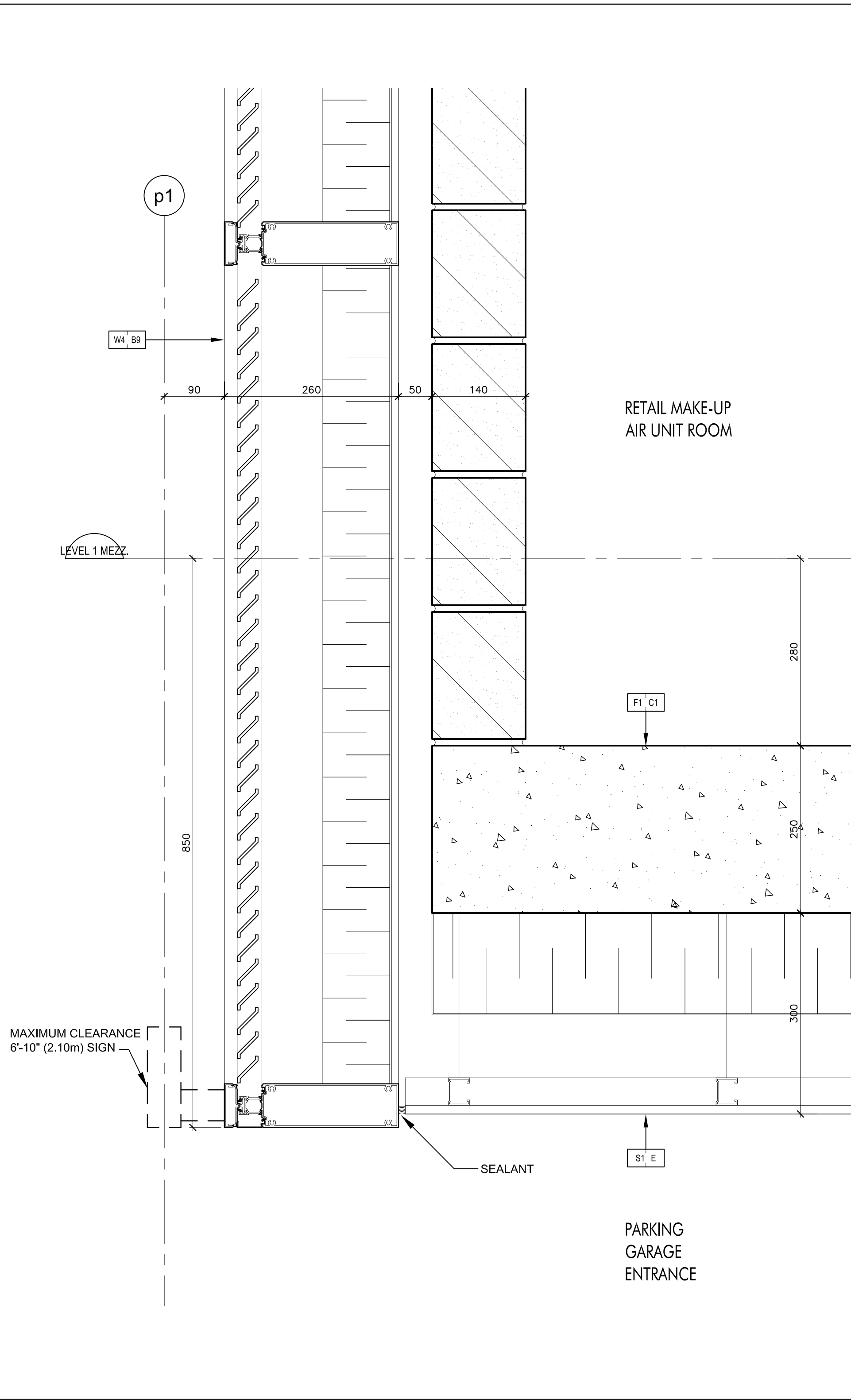
Soffit & Wall Detail @ Parking Garage Entrance @ Level 1 (Ref. Wall Section 5/A7-02) SCALE: 1:5
