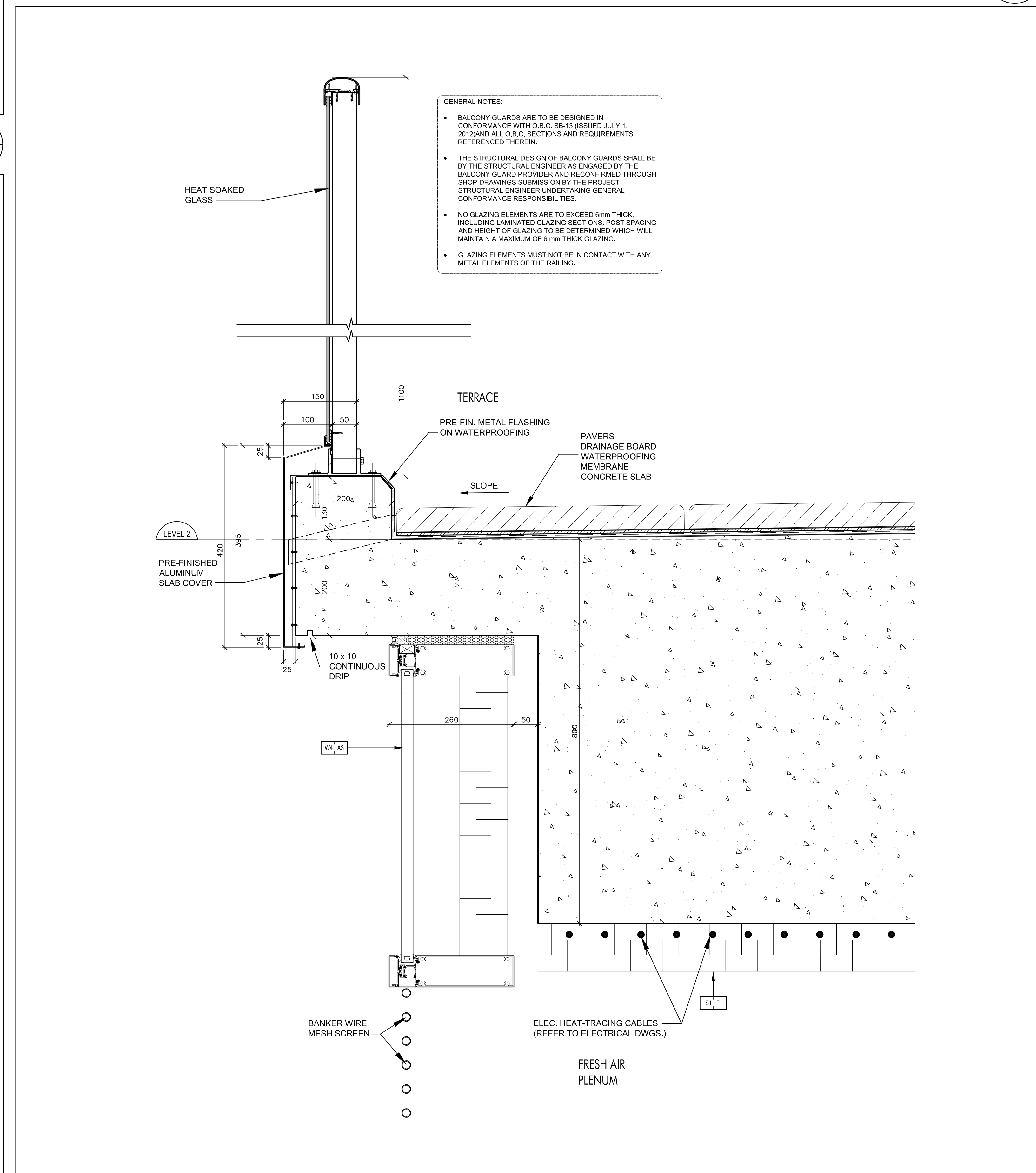
Detail @ Fresh Air Plenum @ Level 2 (Ref. Wall Section 9/A7-04) SCALE: 1:5
