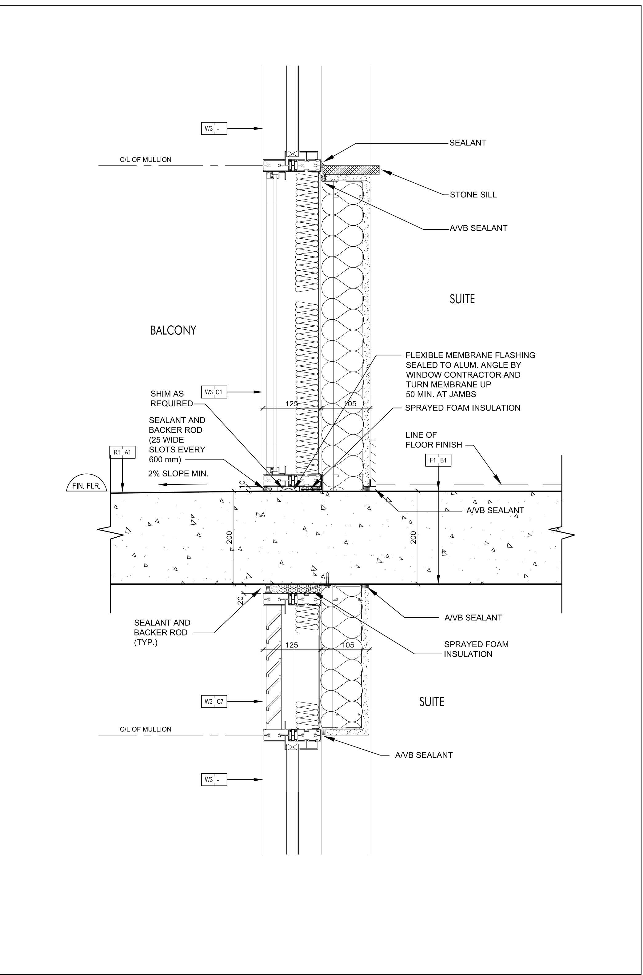
Window Wall @ Balcony SCALE 1:5 A7-11
