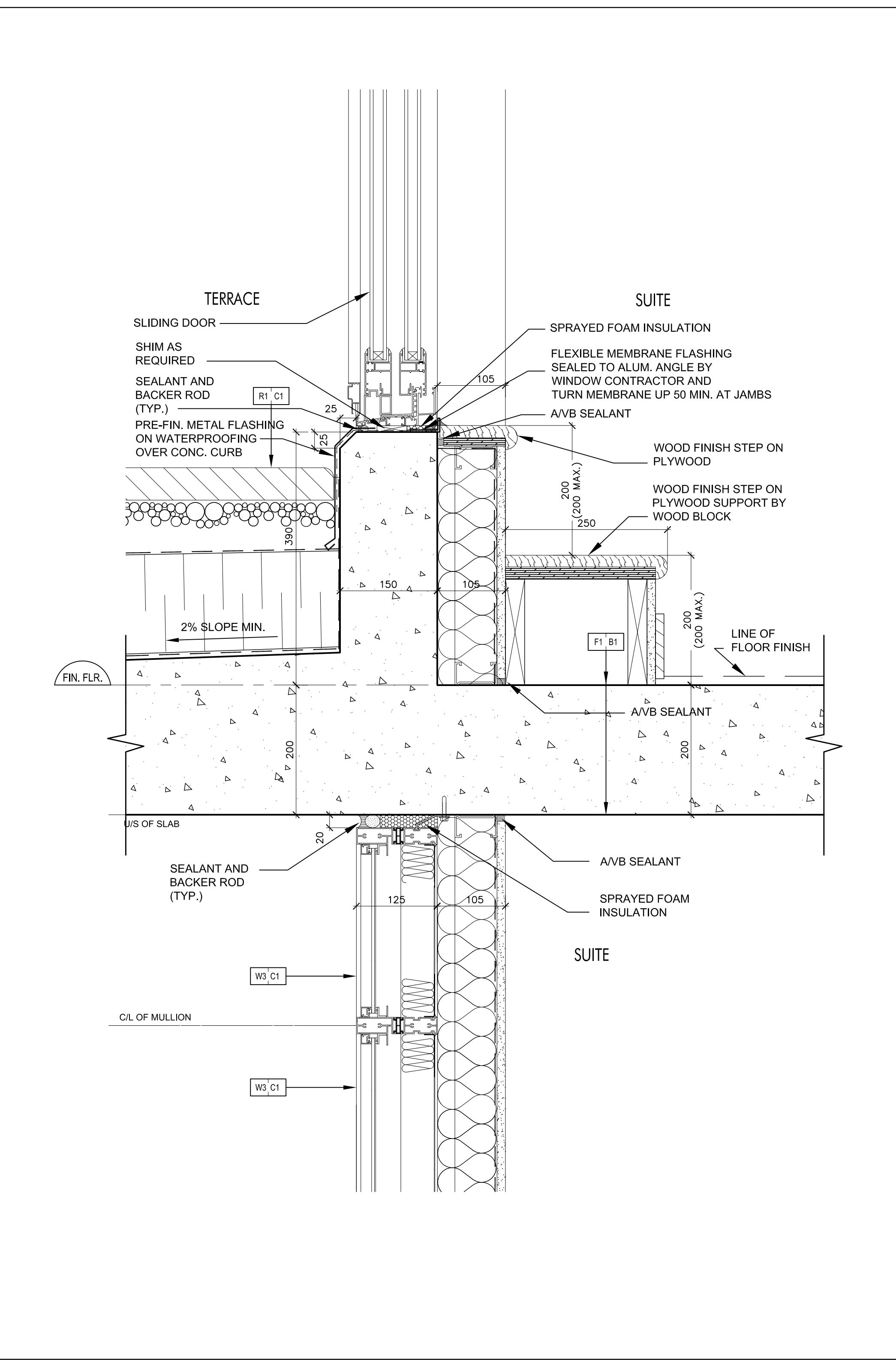
Sliding Door @ Terrace SCALE 1:5 A7-11
