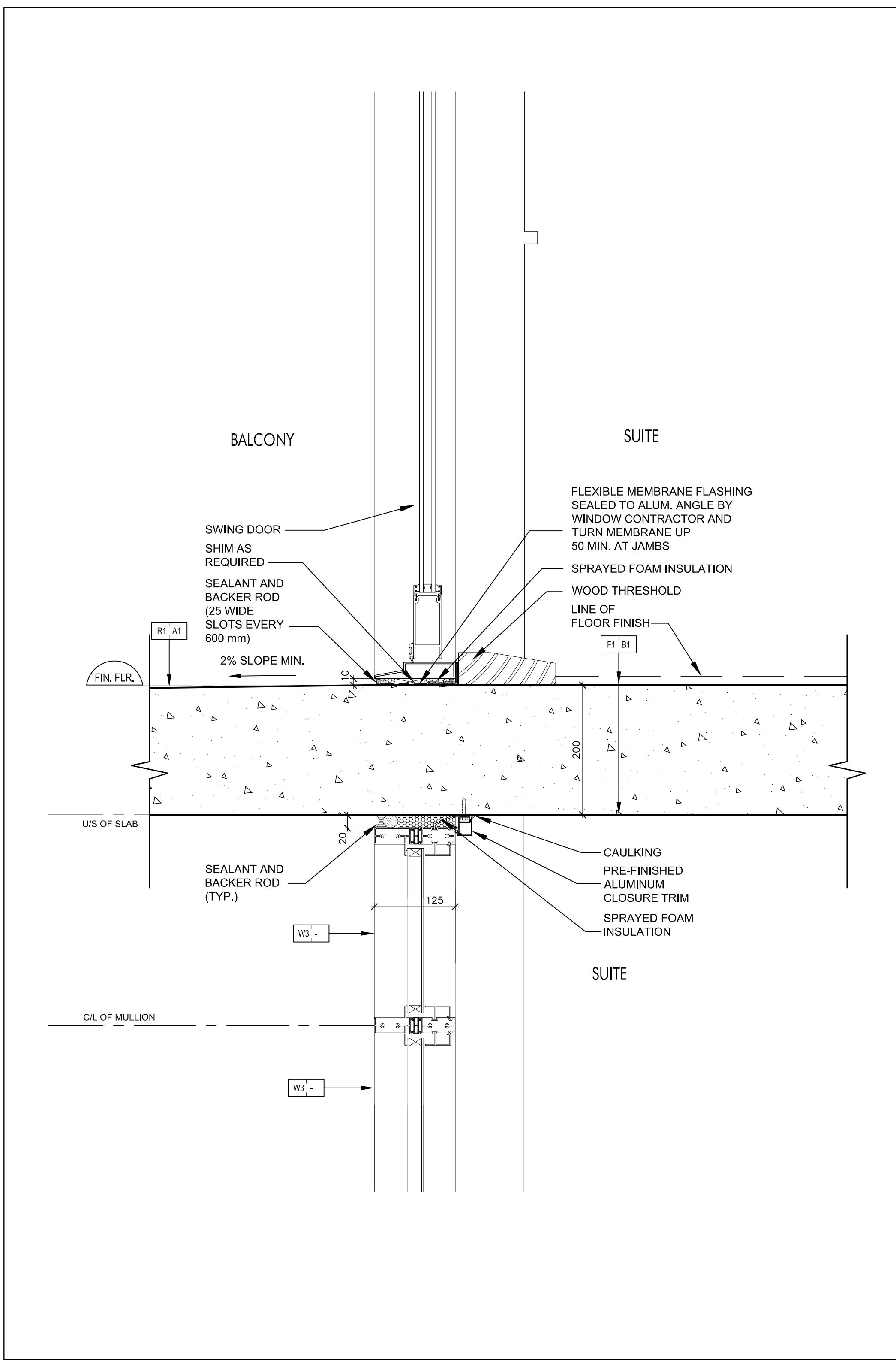
Swing Door @ Balcony SCALE 1:5 A7-11
