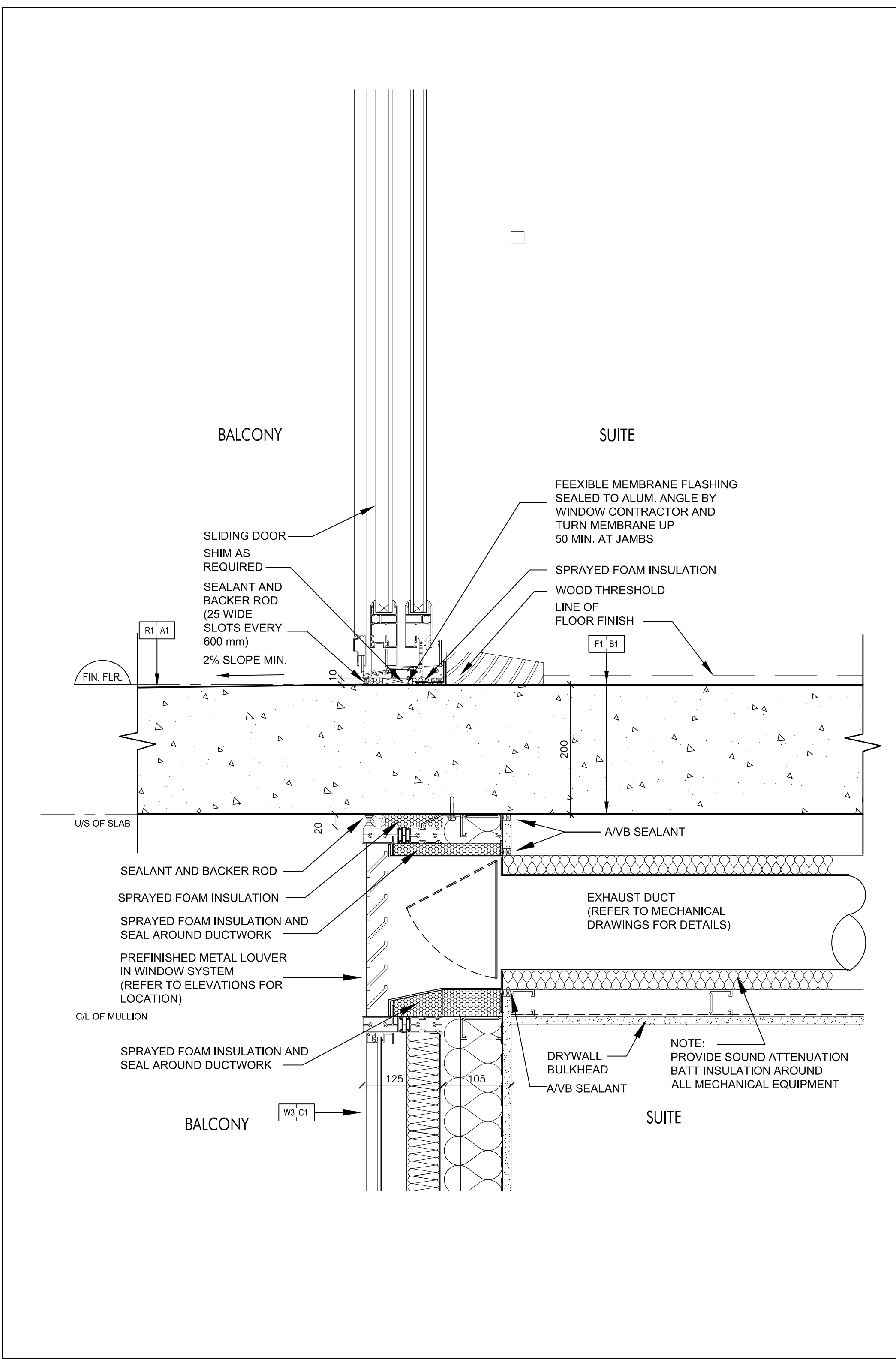
Sliding Door @ Balcony SCALE 1:5 A7-11
