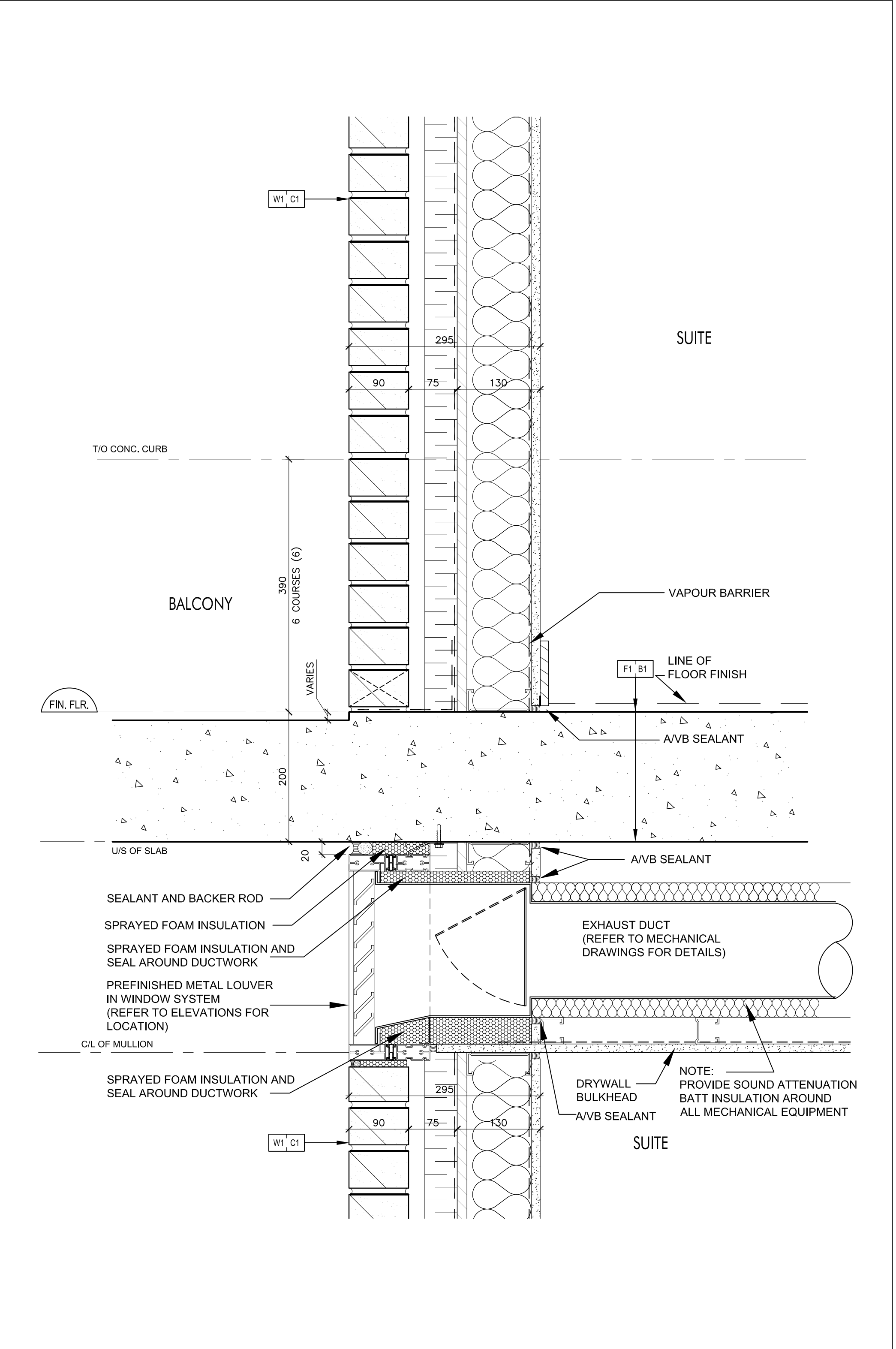
Brick Wall @ Balcony SCALE 1:5 A7-11
