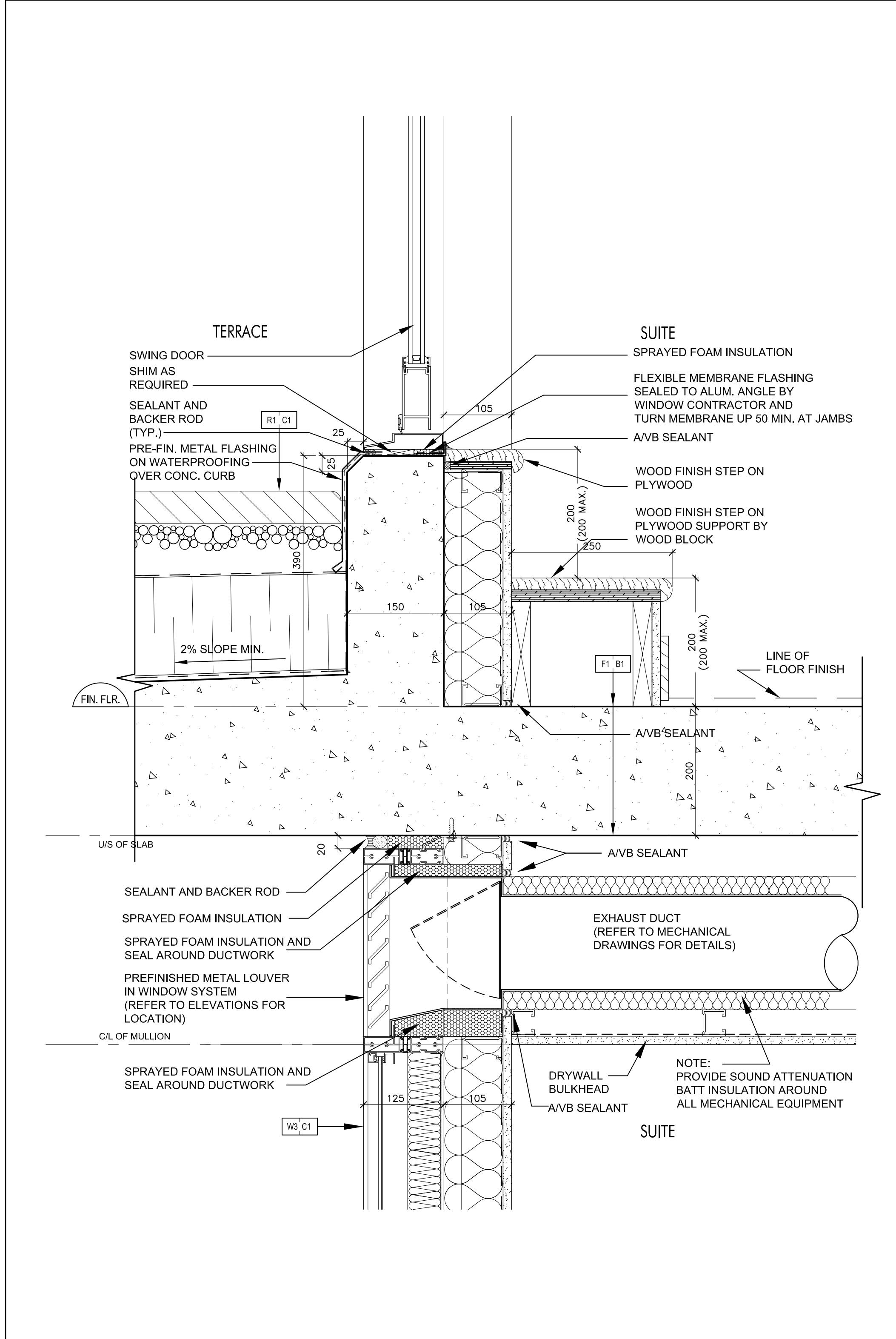
Swing Door @ Terrace SCALE 1:5 A7-11
