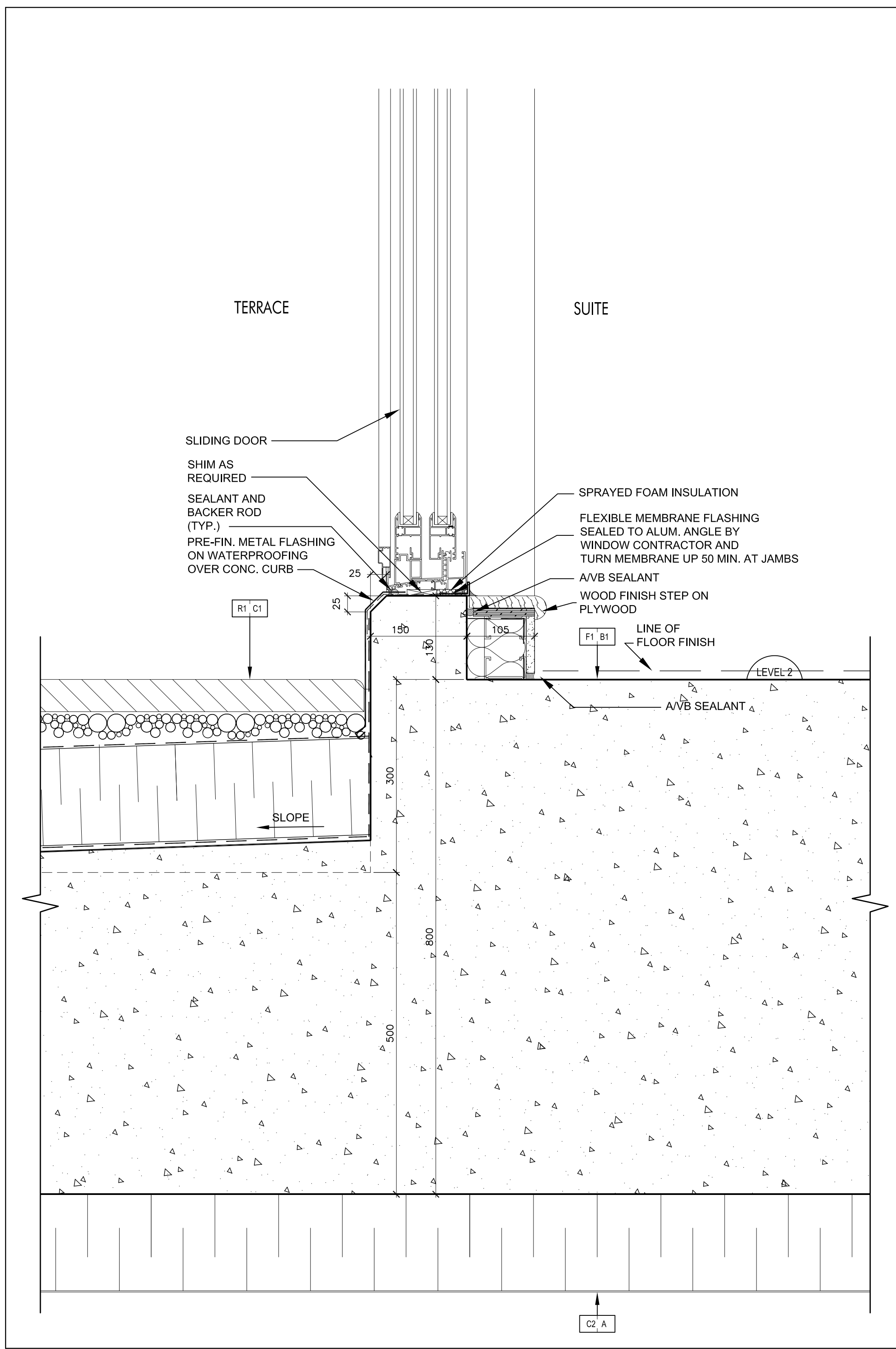
Concrete Curb @ Sliding Door @ Terrace @ Level 2 SCALE 1:5 A7-11
