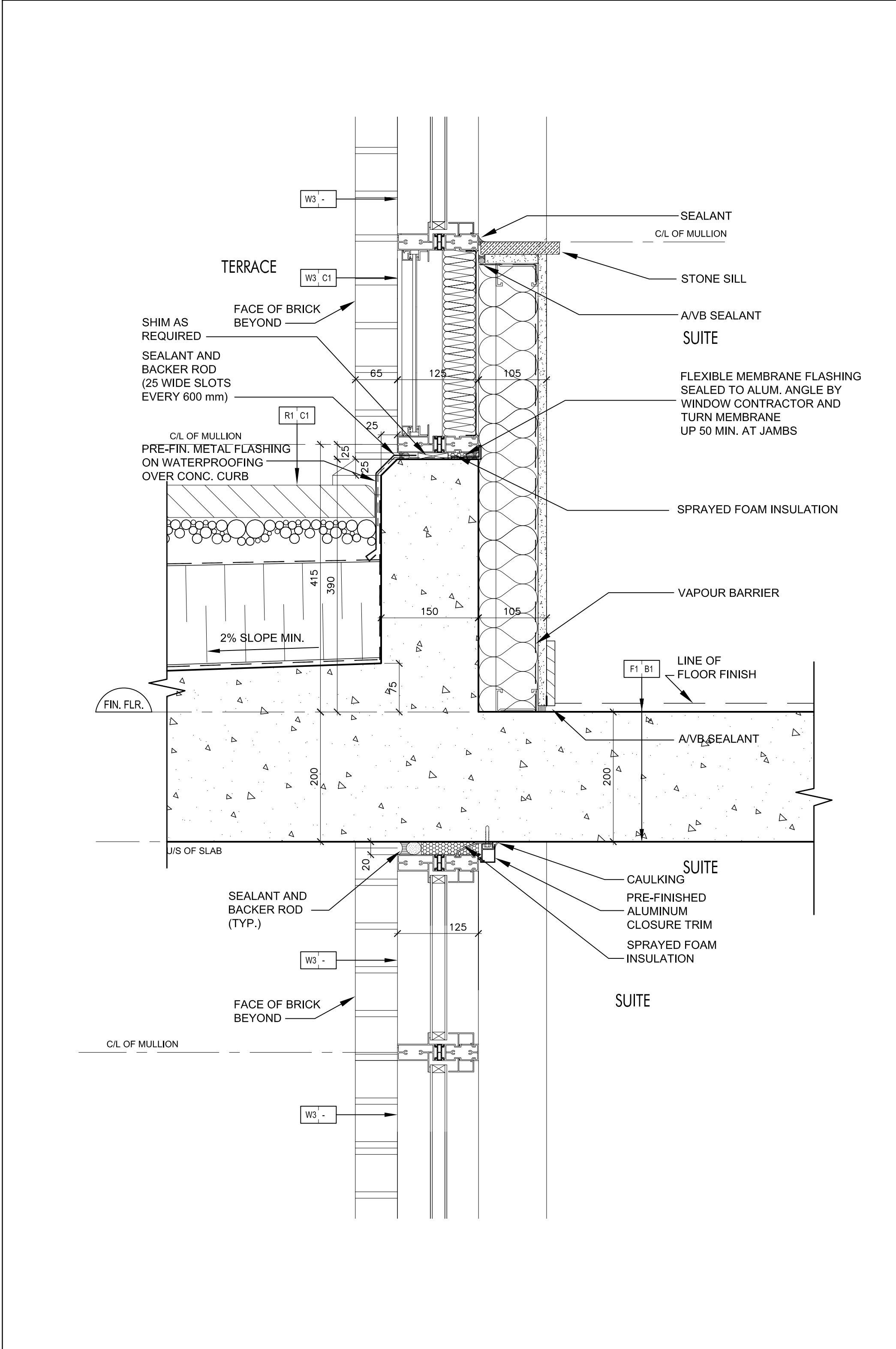
Window Wall @ Terrace SCALE 1:5 A7-11
