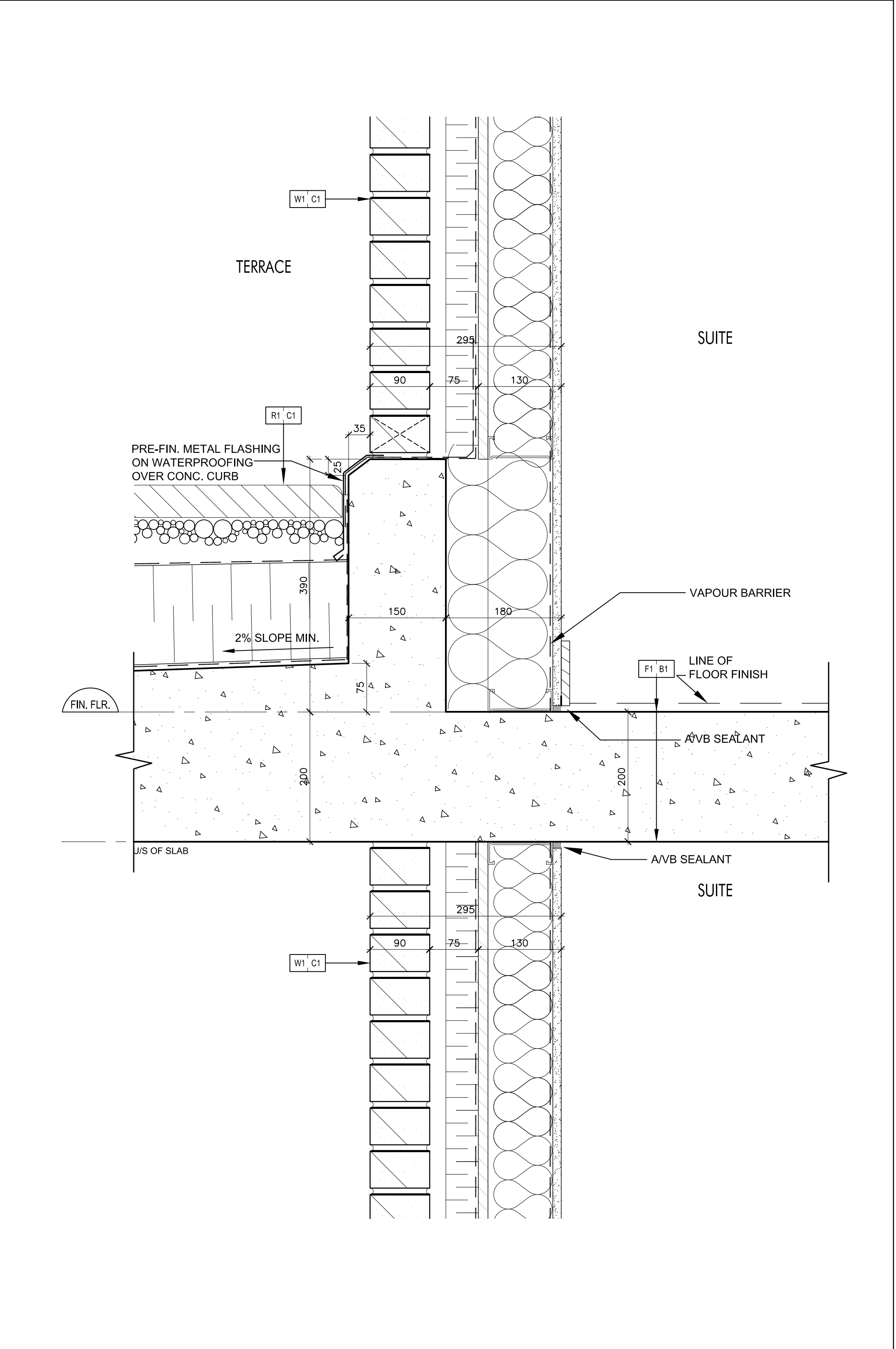
Brick Wall @ Terrace SCALE 1:5 A7-11
