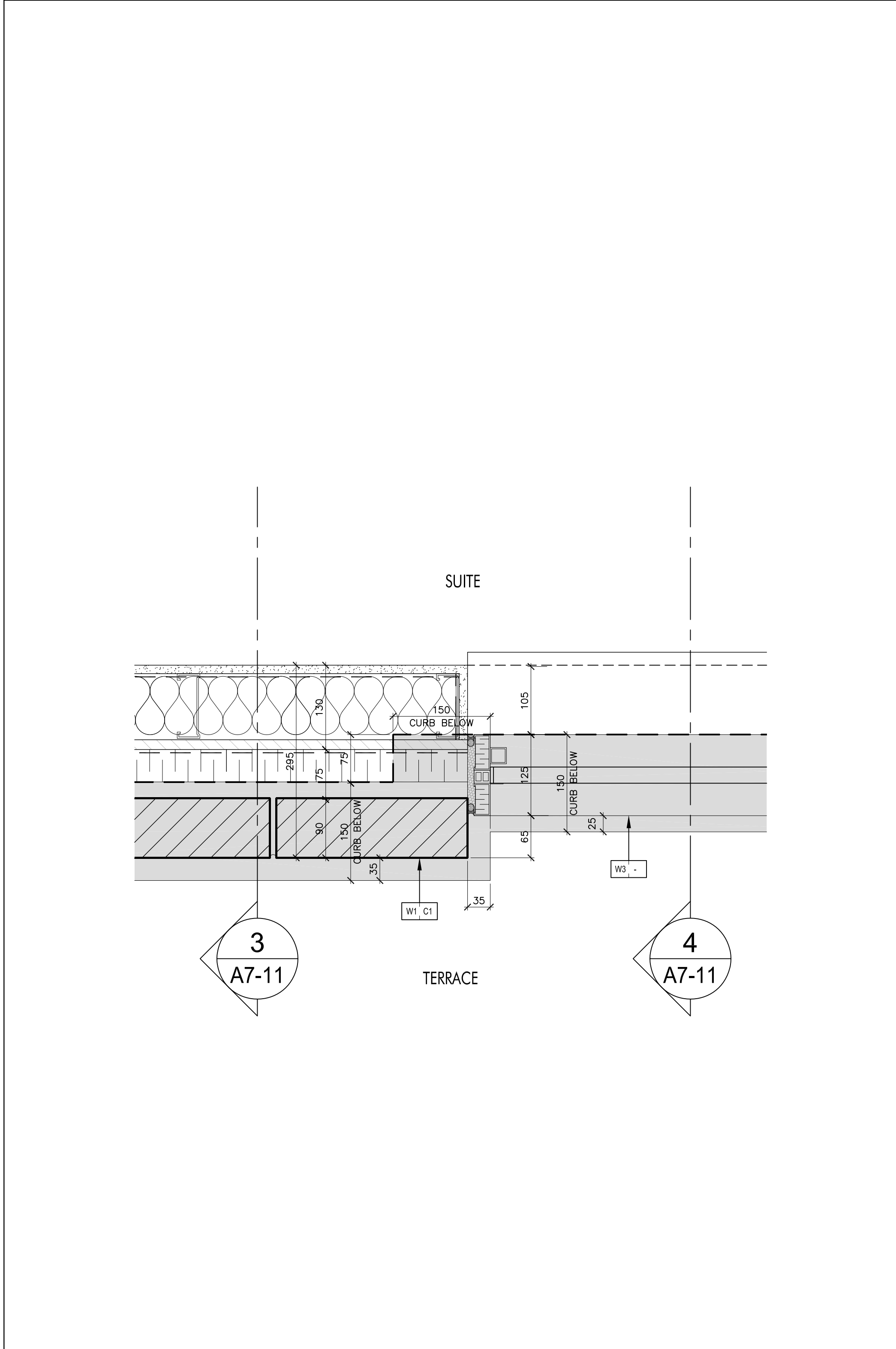
Plan Detail of Window Wall & Brick Wall @ Terrace SCALE 1:5 A7-11
