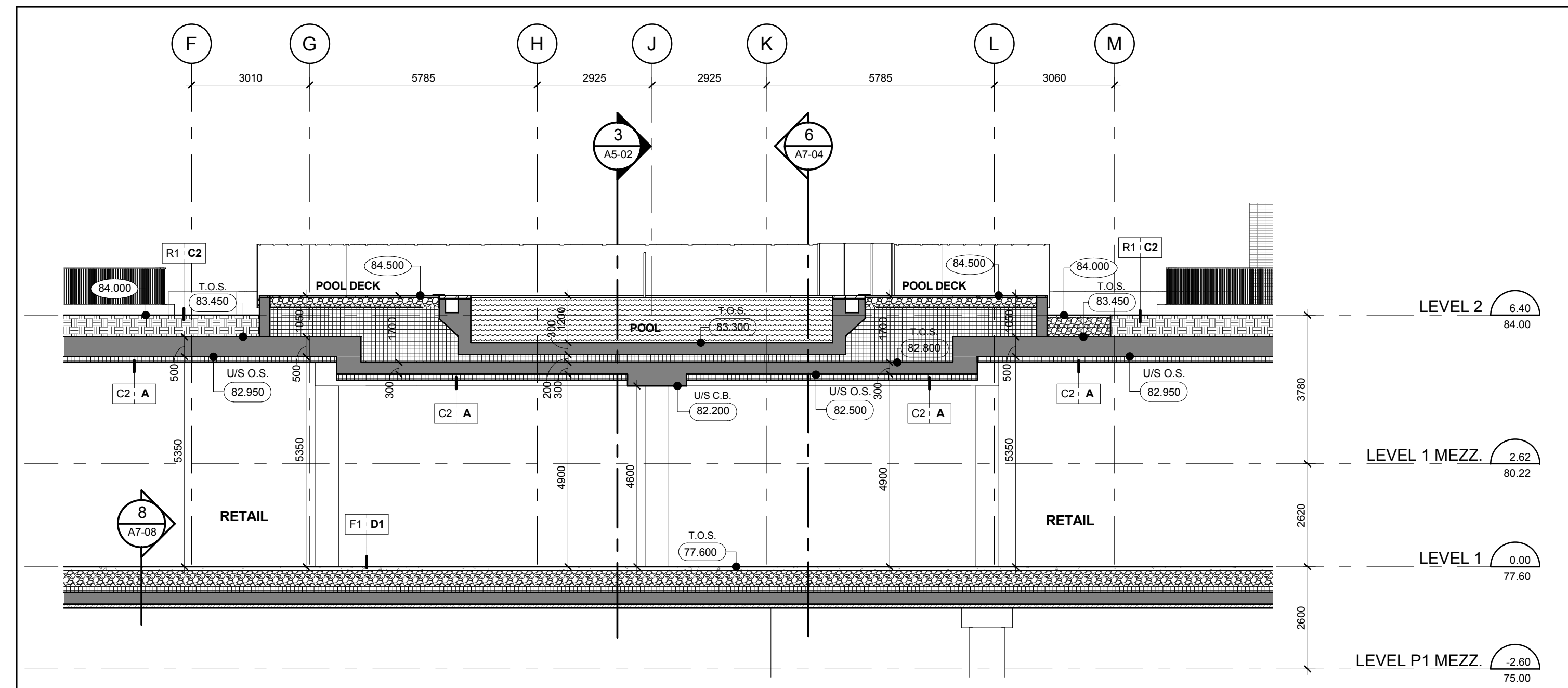
East - West Pool Section Along Gridline p17 4 A5-02 Scale: 1 : 100
