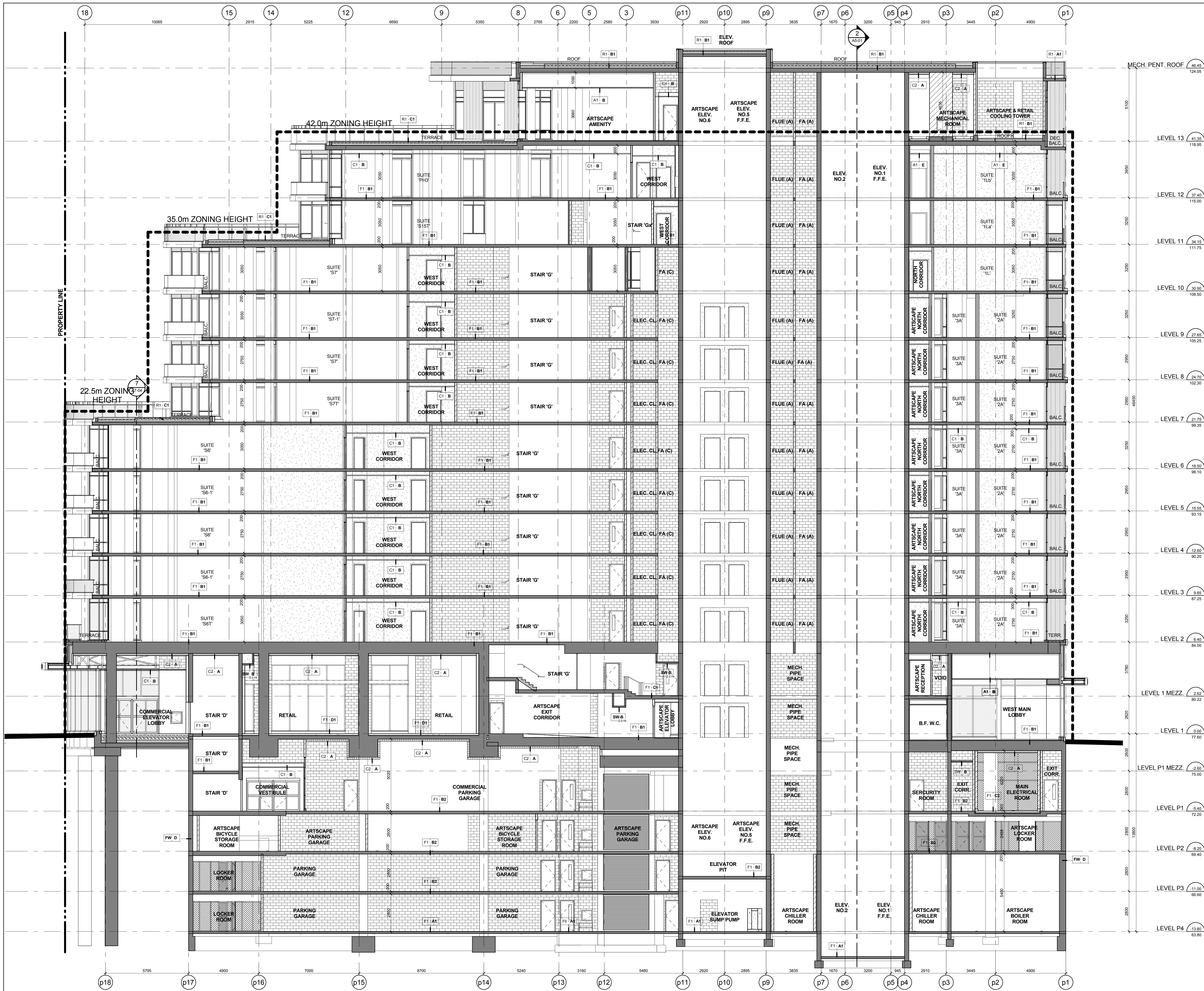
North - South Building Section Along Gridline pD 1 A5-01 Scale: 1 : 100
