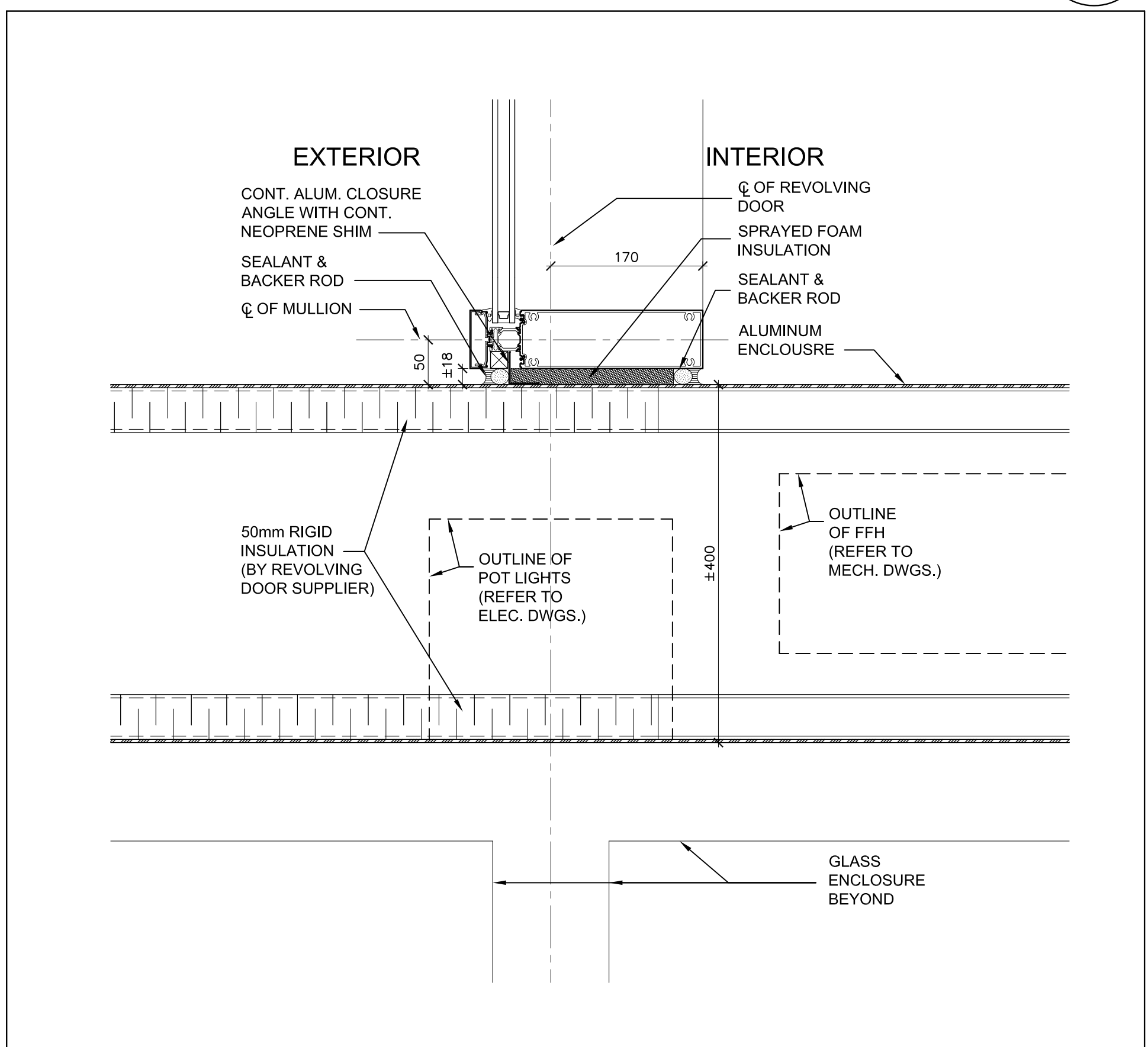
Section Detail @ Revolving Door Roof 4 SCALE 1:5 A7-18
