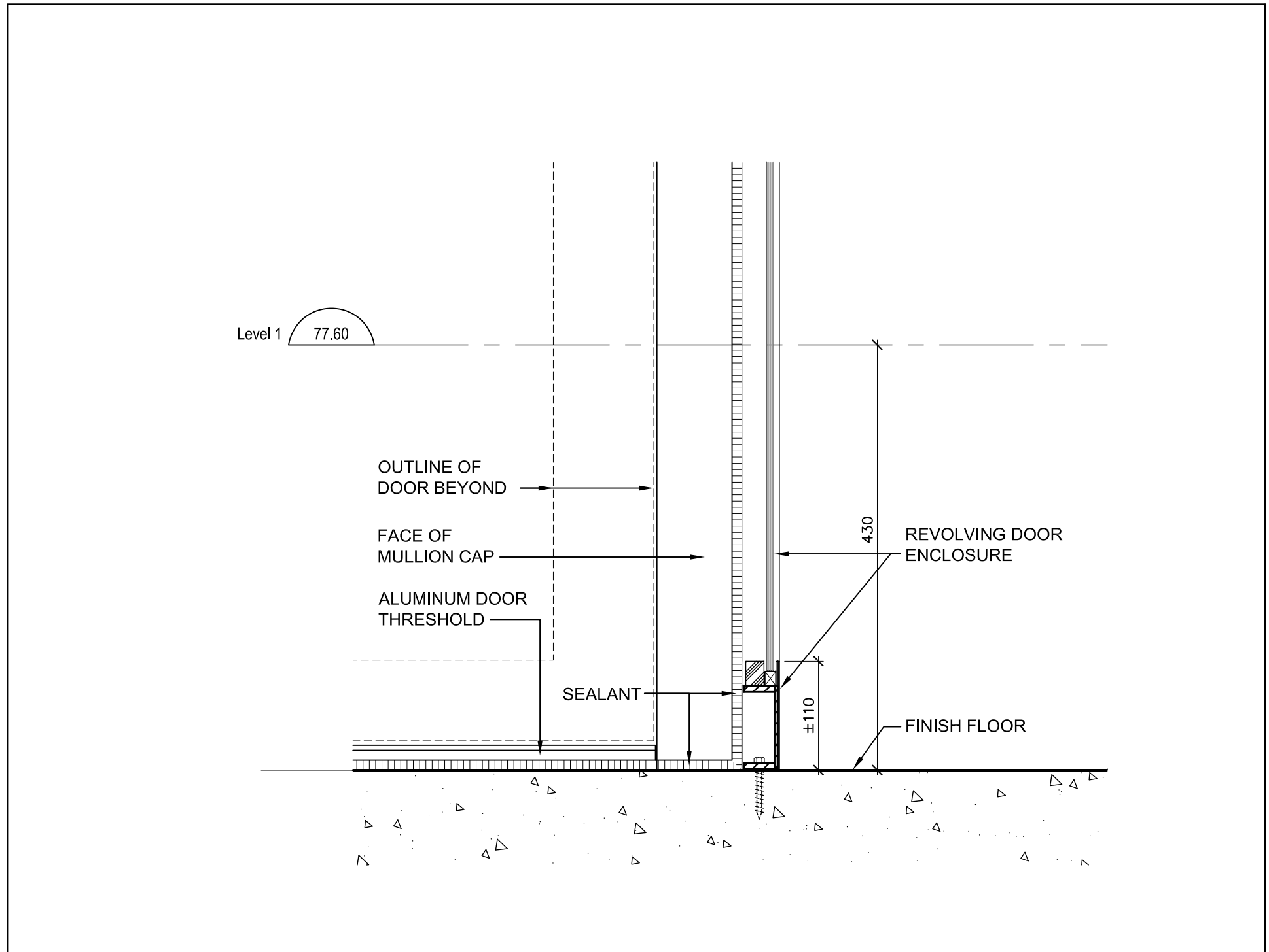
Section Detail @ Revolving Door Enclosure 5 SCALE 1:5 A7-18
