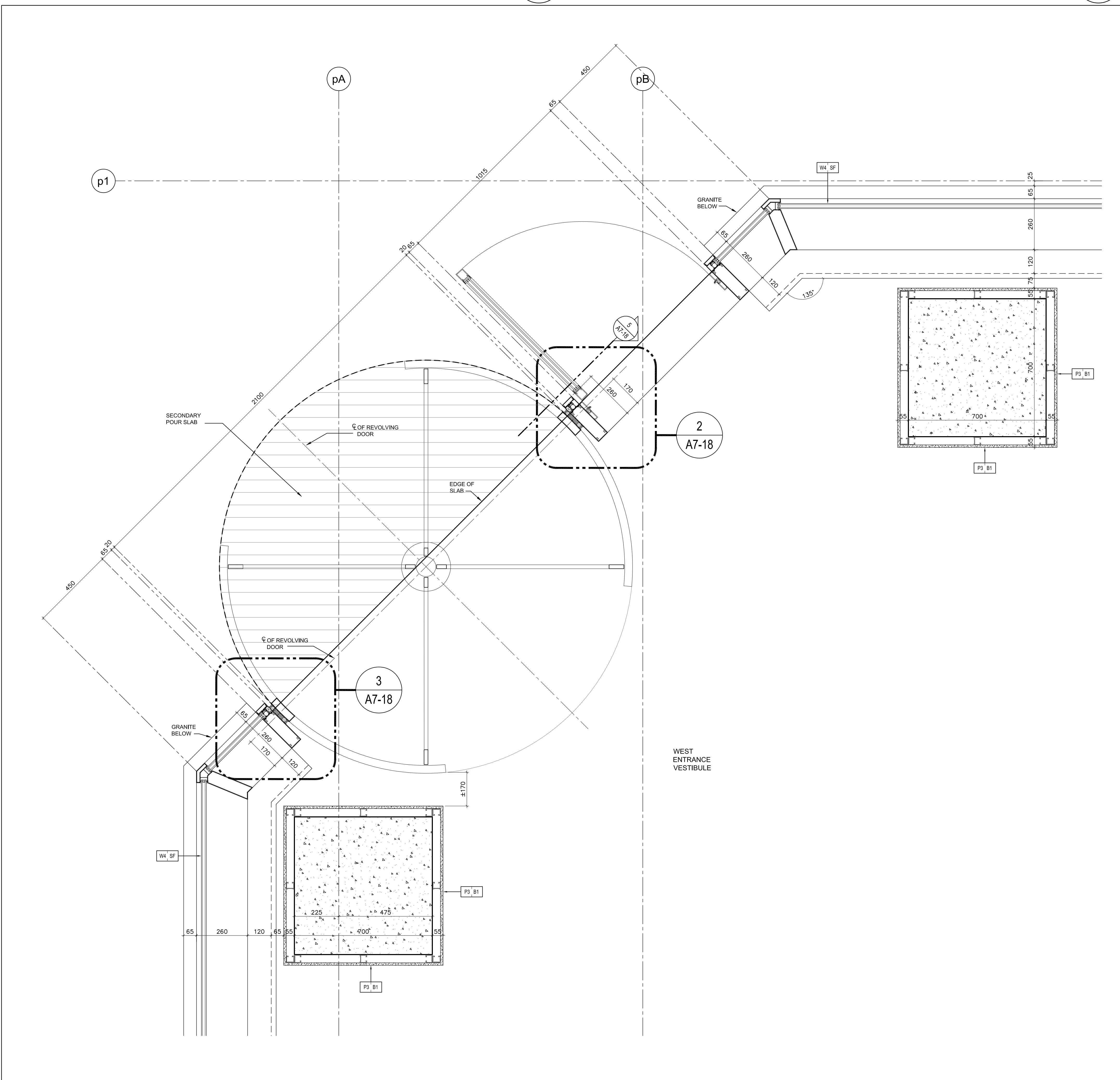
Plan Detail @ Revolving Door @ West Entrance Vestibule @ Level 1 SCALE 1:10 A7-18
