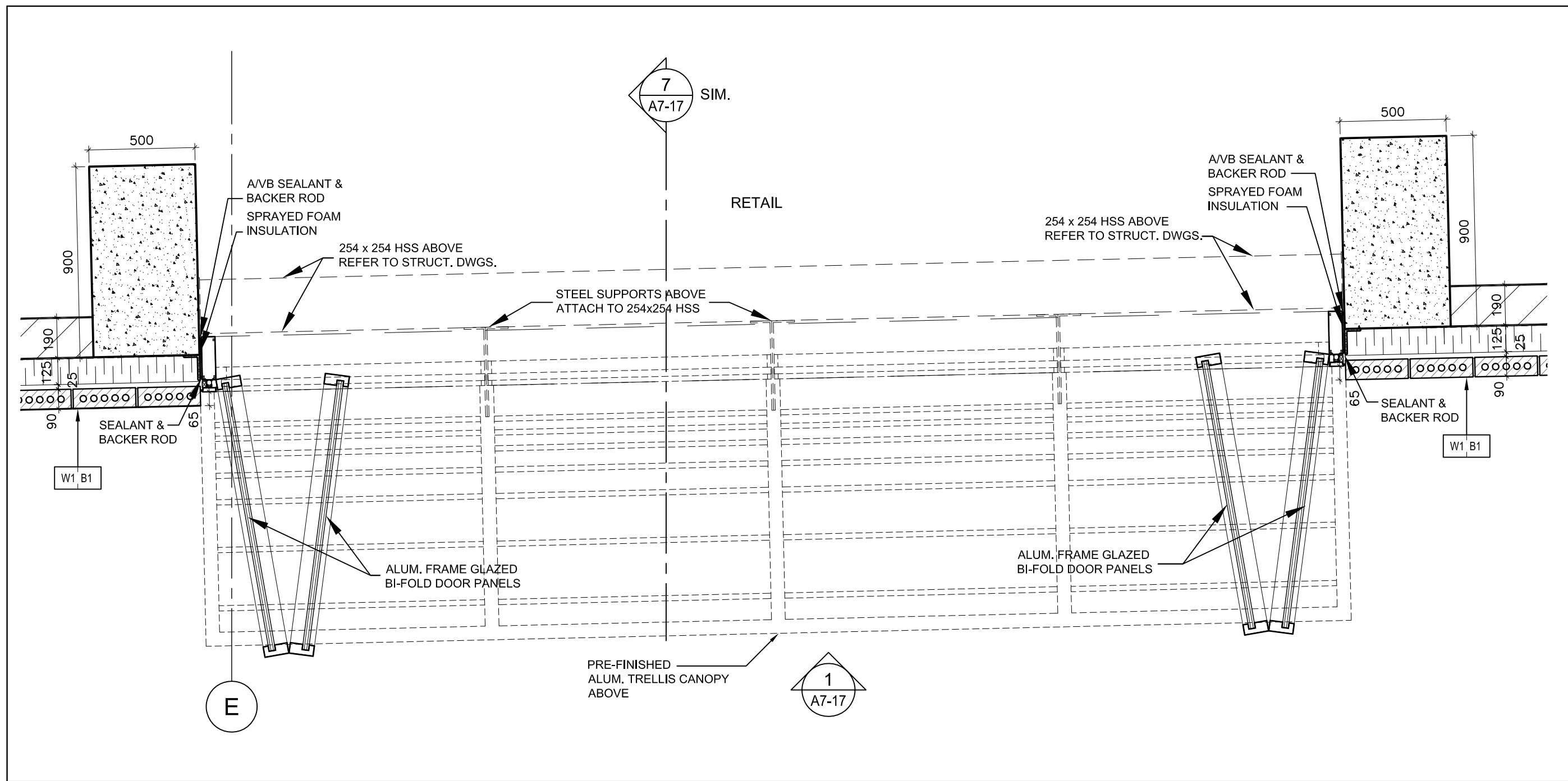
Plan - Bi-Fold Door 1 @ Retail @ Level 1 2 A7-17 SCALE 1:20
