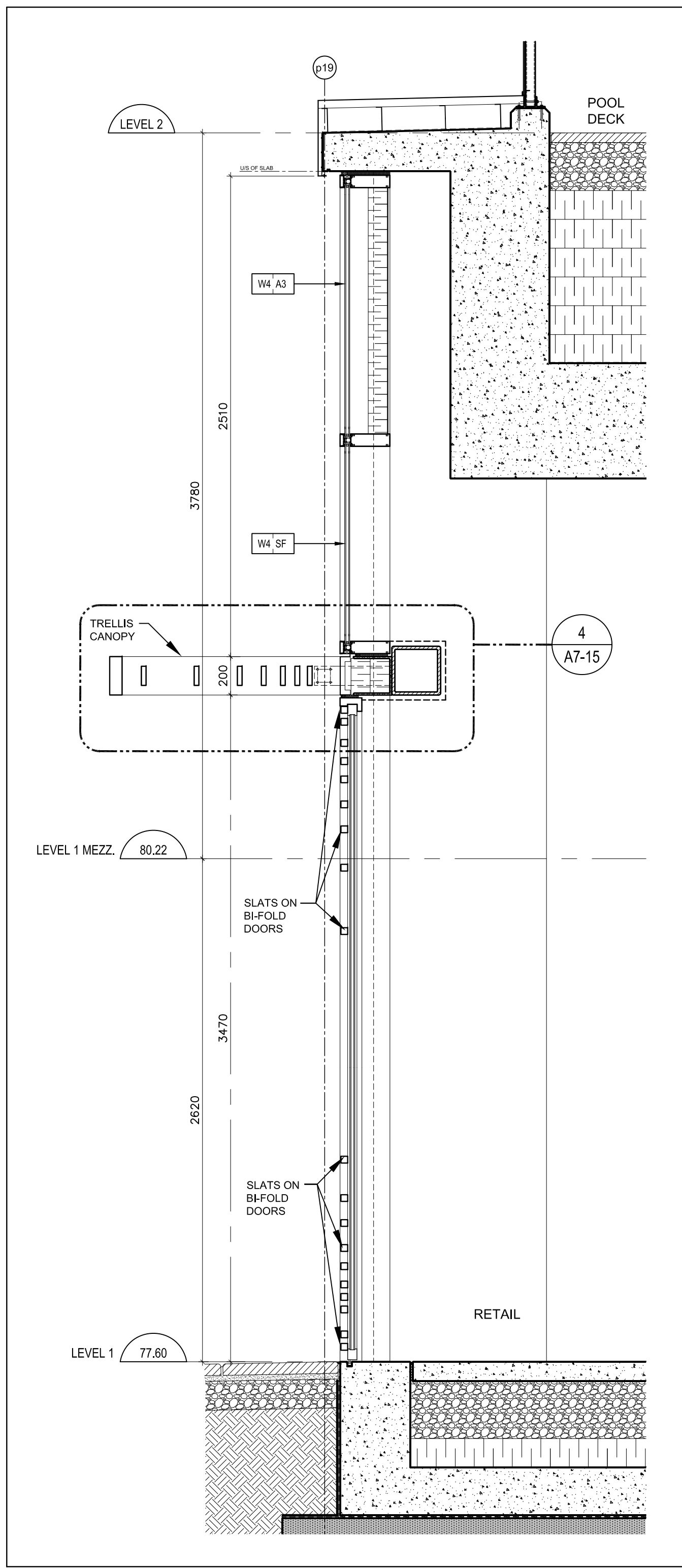
Section thru Bi-Fold Door @ Retail @ Level 1 7 A7-17 SCALE 1:20
