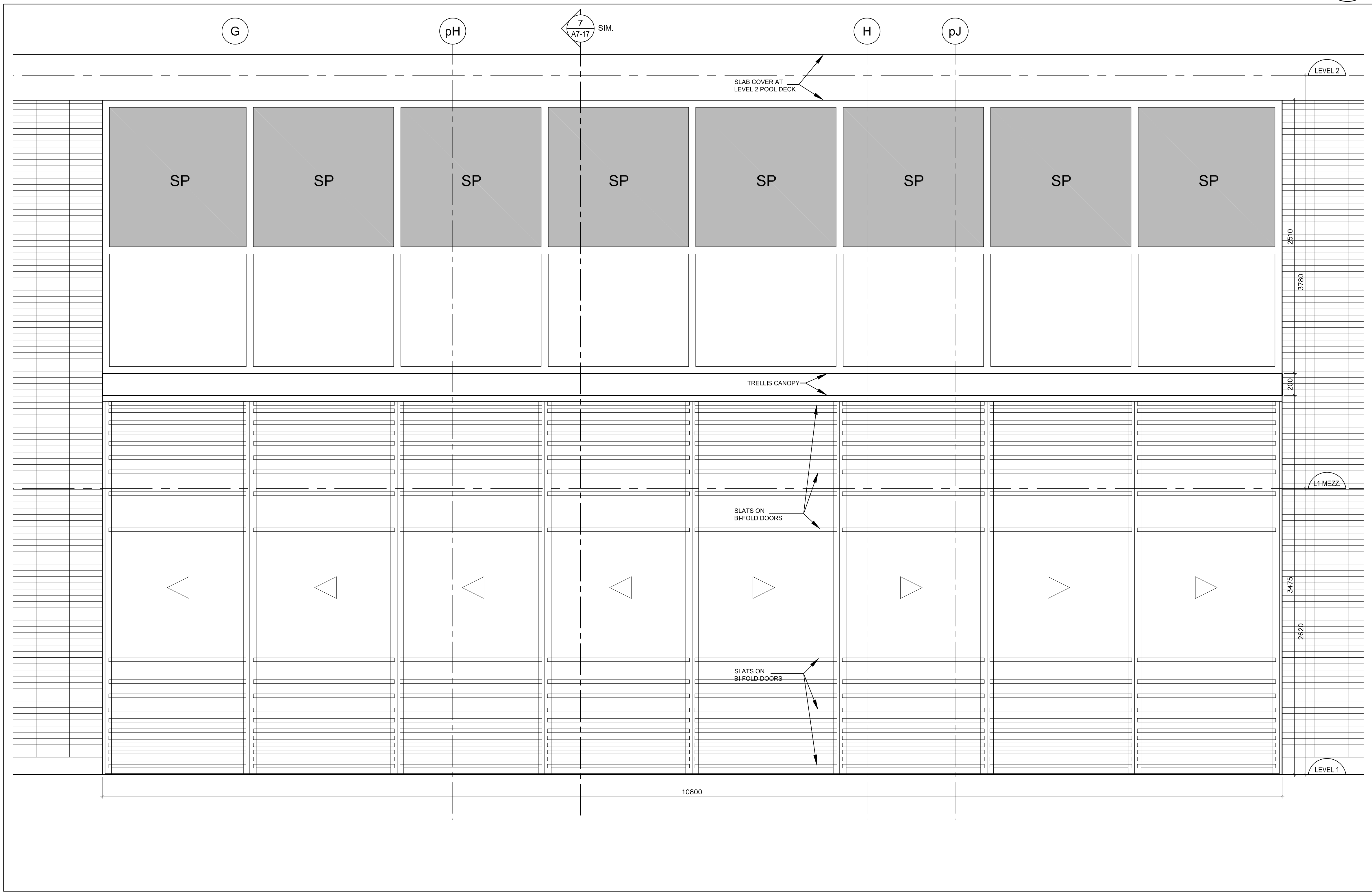
Elevation - Bi-Fold Door 2 @ Retail @ Level 1 3 A7-17 SCALE 1:20
