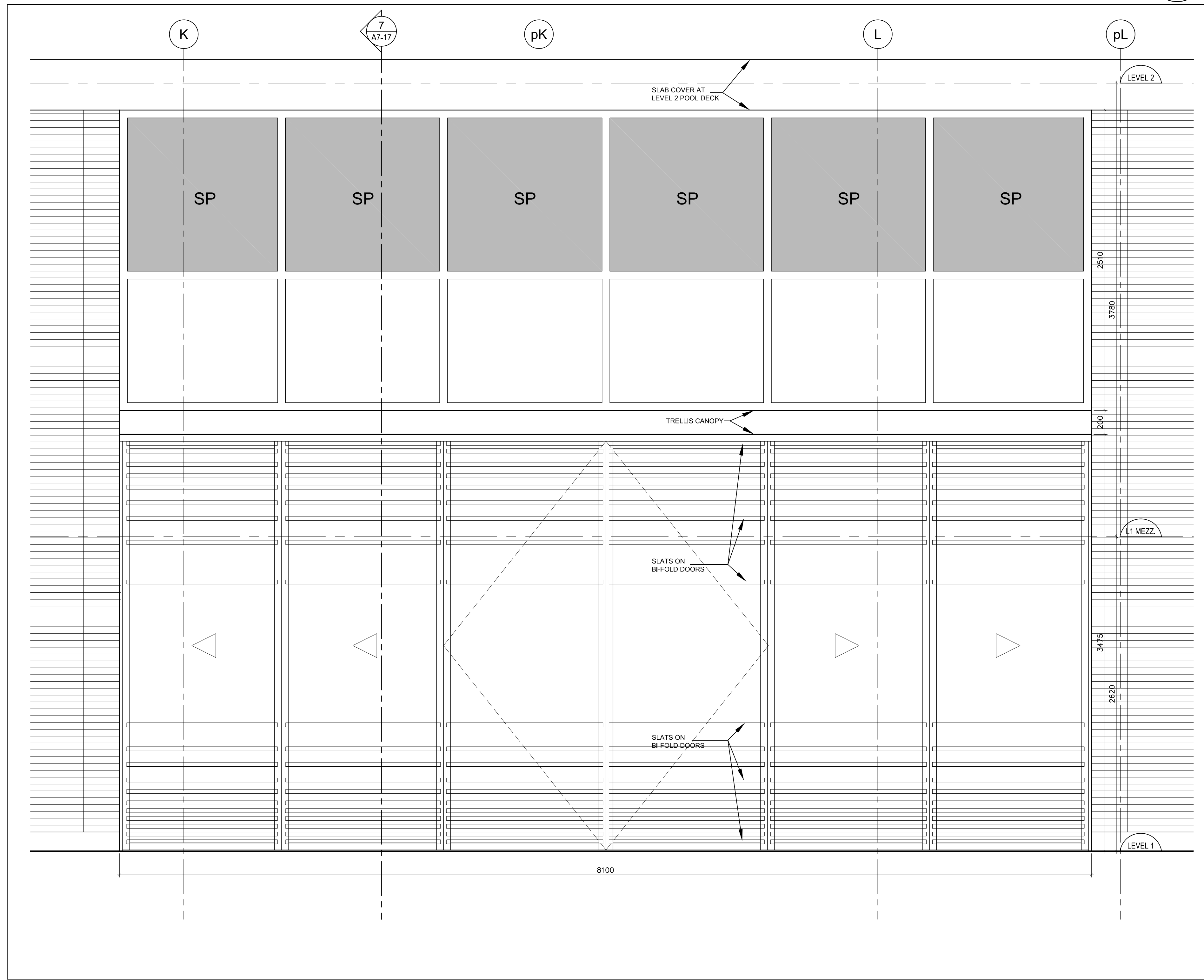
Elevation - Bi-Fold Door 3 @ Retail @ Level 1 5 A7-17 SCALE 1:20
