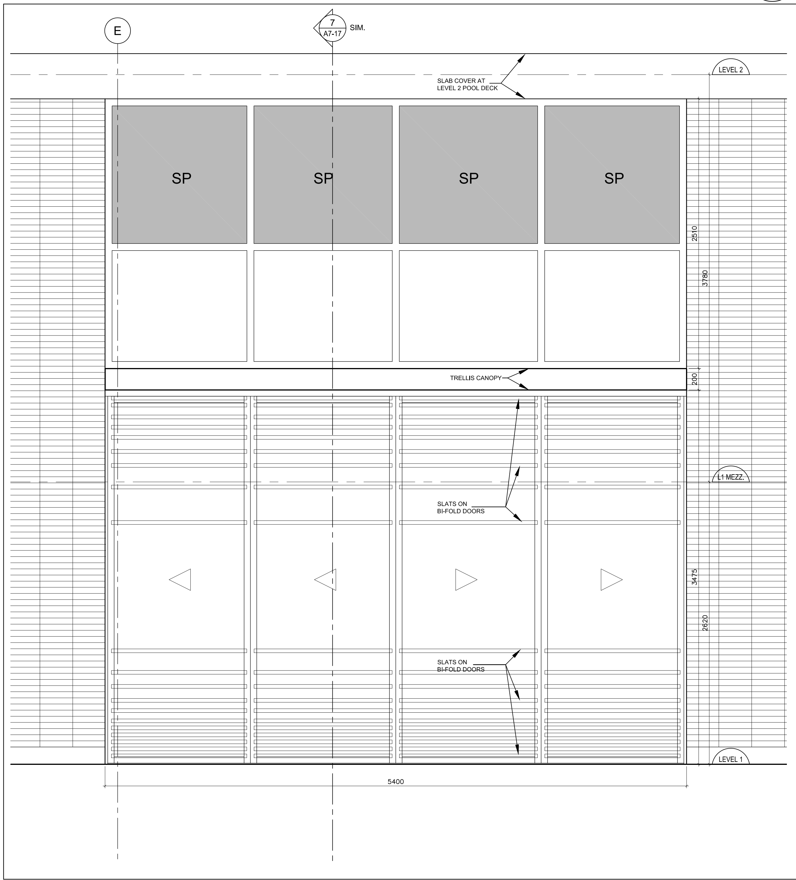
Elevation - Bi-Fold Door 1 @ Retail @ Level 1 1 A7-17 SCALE 1:20
