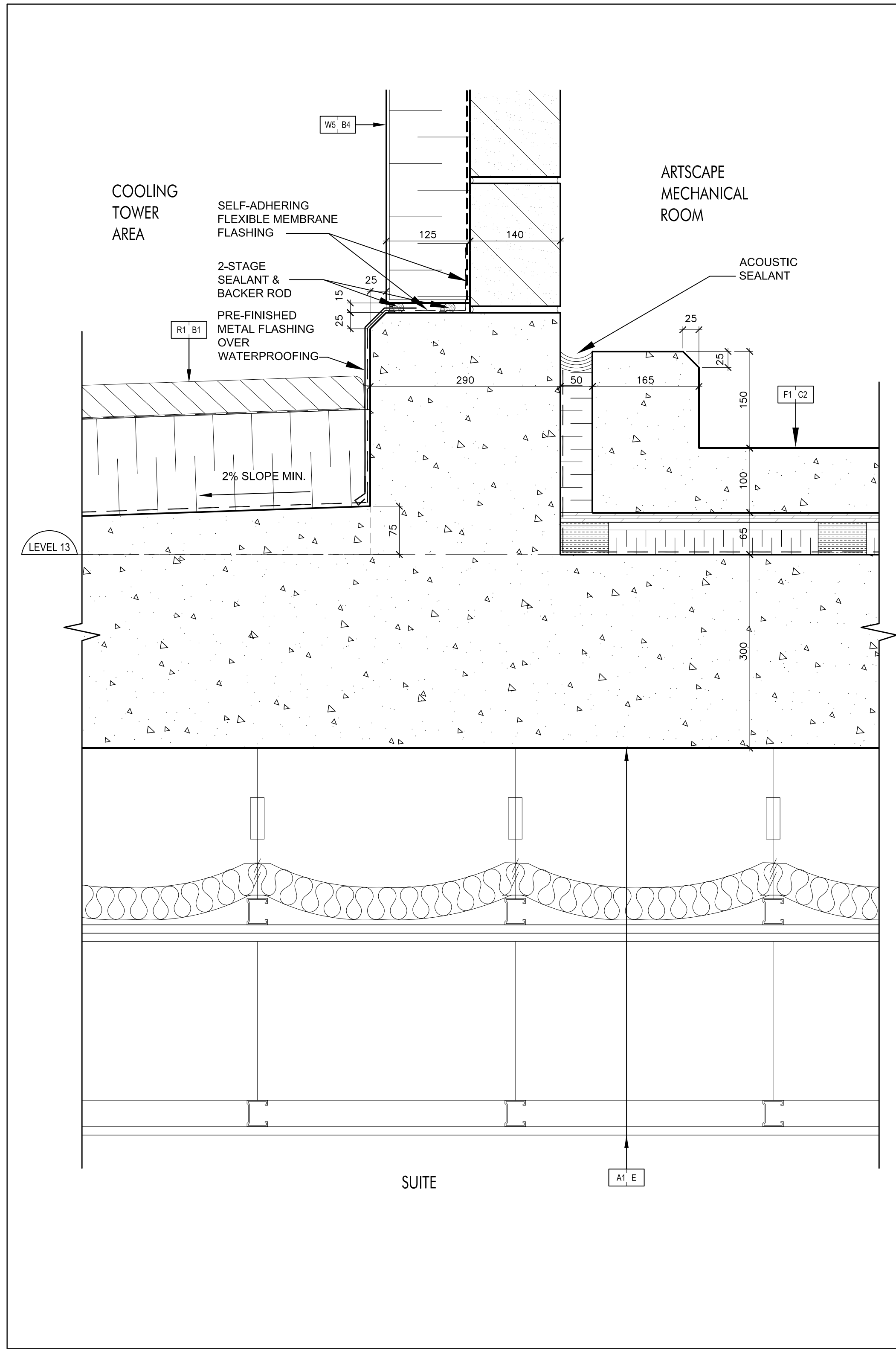
Conc. Curb @ Mechanical Room Floating Slab @ Level 13 (Ref. Wall Section 4/A7-01) SCALE 1:5 A7-14
