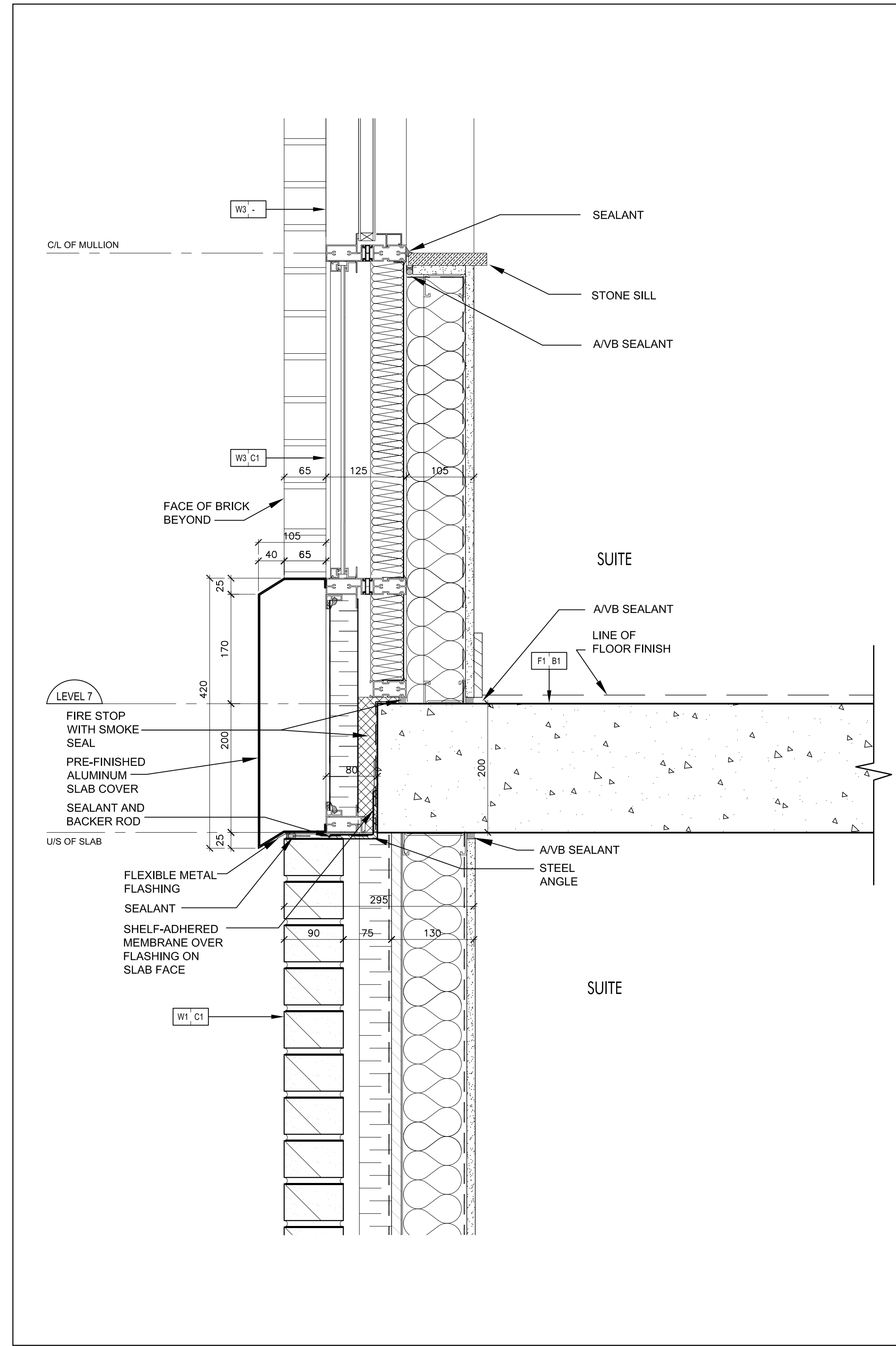
Pre-Finished Aluminum Slab Cover @ Level 7 (Ref. Wall Section 5/A7-01) SCALE 1:5 A7-14
