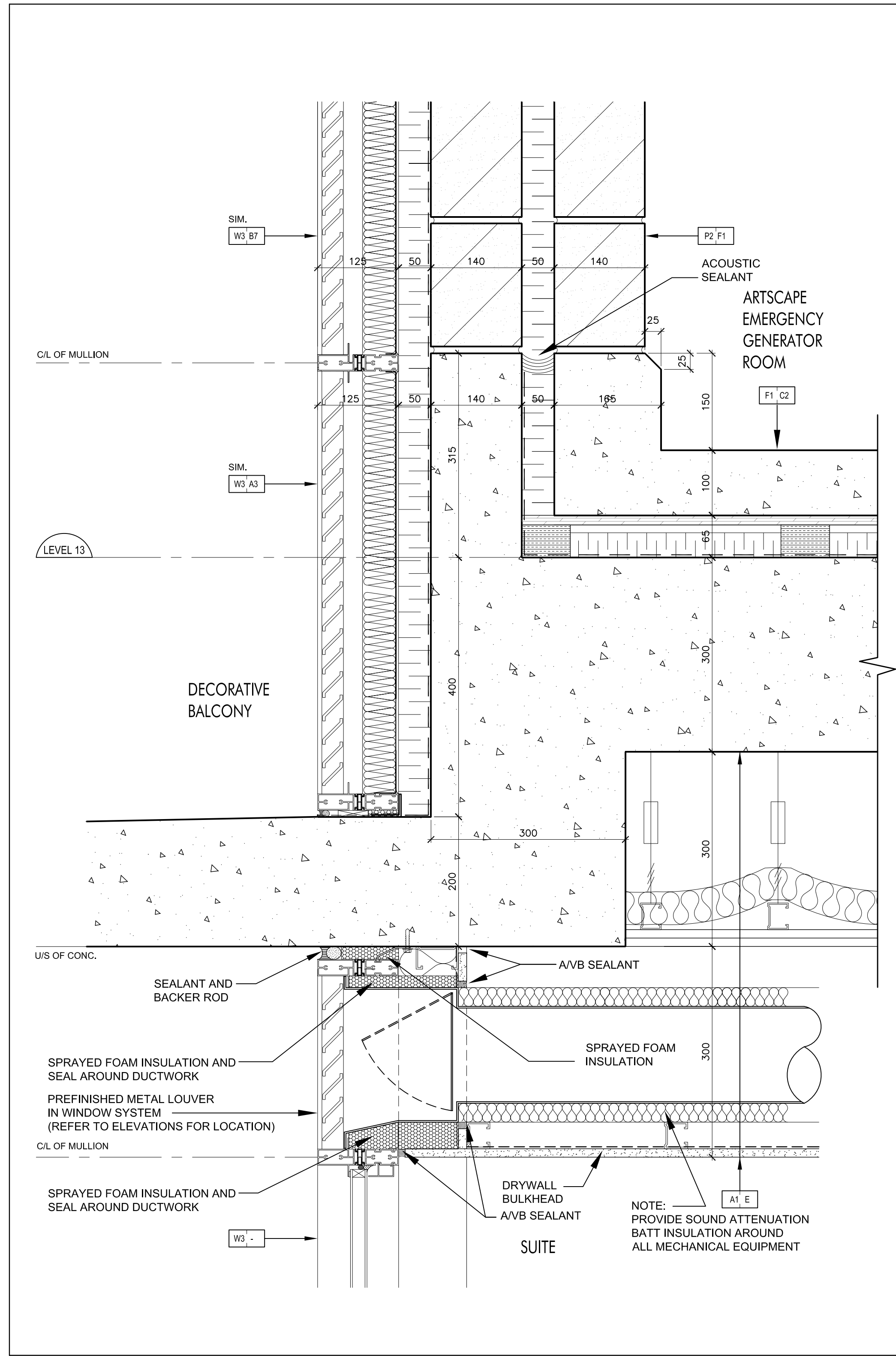
Floating Floor @ Emergency Generator Room @ Level 13 (Ref. Wall Section 6/A7-01) SCALE 1:5 A7-14
