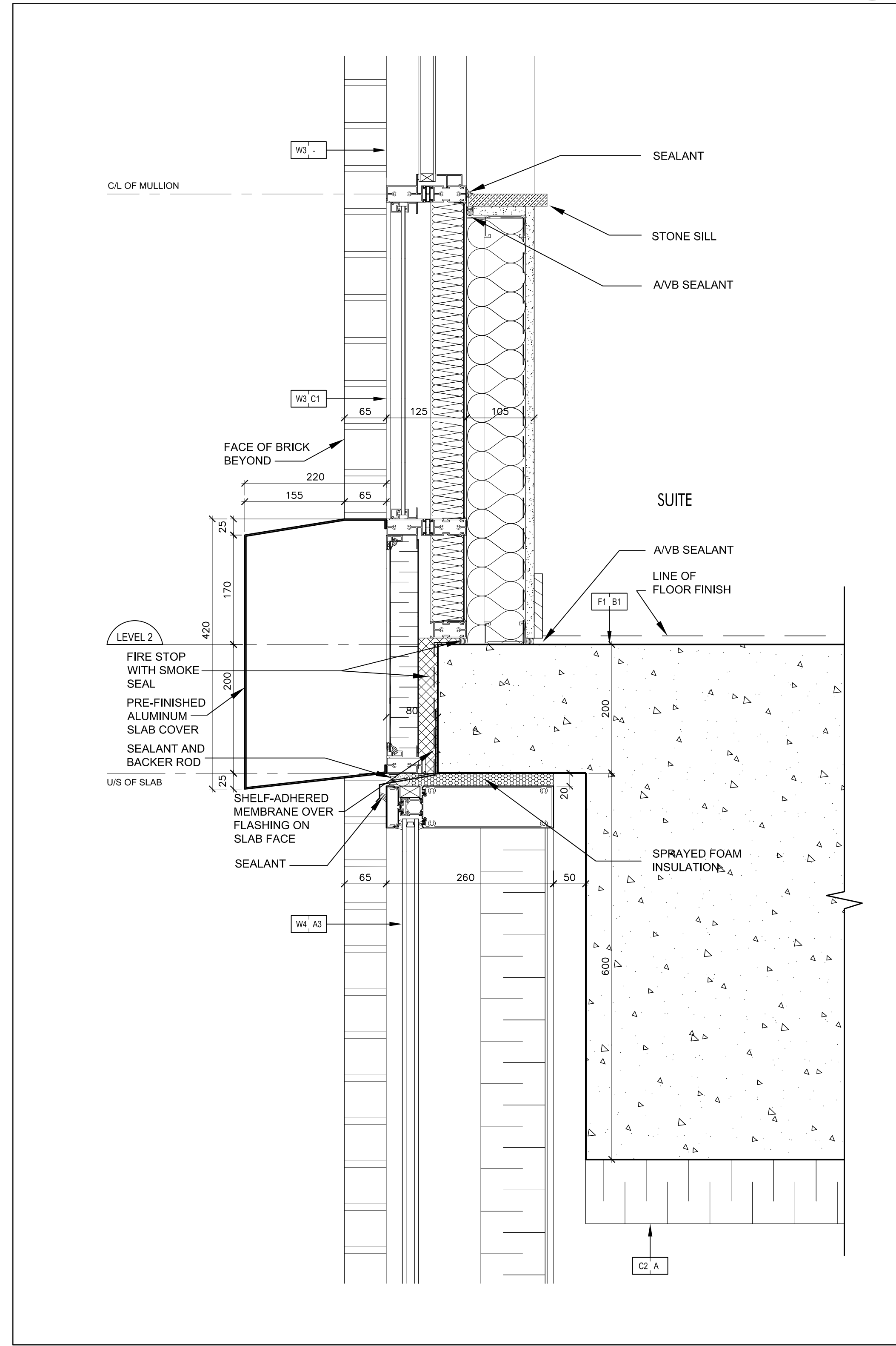
Pre-Fin. Alum. Slab Cover @ Window Wall & Curtain Wall-Level 2 (Ref. Wall Section 4/A7-01) SCALE 1:5 A7-14
