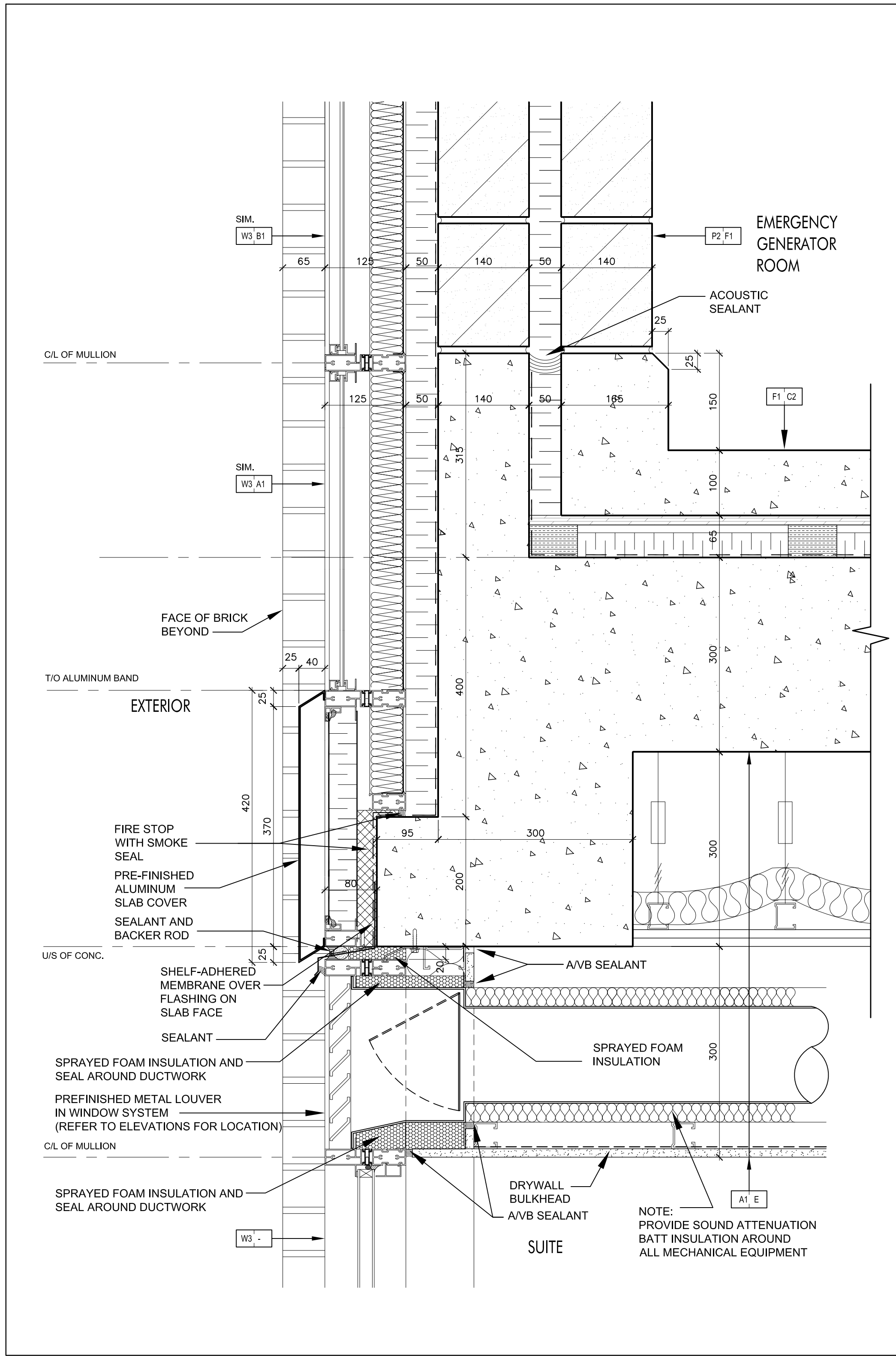
Floating Floor @ Emergency Generator Room @ Level 13 (Ref. Wall Section 7/A7-02) SCALE 1:5 A7-14
