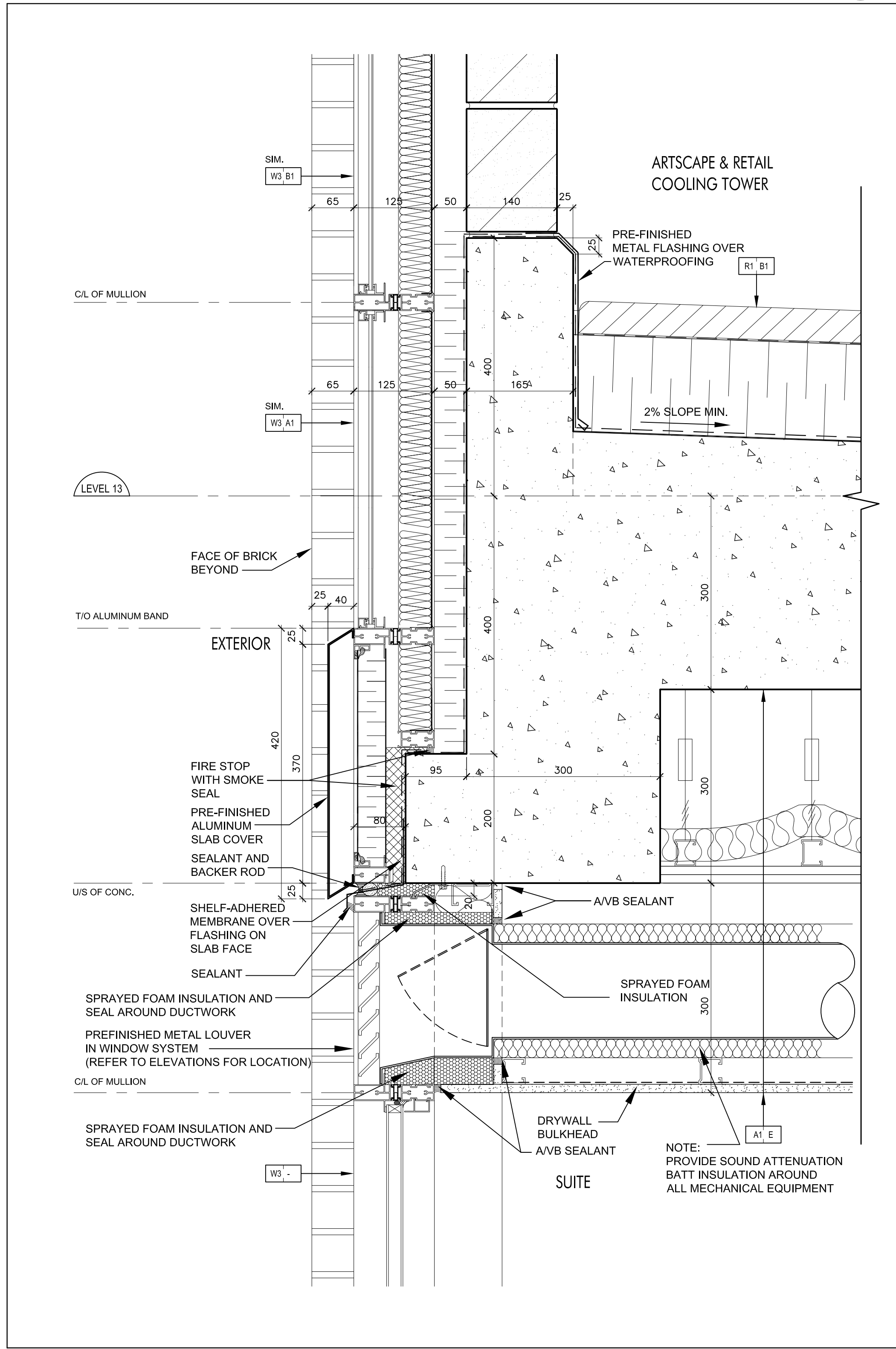
Window Wall Bypass & Pre-Fin. Alum. Slab Cover @ Level 13 (Ref. Wall Section 4/A7-01) SCALE 1:5 A7-14
