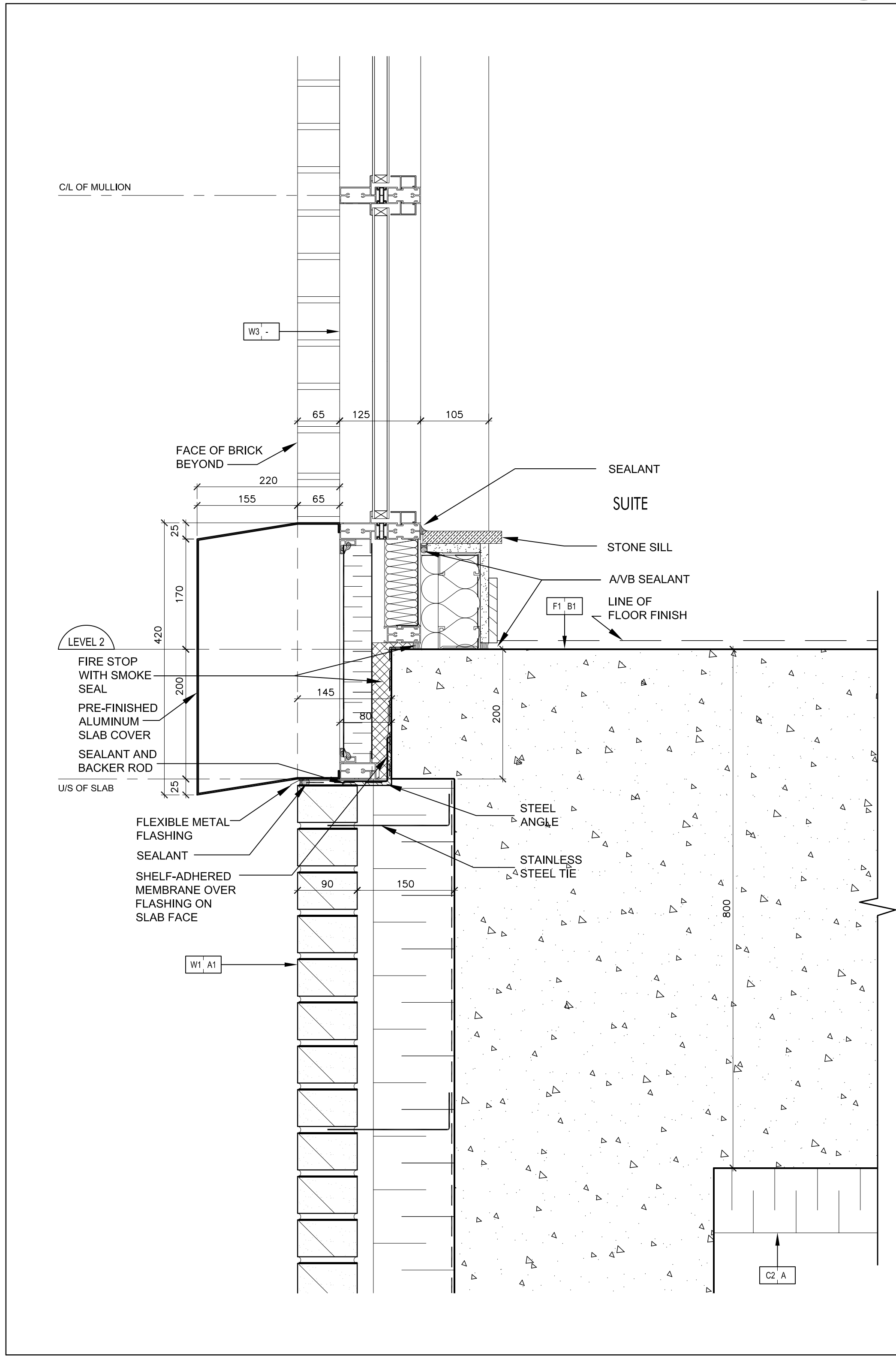
Pre-Fin. Alum. Slab Cover @ Window Wall & Brick Wall-Level 2 (Ref. Wall Section 4/A7-09) SCALE 1:5 A7-14
