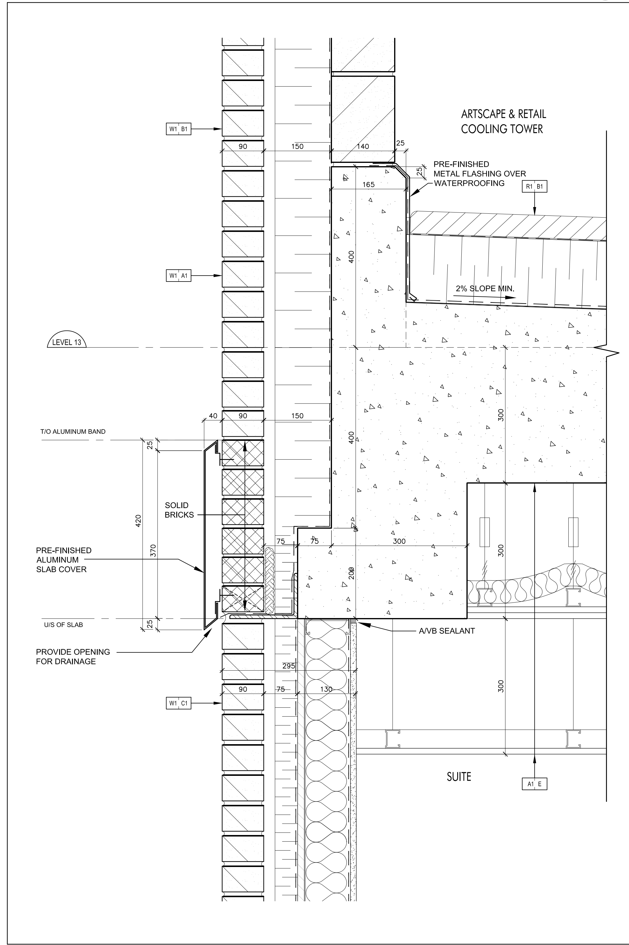
Pre-Finished Aluminum Slab Cover @ Level 13 (Ref. Wall Section 5/A7-01) SCALE 1:5 A7-14
