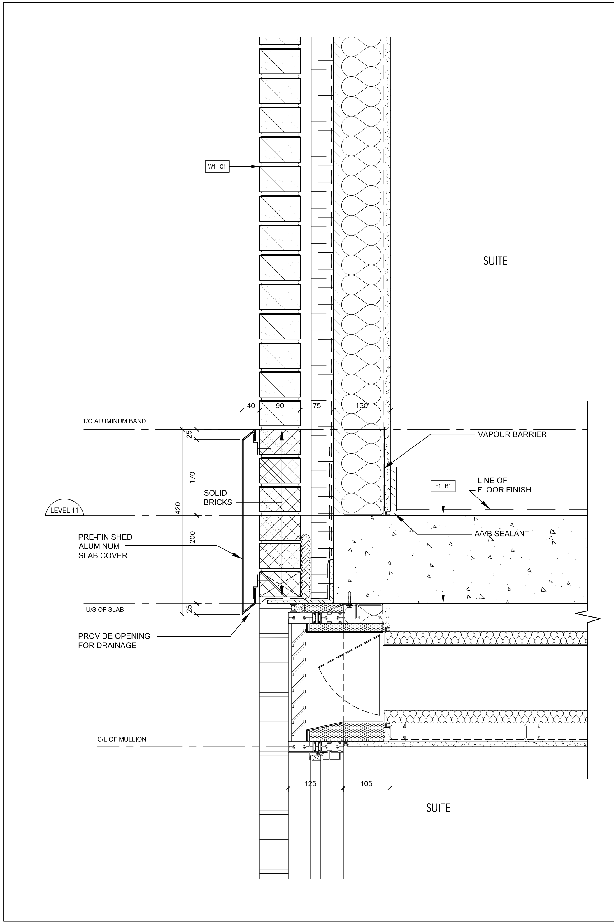
Pre-Finished Aluminum Slab Cover @ Level 11 (Ref. Wall Section 5/A7-01) SCALE 1:5 A7-14
