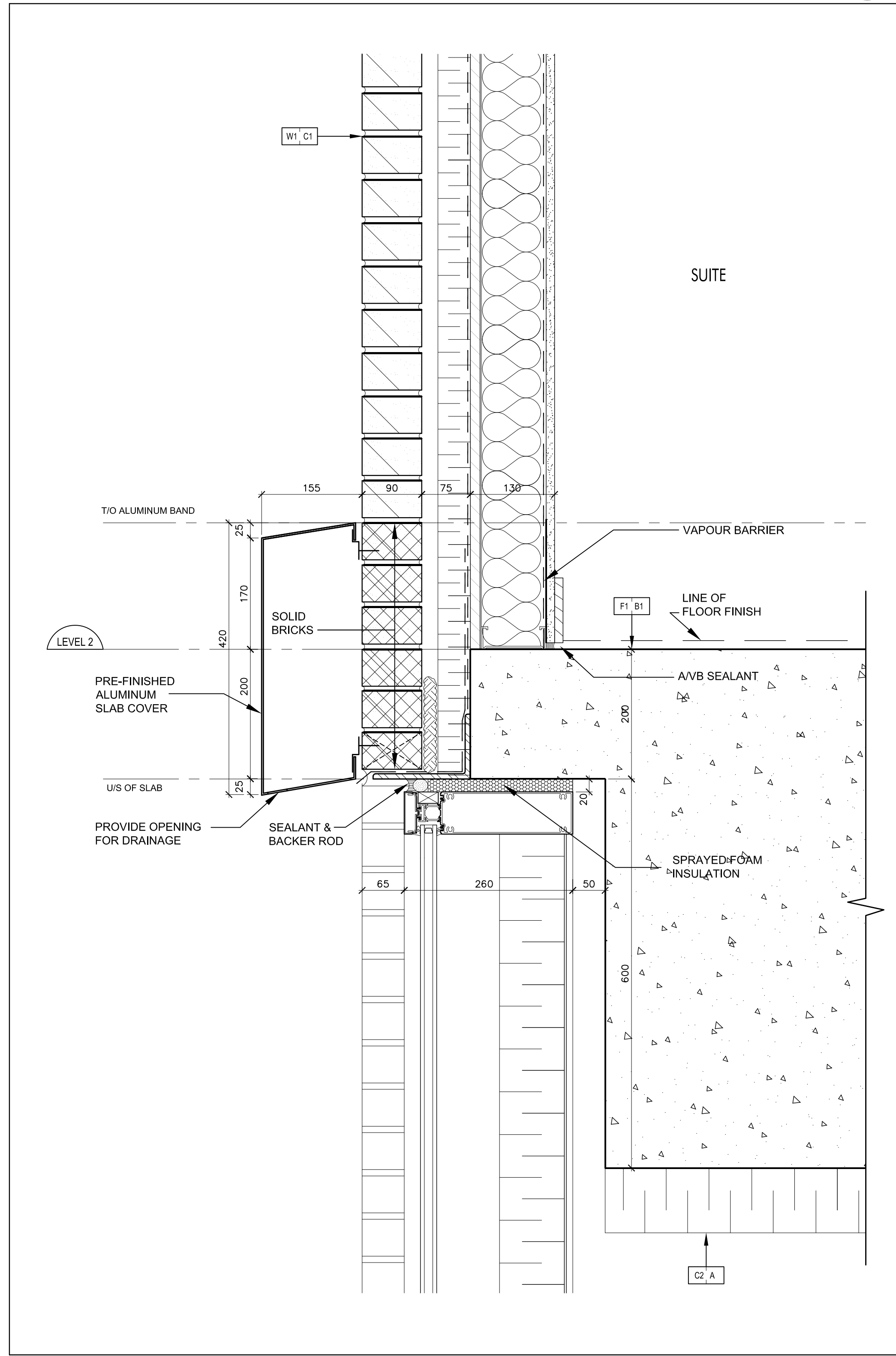
Pre-Fin. Alum. Slab Cover @ Brick Wall & Curtain Wall-Level 2 (Ref. Wall Section 5/A7-01) SCALE 1:5 A7-14
