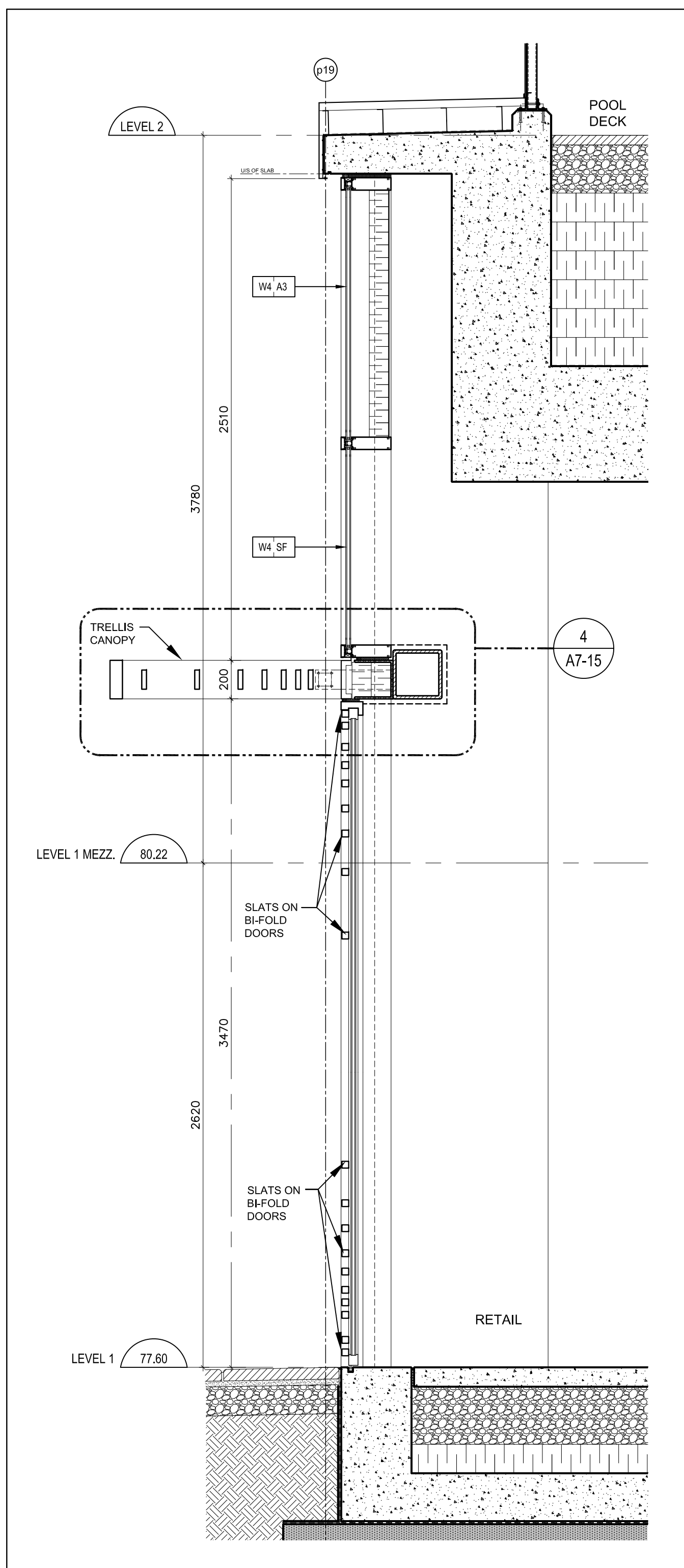
Section thru Bi-Fold Door @ Retail @ Level 1
