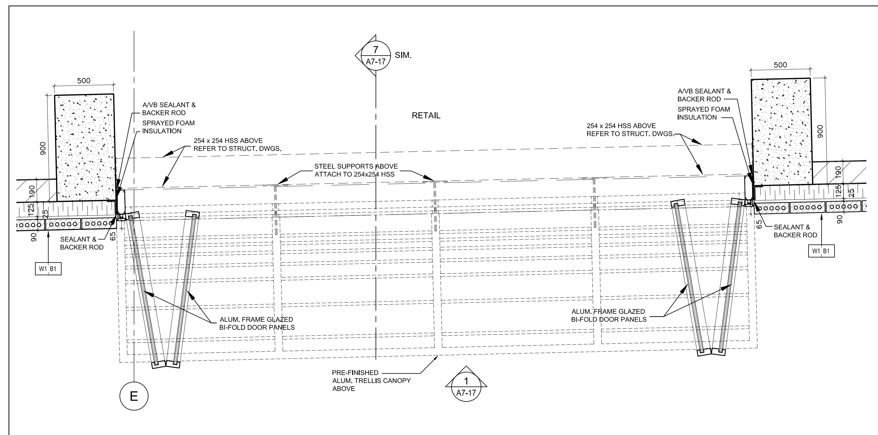
Plan - Bi-Fold Door 1 @ Retail @ Level 1
