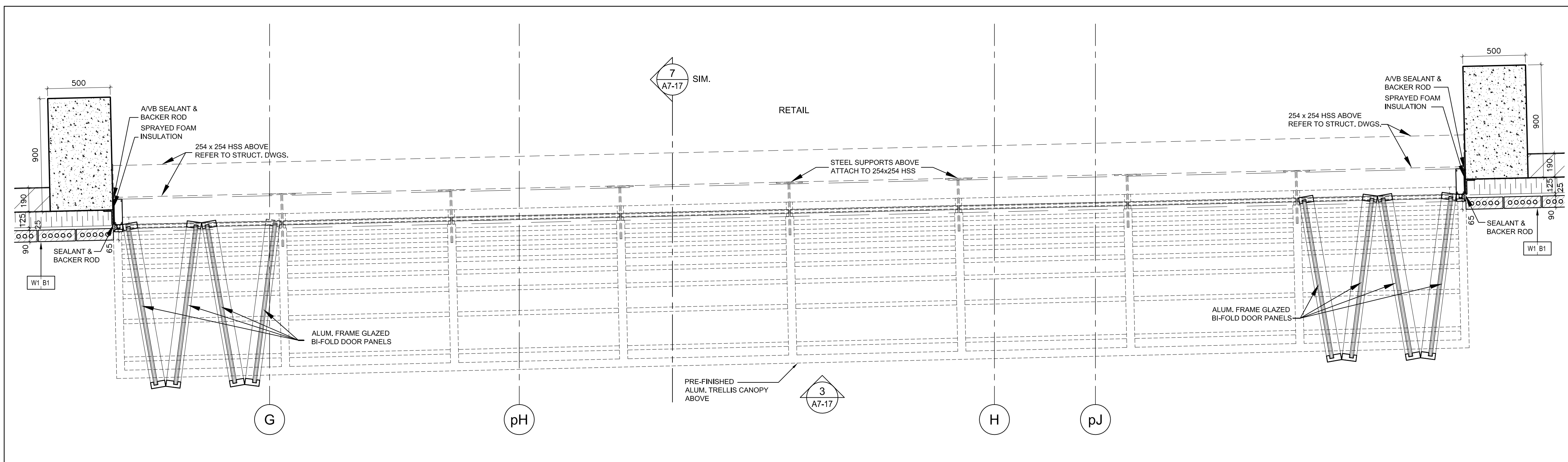
Plan - Bi-Fold Door 2 @ Retail @ Level 1
