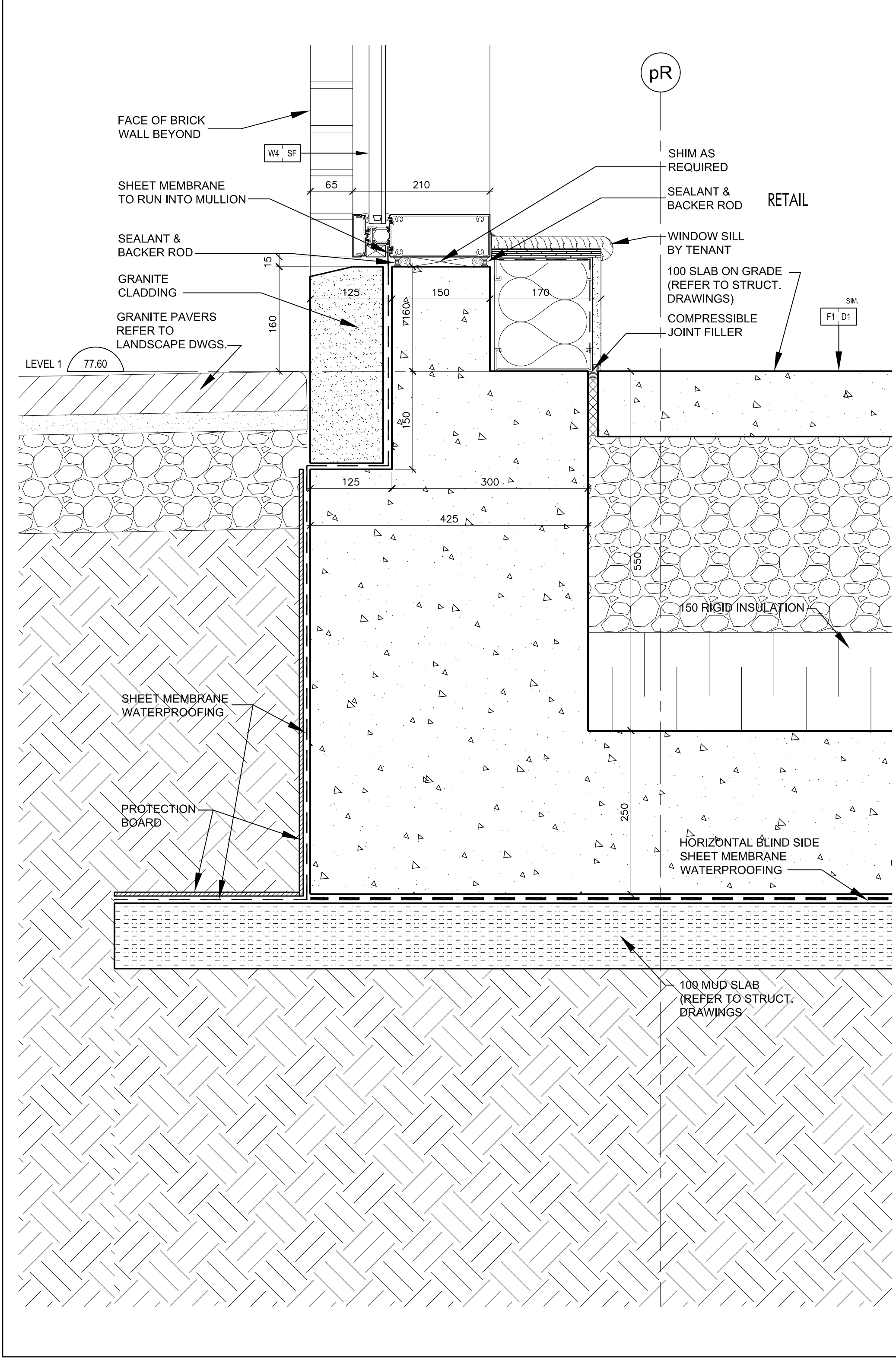
Curtain Wall Sill @ Retail 7 SCALE 1:5 A7-08
