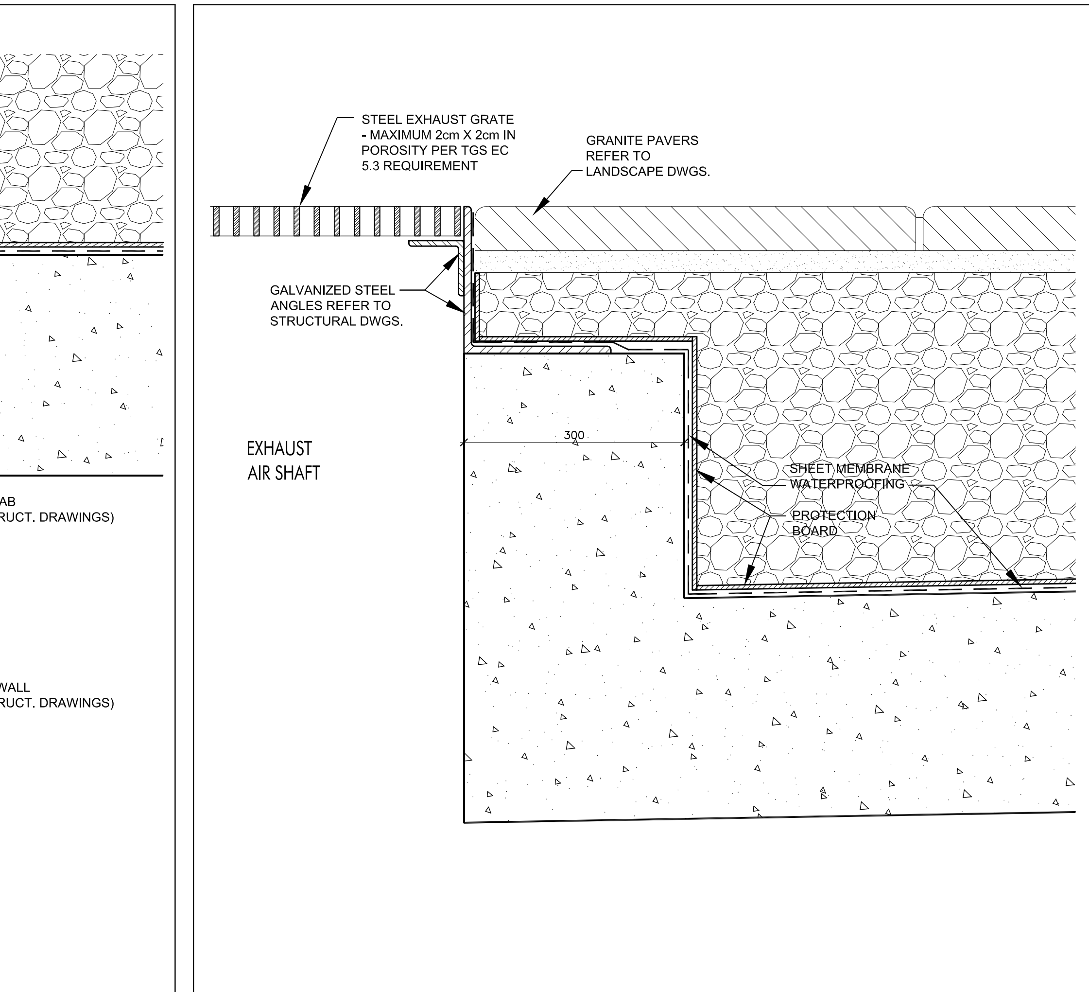
Section thru Exhaust Air Shaft Steel Grate @ Level 1 3 SCALE 1:5 A7-08
