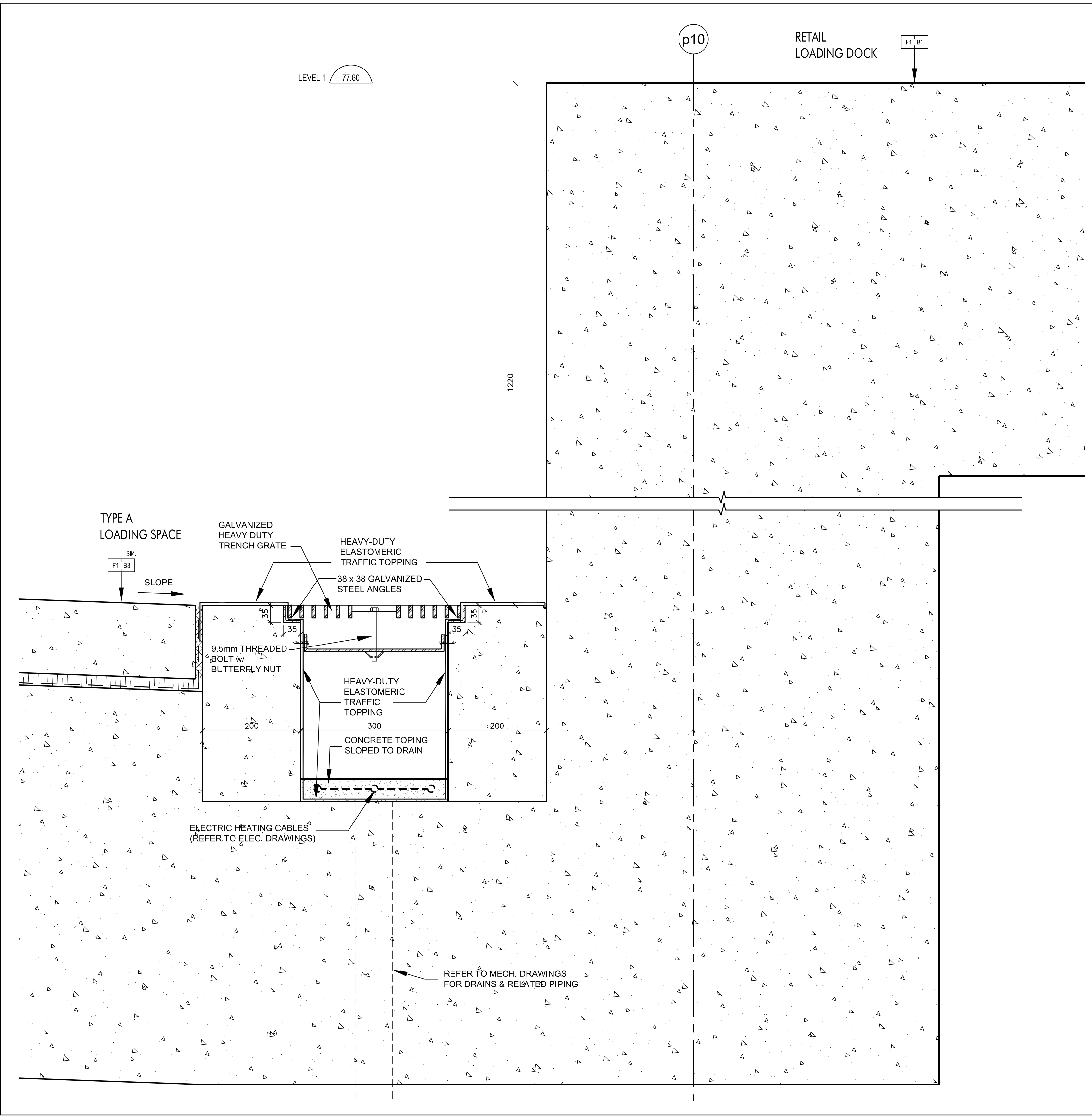
Trench Detail @ Loading Space 10 SCALE 1:5 A7-08
