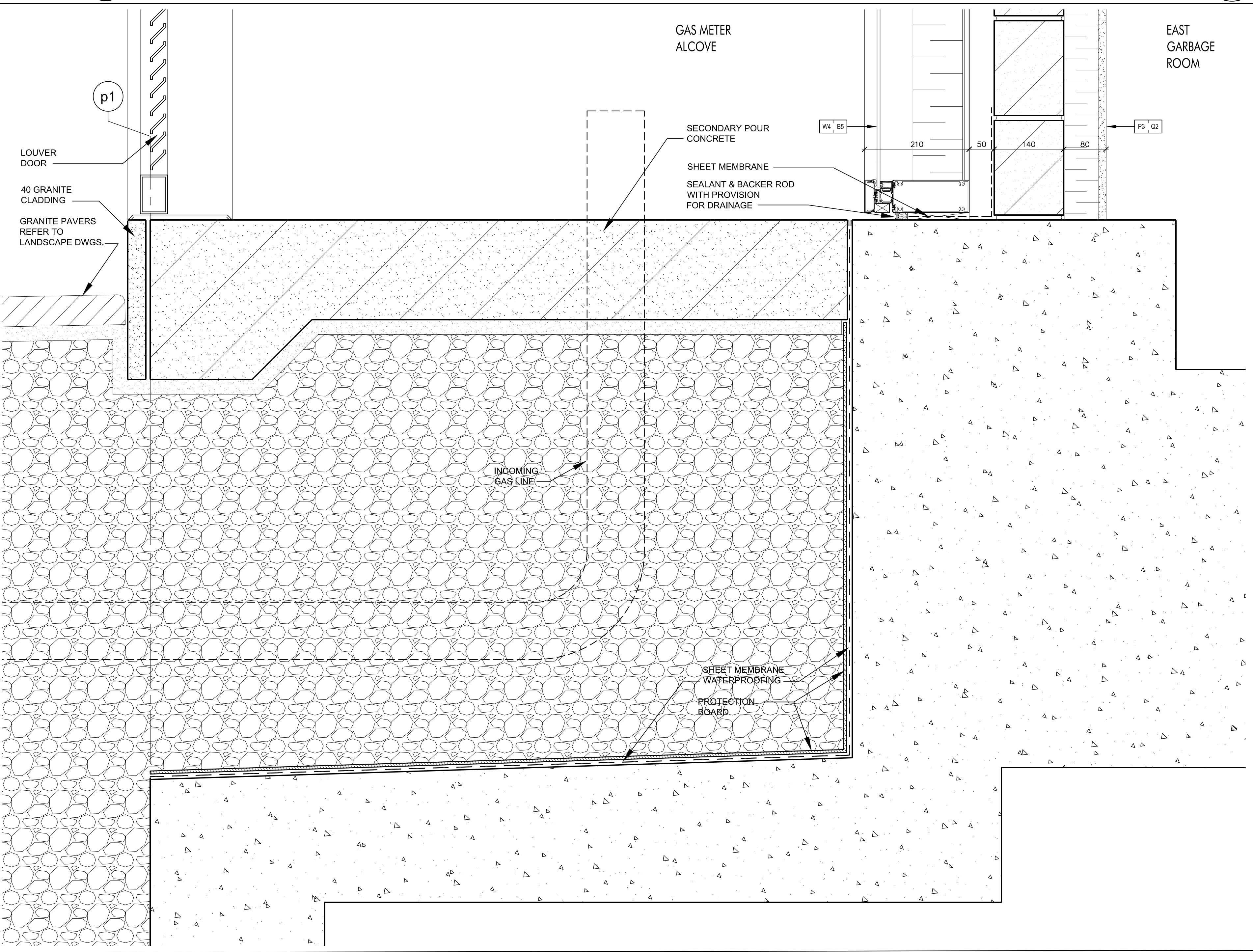
Curtain Wall Sill @ Gas Meter Alcove 9 SCALE 1:5 A7-08
