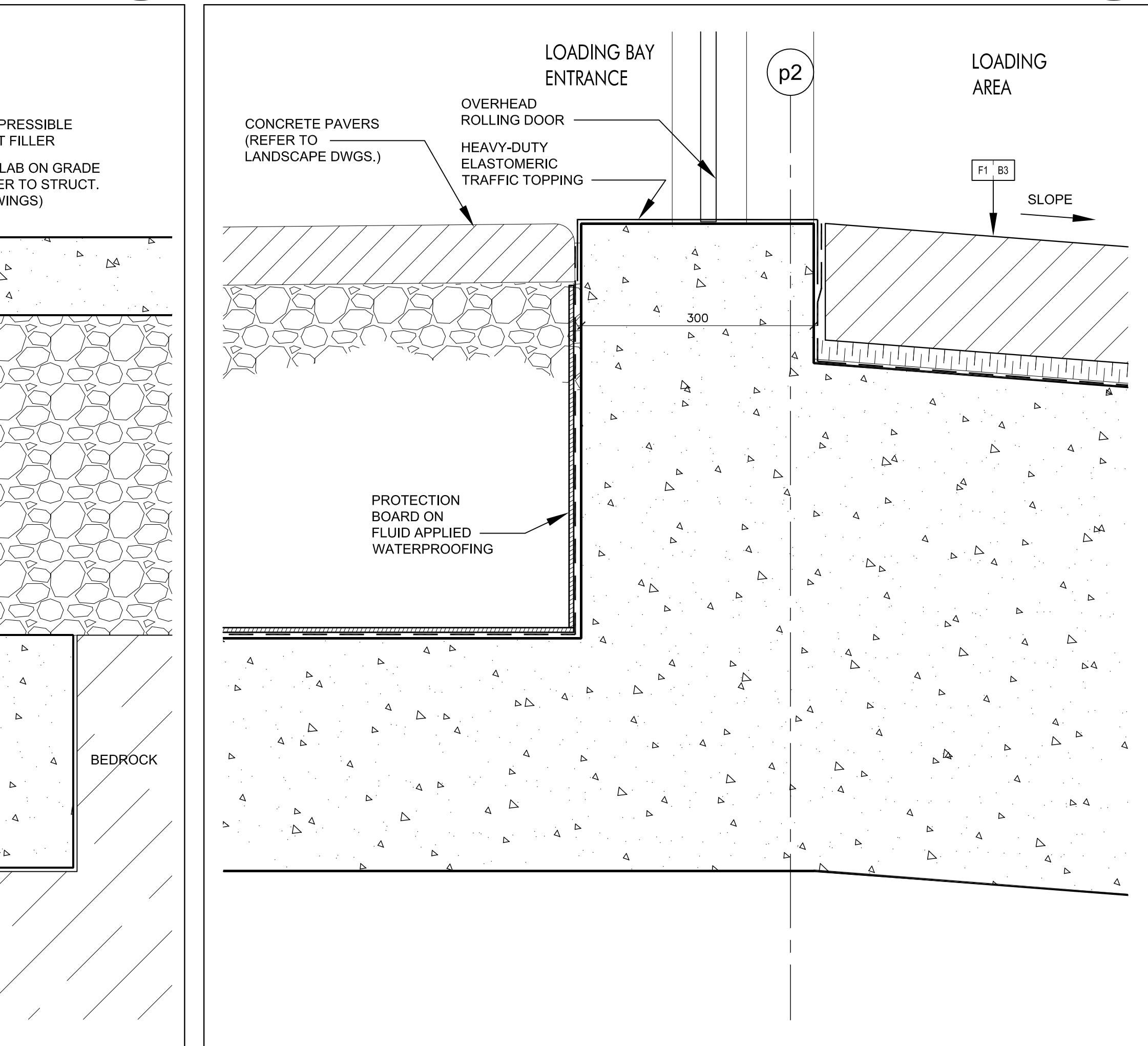
Entrance & O/H Door @ Loading Area 2 SCALE 1:5 A7-08
