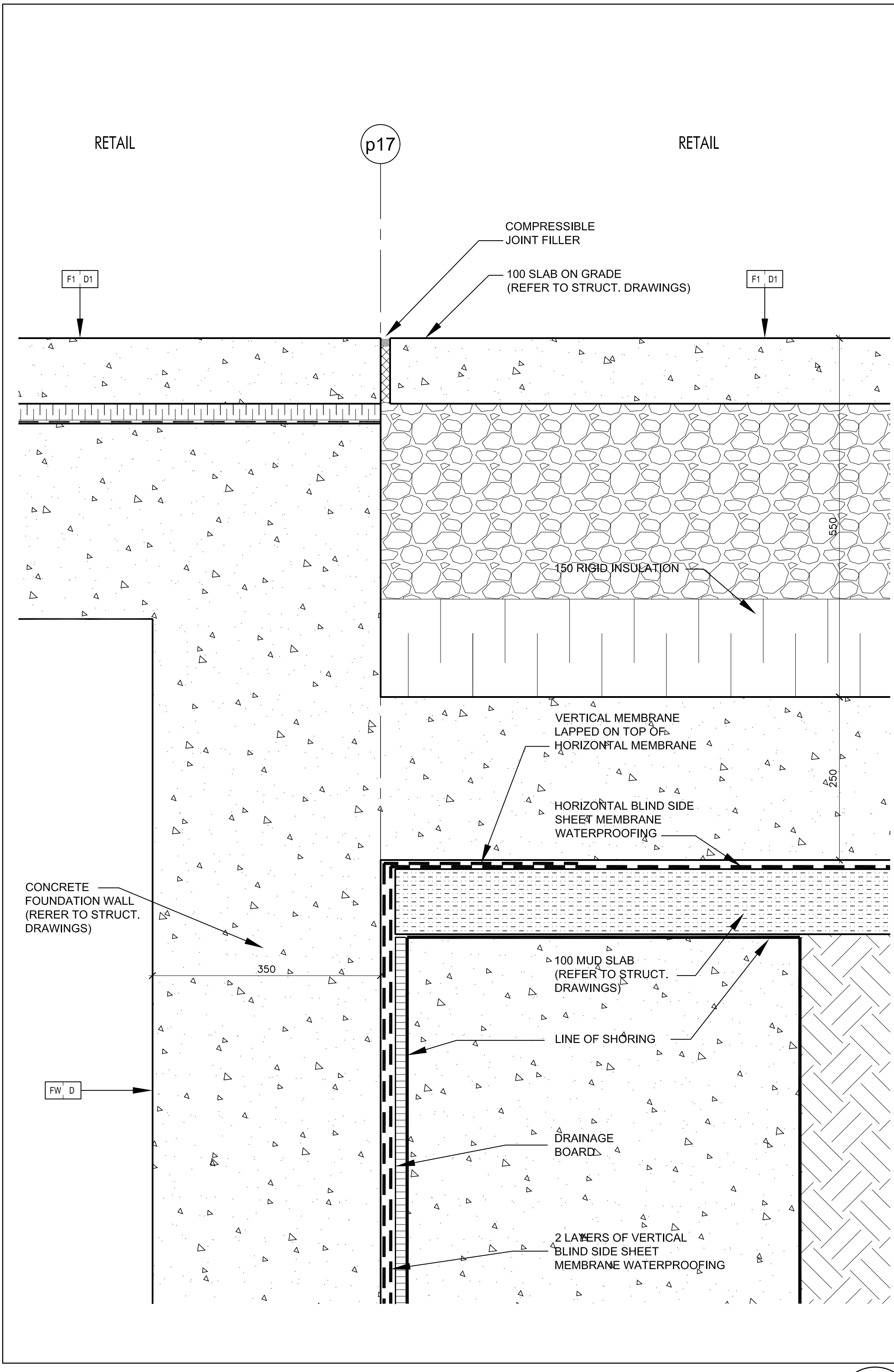
Foundation Wall @ Caisson Wall 8 SCALE 1:5 A7-08
