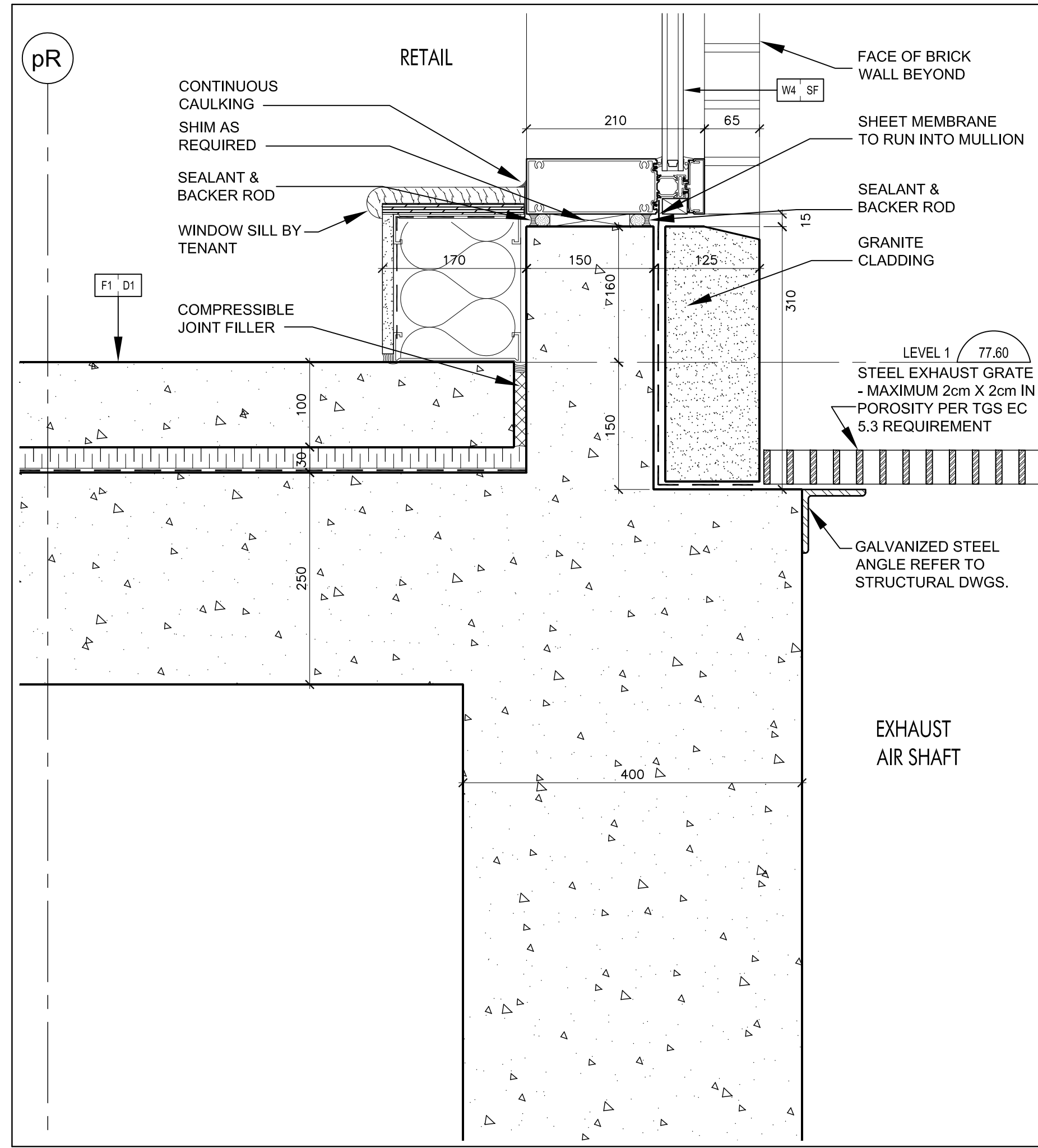
Curtain Wall Sill @ Retail & Steel Grate 4 SCALE 1:5 A7-08
