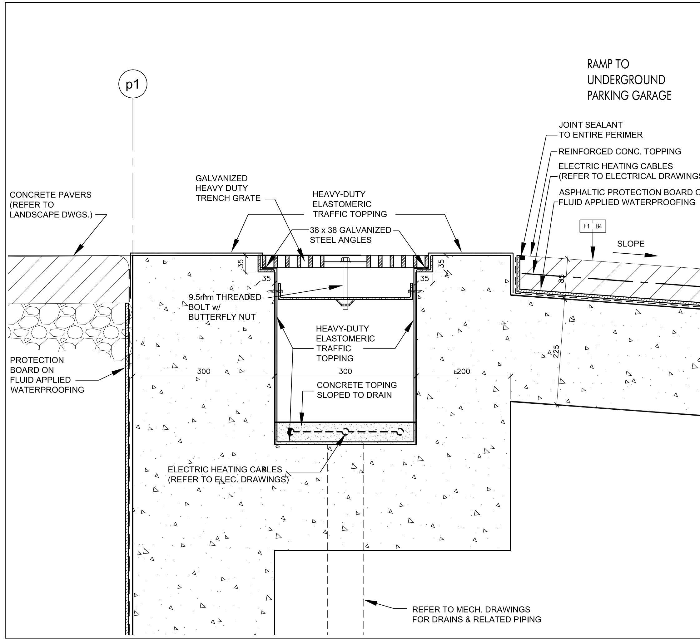
Entrance to Residential Parking 1 SCALE 1:5 A7-08
