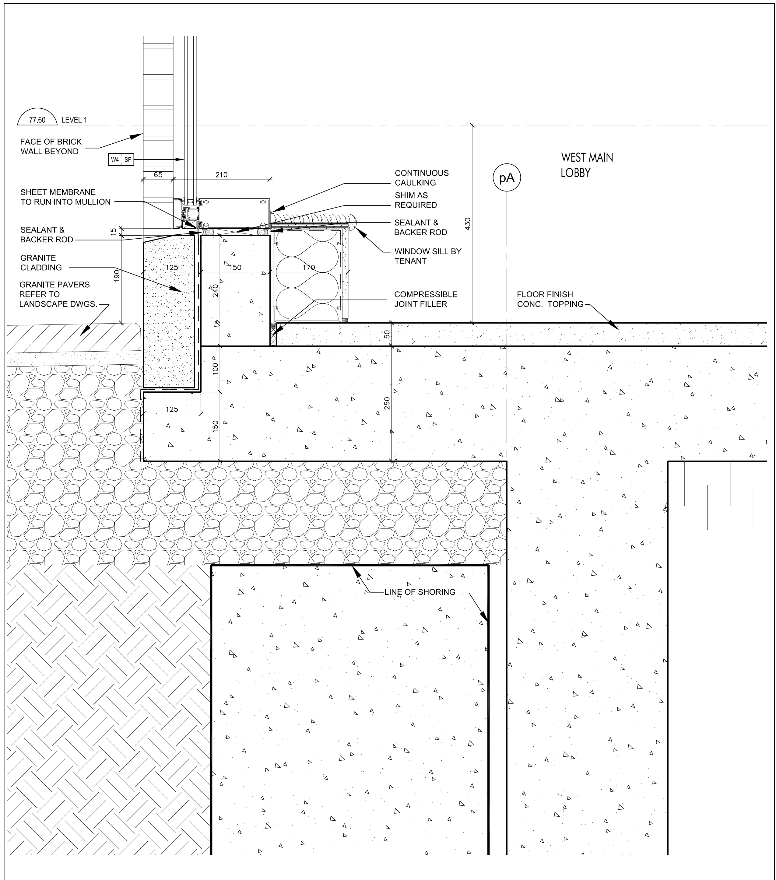
Curtain Wall Sill @ West Main Lobby 11 SCALE 1:5 A7-08
