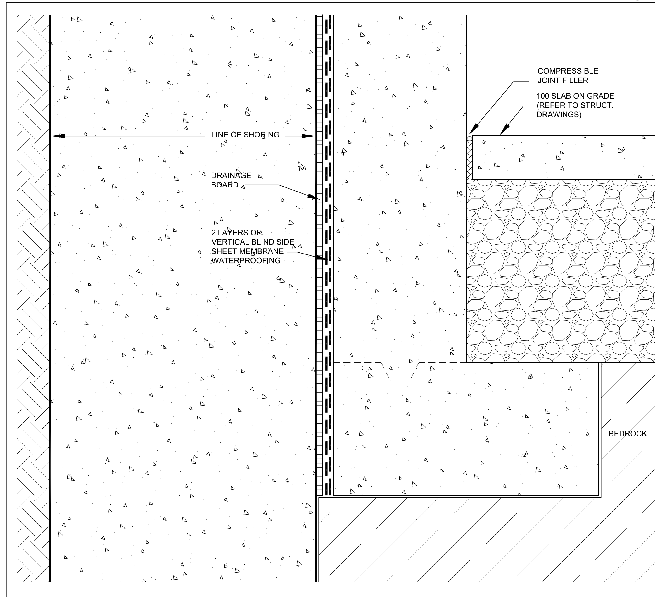
Foundation Wall @ Caisson Wall 5 SCALE 1:5 A7-08
