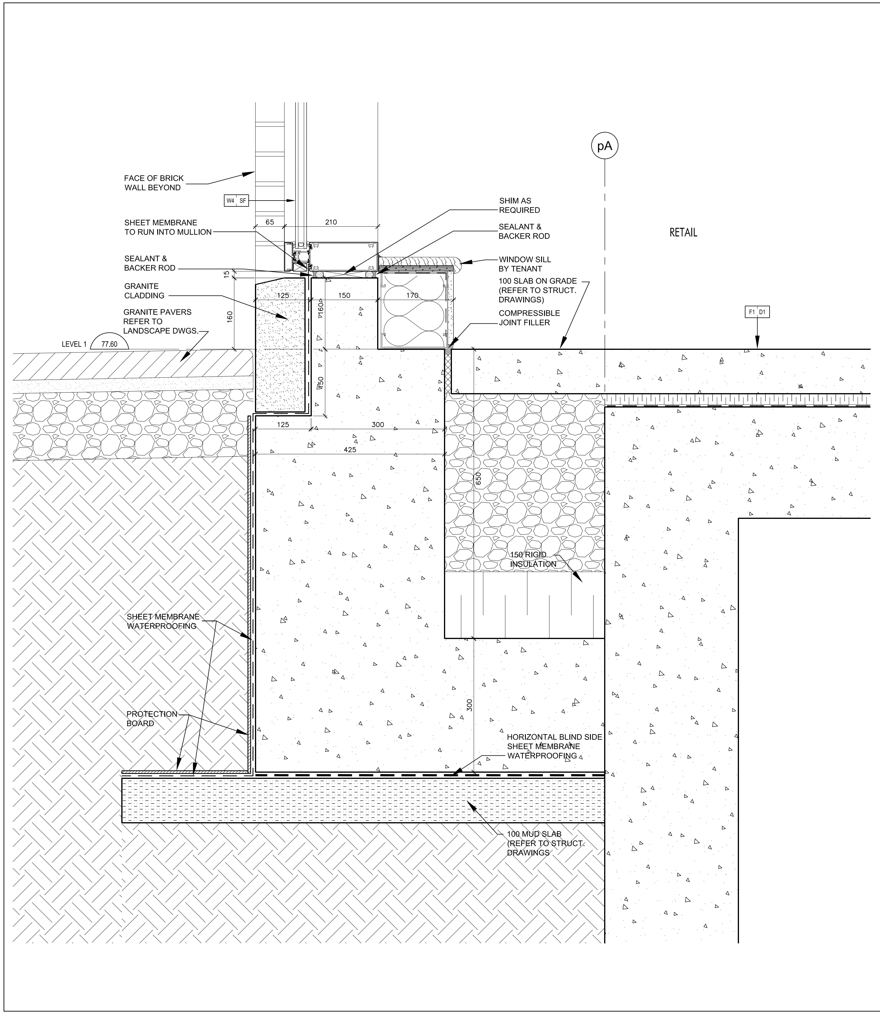
Curtain Wall Sill @ Retail 12 SCALE 1:5 A7-08
