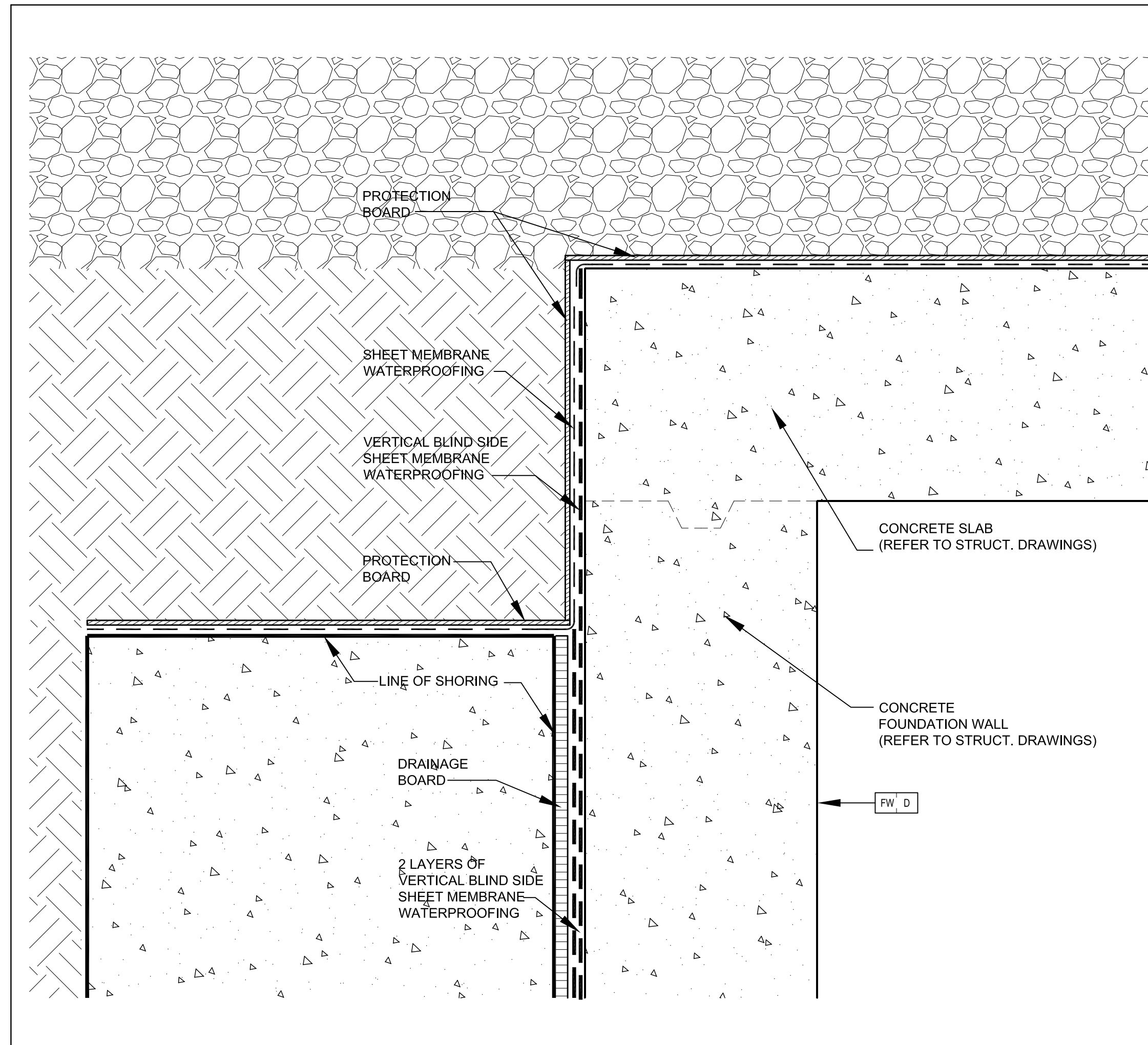
Foundation Wall @ Caisson Wall 6 SCALE 1:5 A7-08
