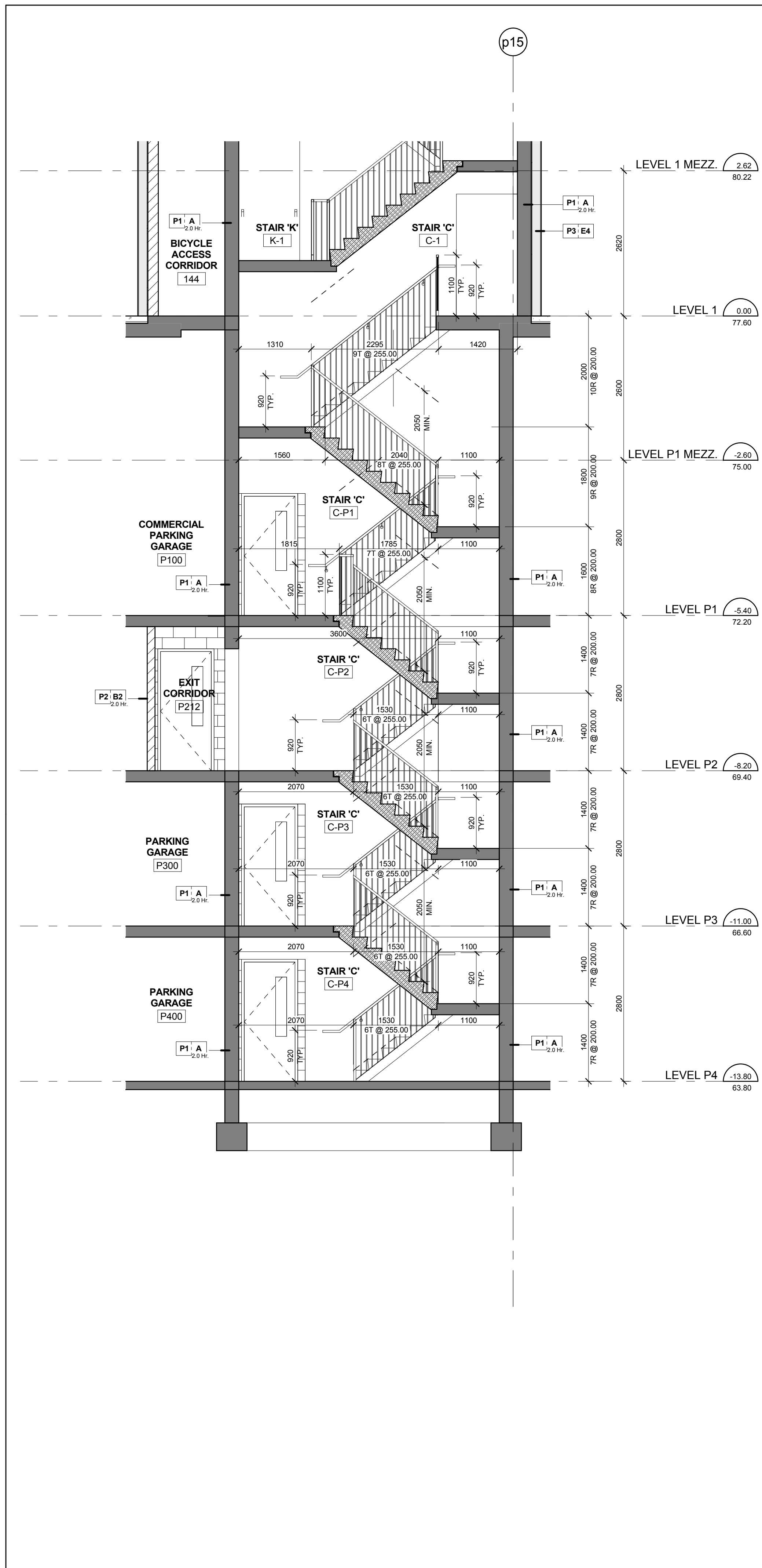
Stair 'C' - Stair Section Levels P4 - 1 Mezzanine Scale: 1 : 50 A6-02
