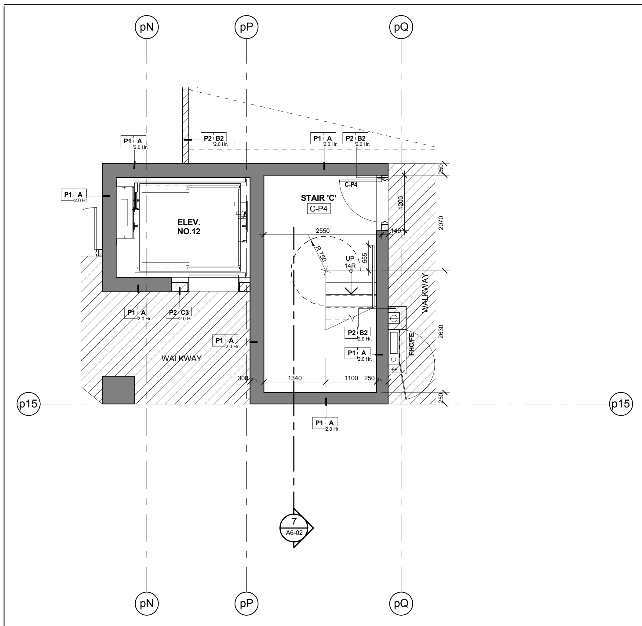
Stair 'C' - Stair Plan - Level P4 Scale: 1 : 50 A6-02
