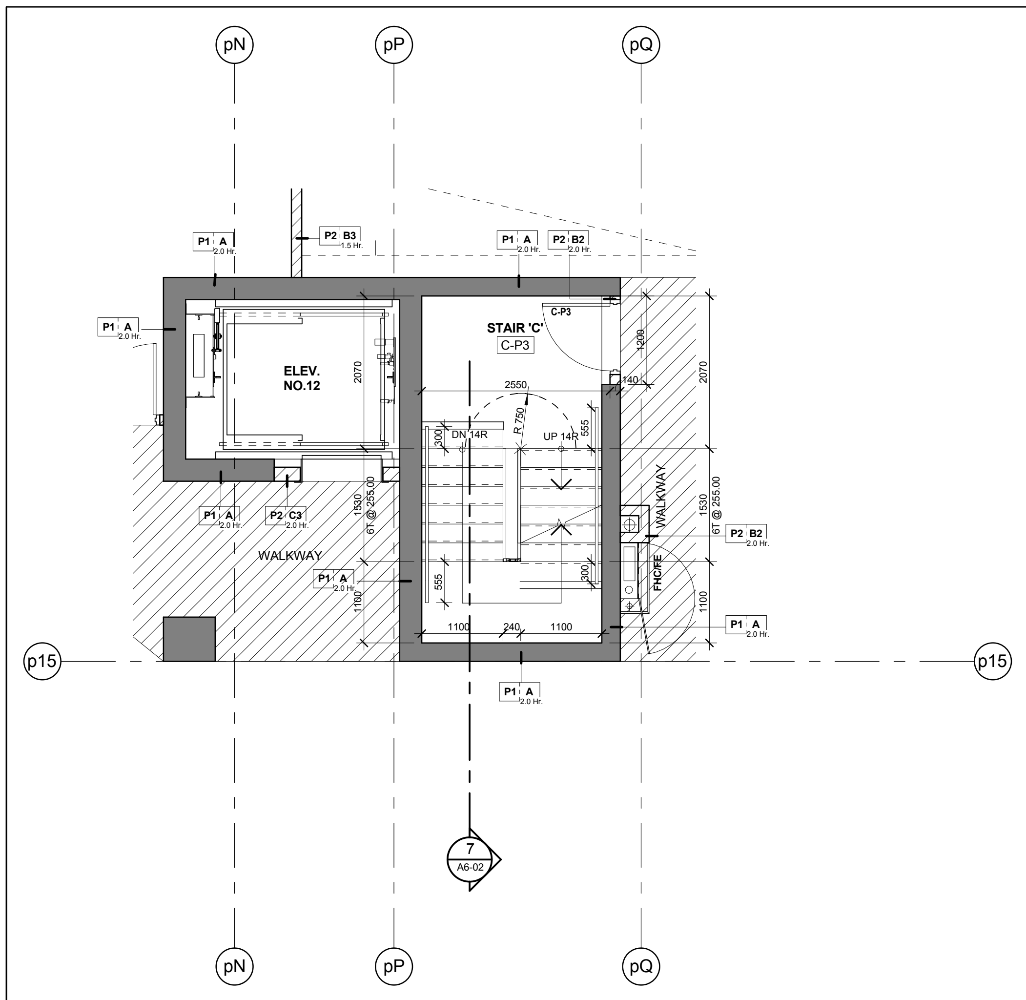
Stair 'C' - Stair Plan - Level P3 Scale: 1 : 50 A6-02
