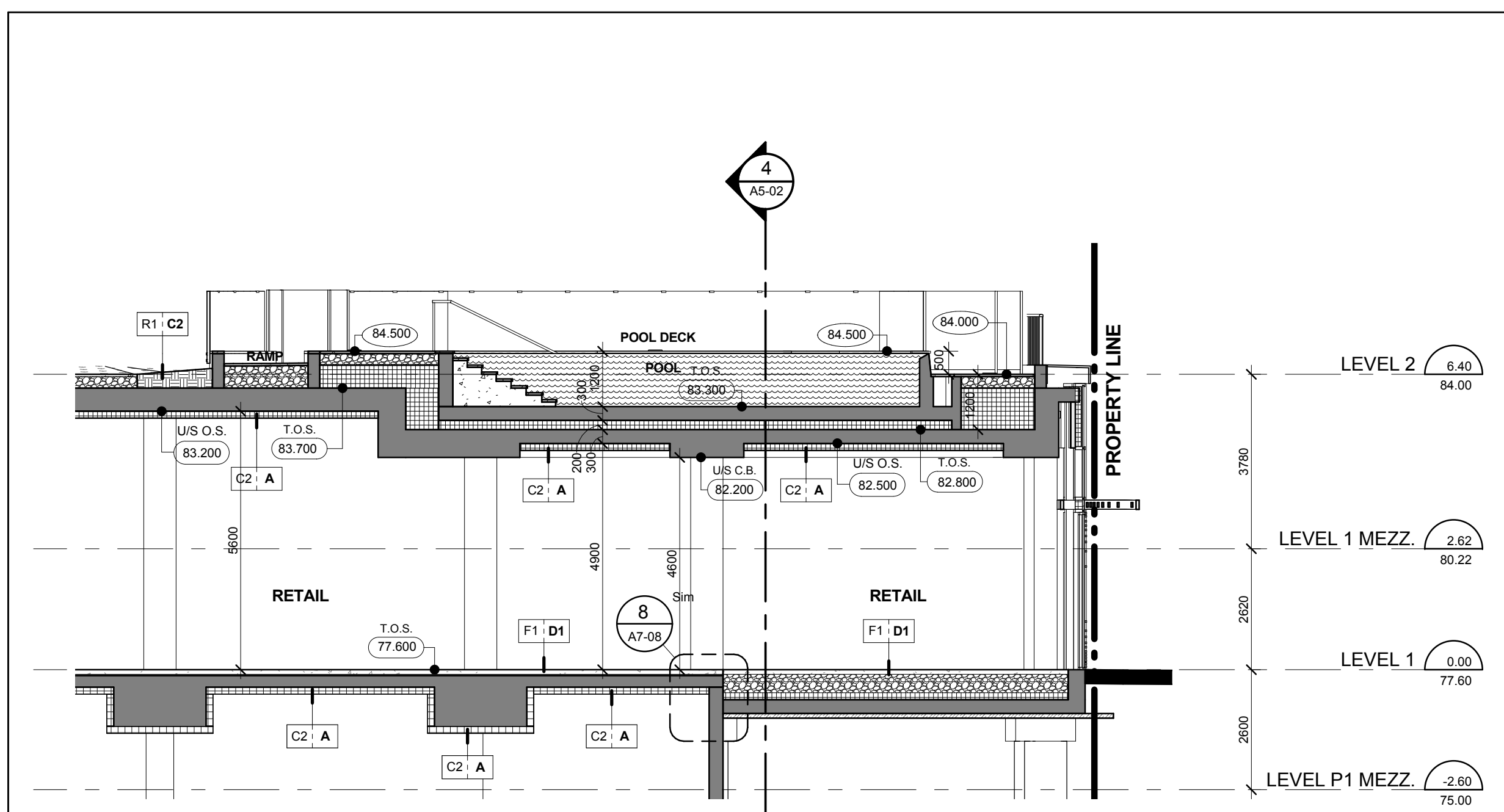
North - South Pool Section Along Gridline J 3 A5-02 Scale: 1 : 100
