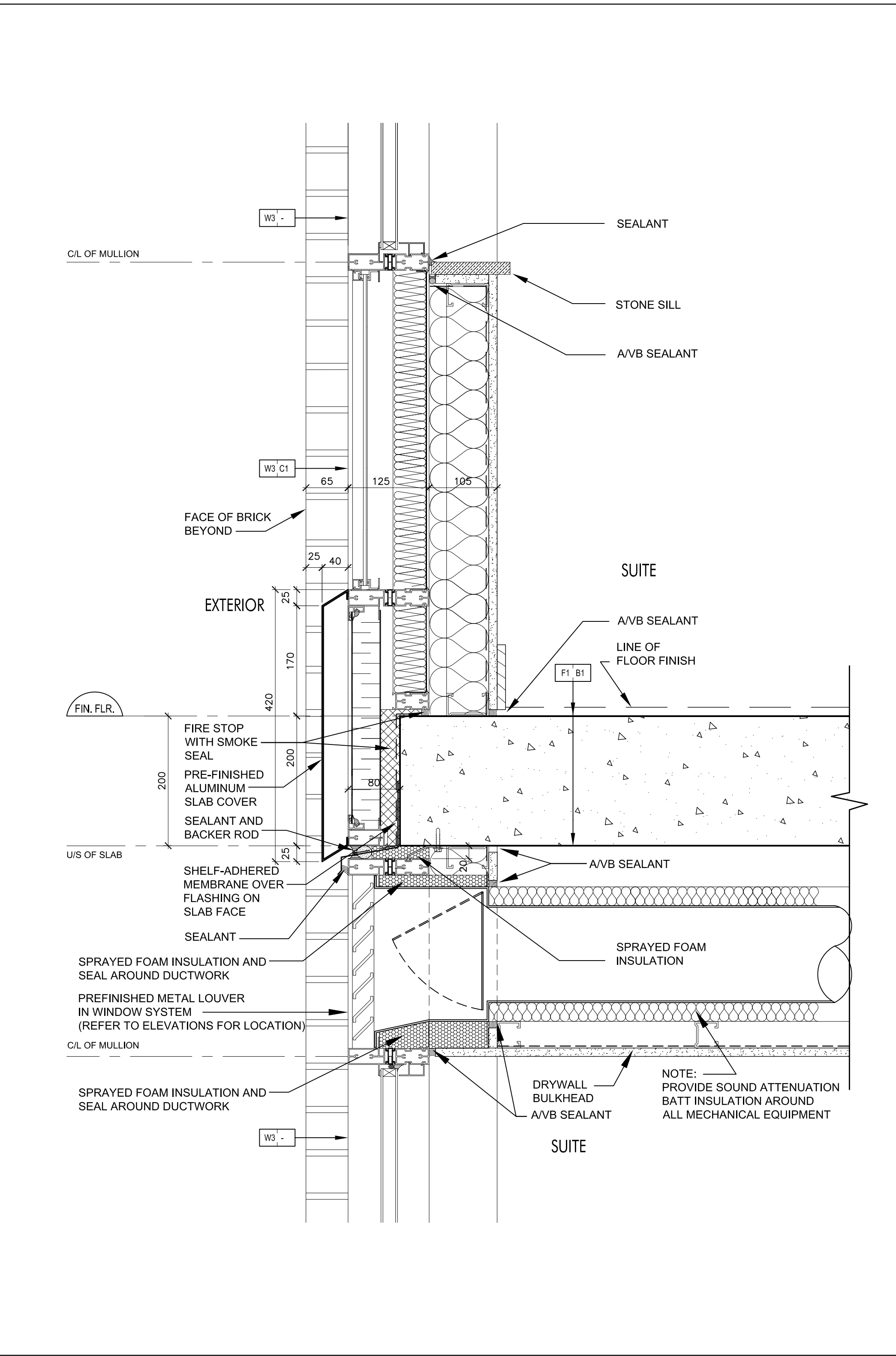
Pre-Finished Aluminum Slab Cover @ Window Wall 7 SCALE: 1:5 A7-12
