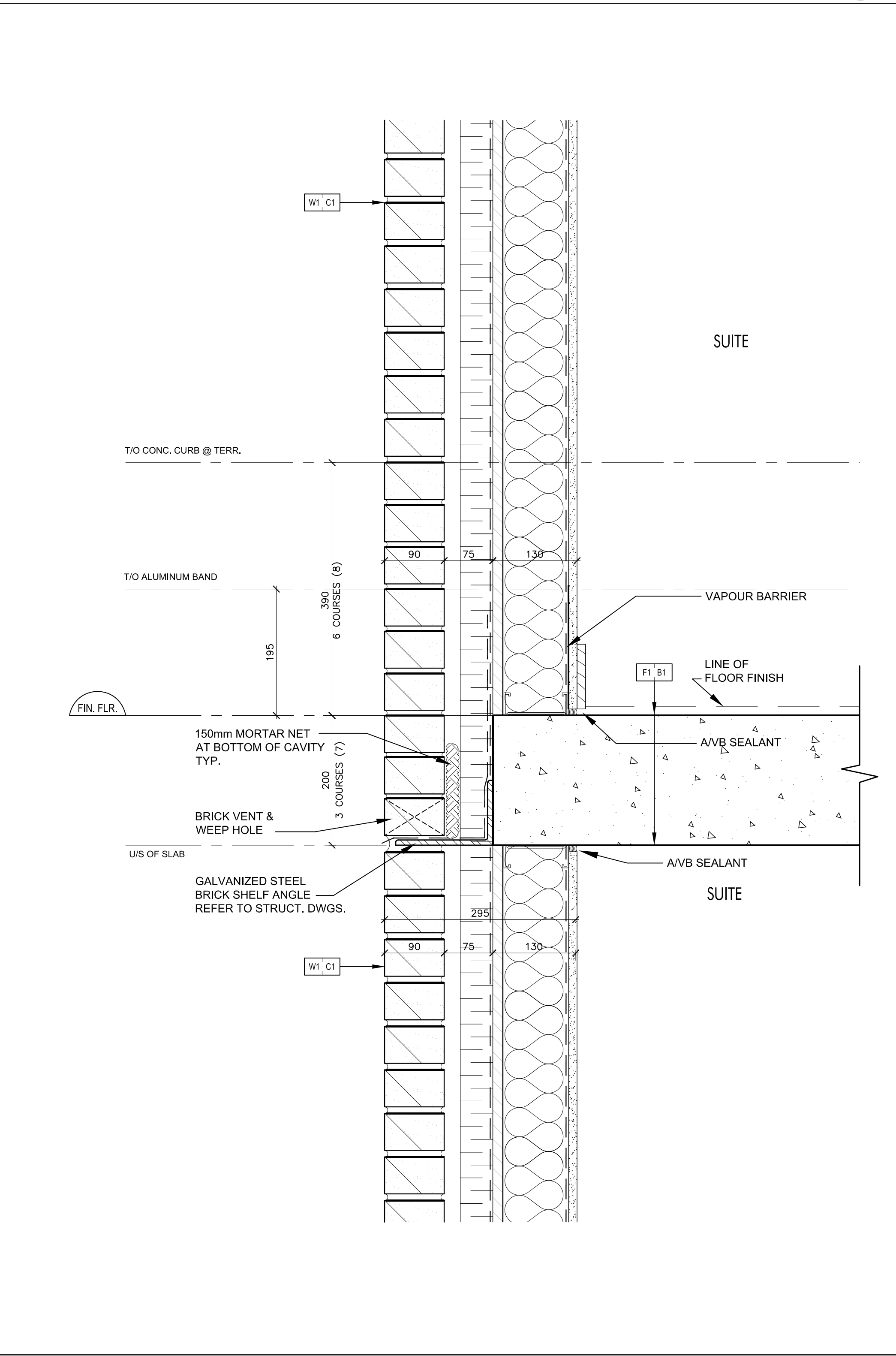
Typical Brick Coursing @ Concrete Slab 1 SCALE: 1:5 A7-12
