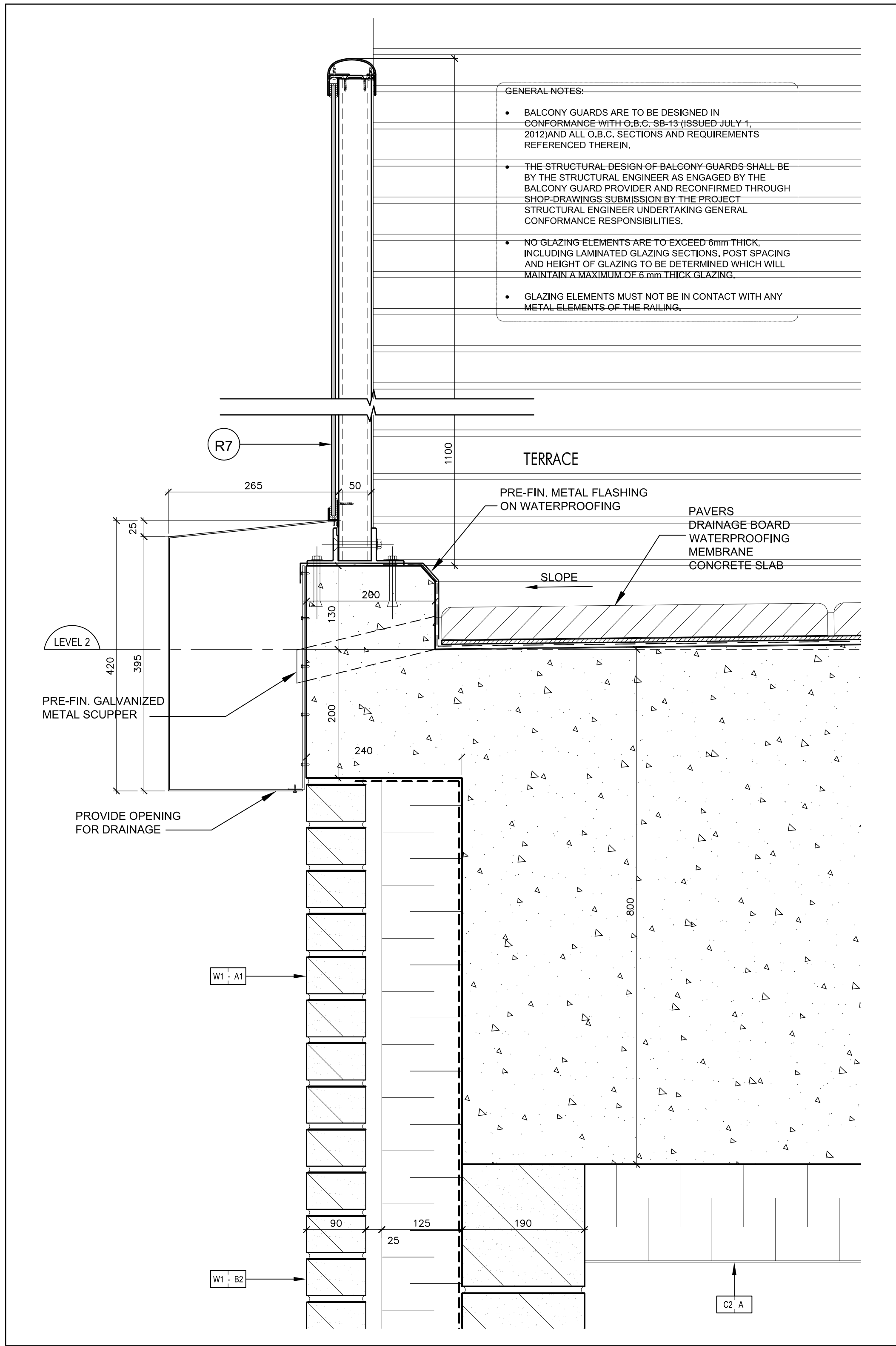
Railing & Pre-Fin. Aluminum Band @ Level 2 Terrace 12 SCALE: 1:5 A7-12
