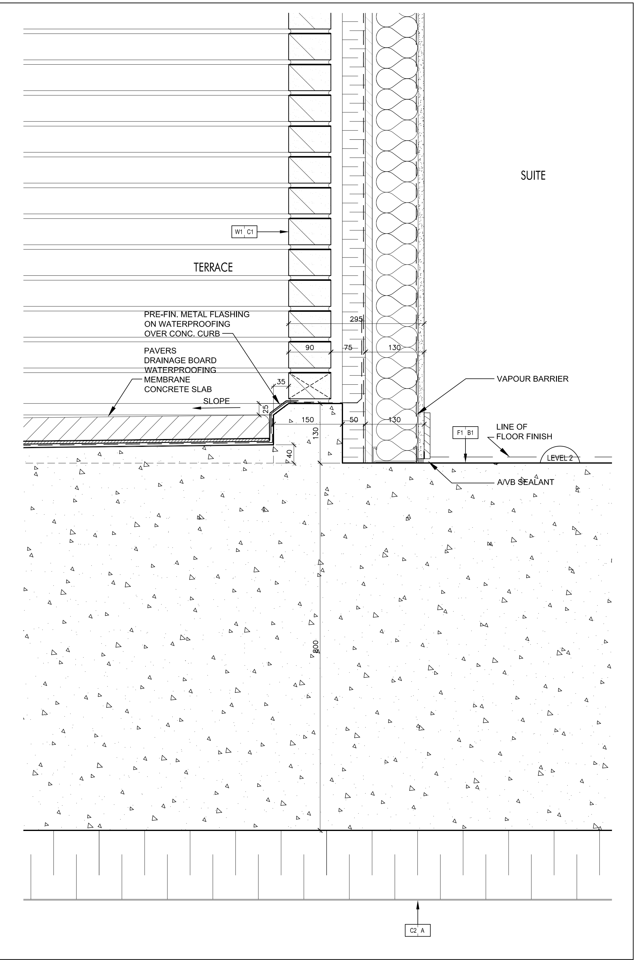
Concrete Curb @ Level 2 Terrace @ Brick Veneer Wall 9 SCALE: 1:5 A7-12
