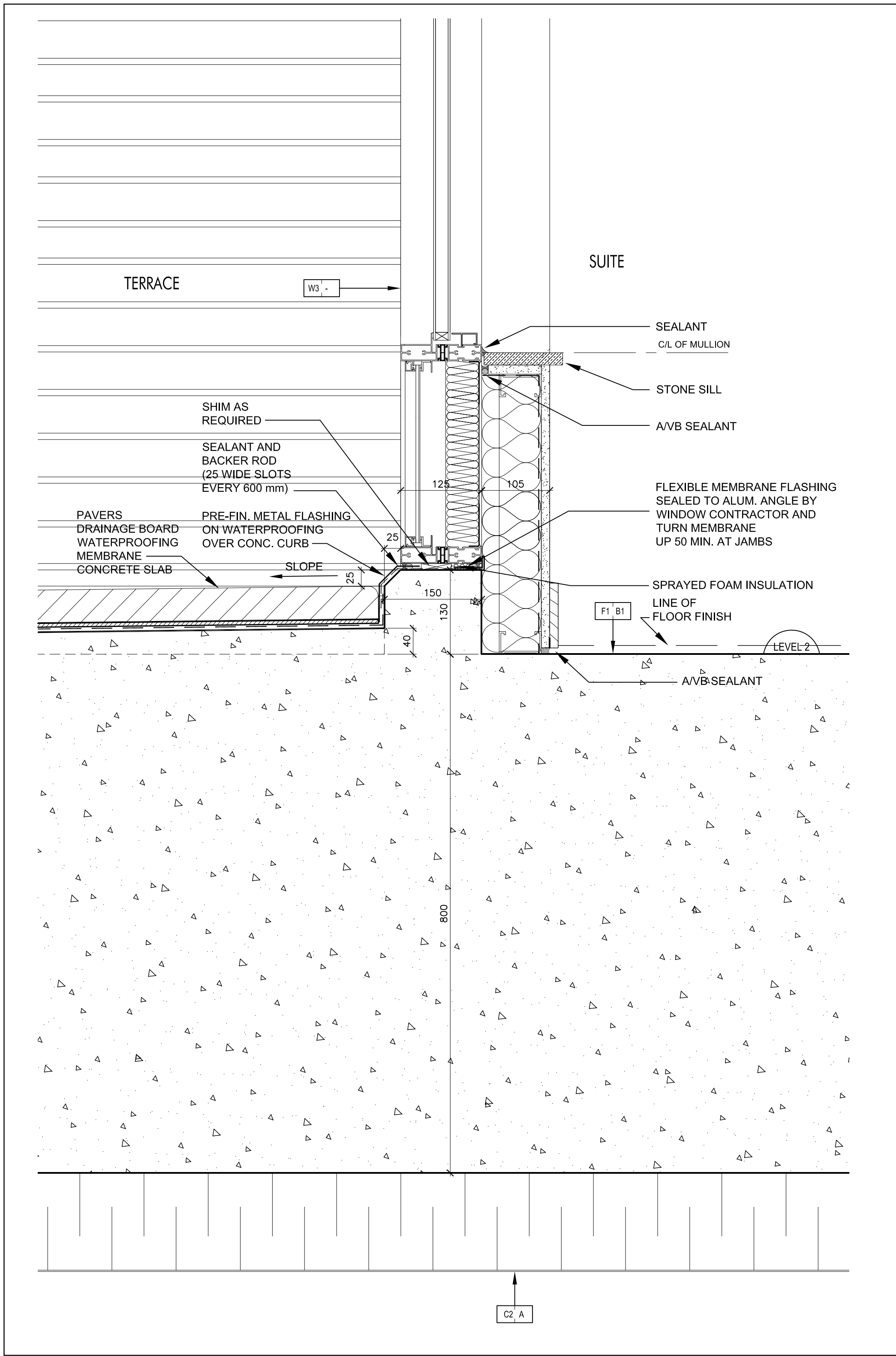
Concrete Curb @ Level 2 Terrace @ Window Wall 11 SCALE: 1:5 A7-12
