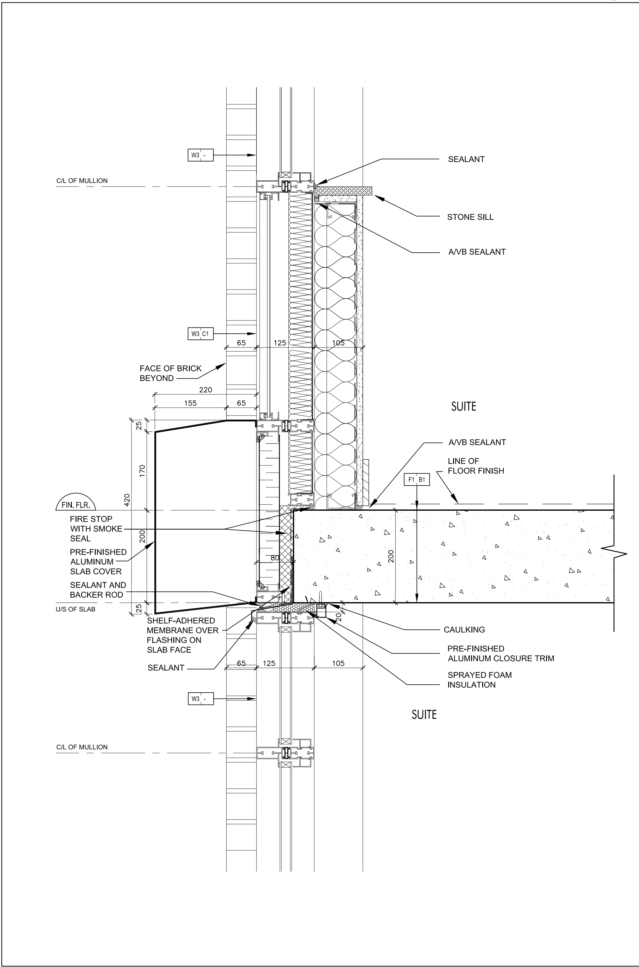
Pre-Finished Aluminum Slab Cover @ Window Wall 4 SCALE: 1:5 A7-12
