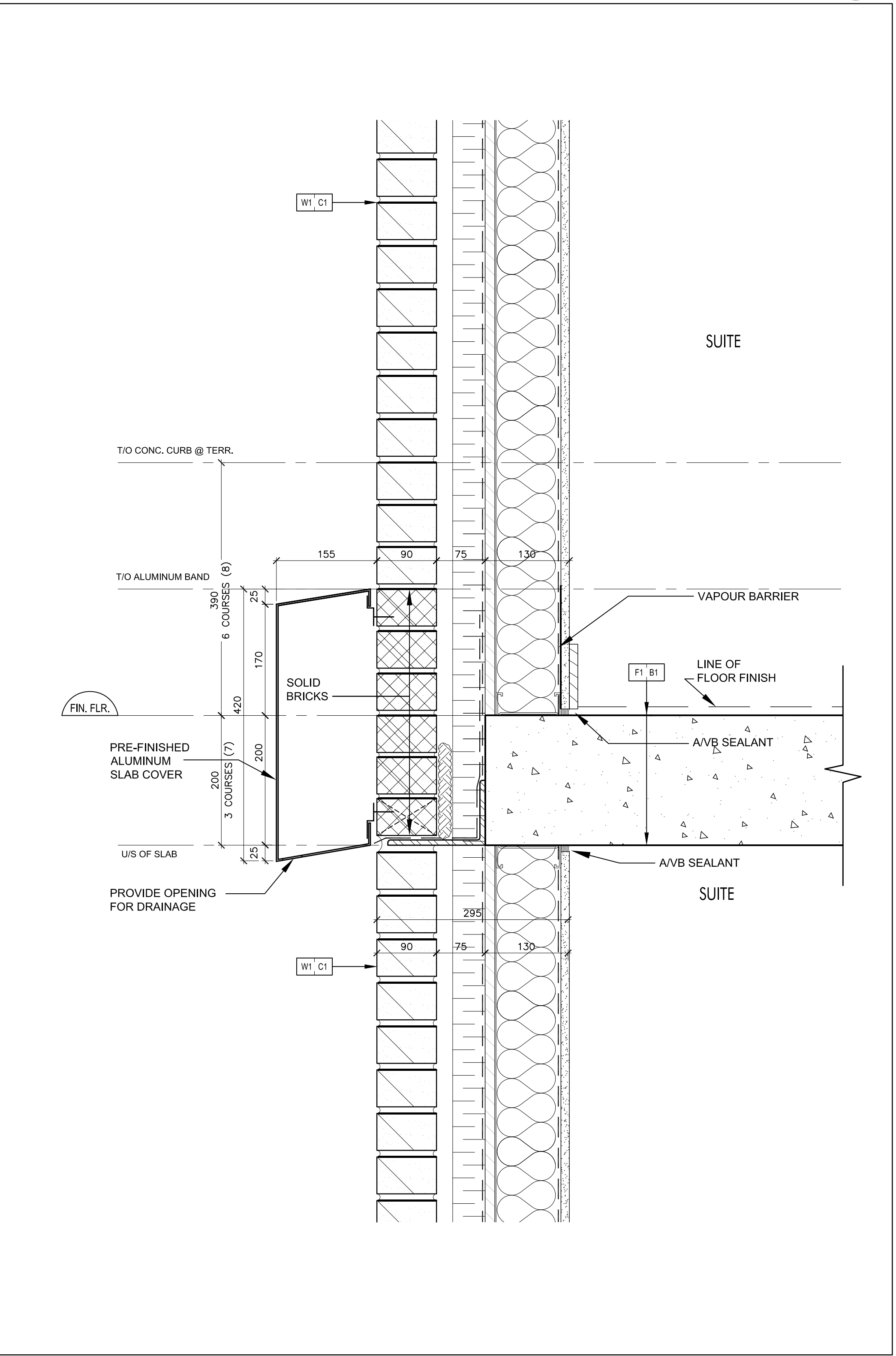
Pre-Finished Aluminum Slab Cover @ Brick Wall 2 SCALE: 1:5 A7-12
