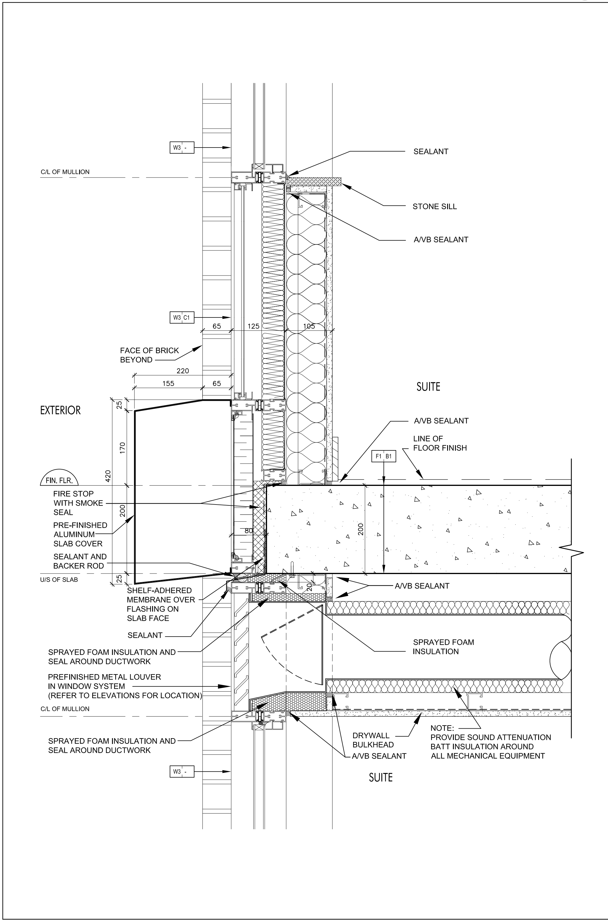
Pre-Finished Aluminum Slab Cover @ Window Wall 5 SCALE: 1:5 A7-12
