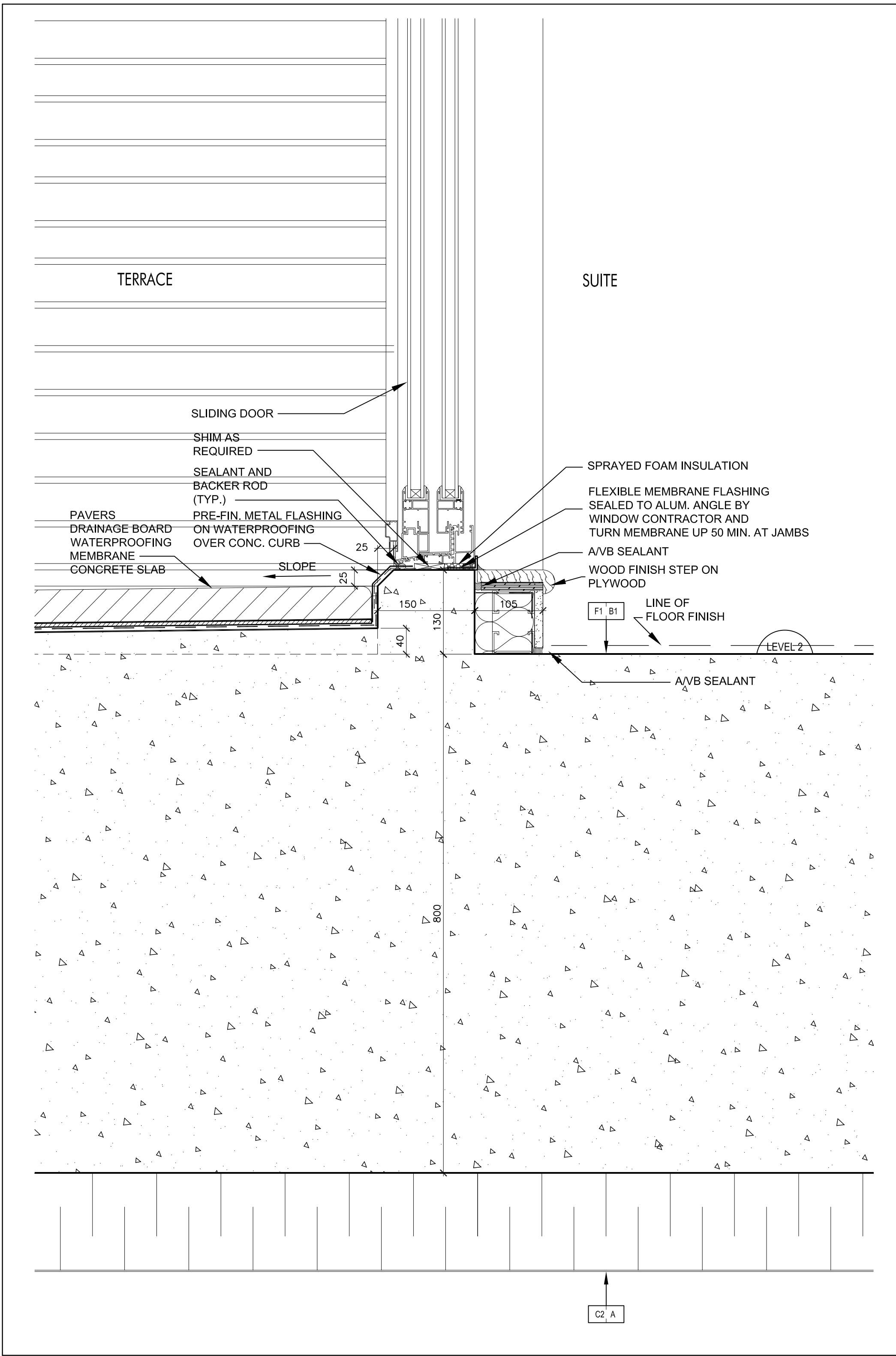
Concrete Curb @ Level 2 Terrace @ Sliding Door 10 SCALE: 1:5 A7-12
