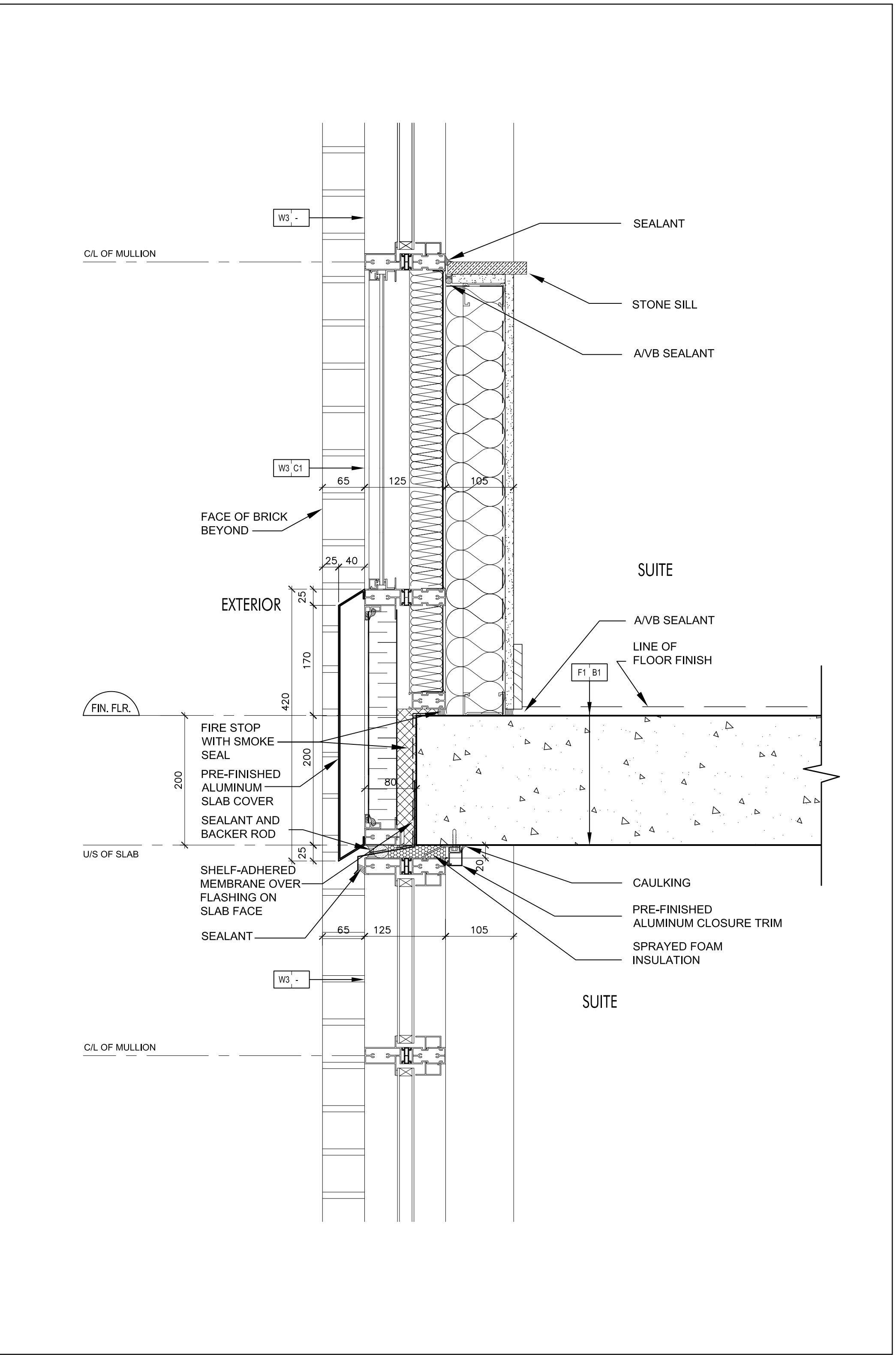
Pre-Finished Aluminum Slab Cover @ Window Wall 8 SCALE: 1:5 A7-12
