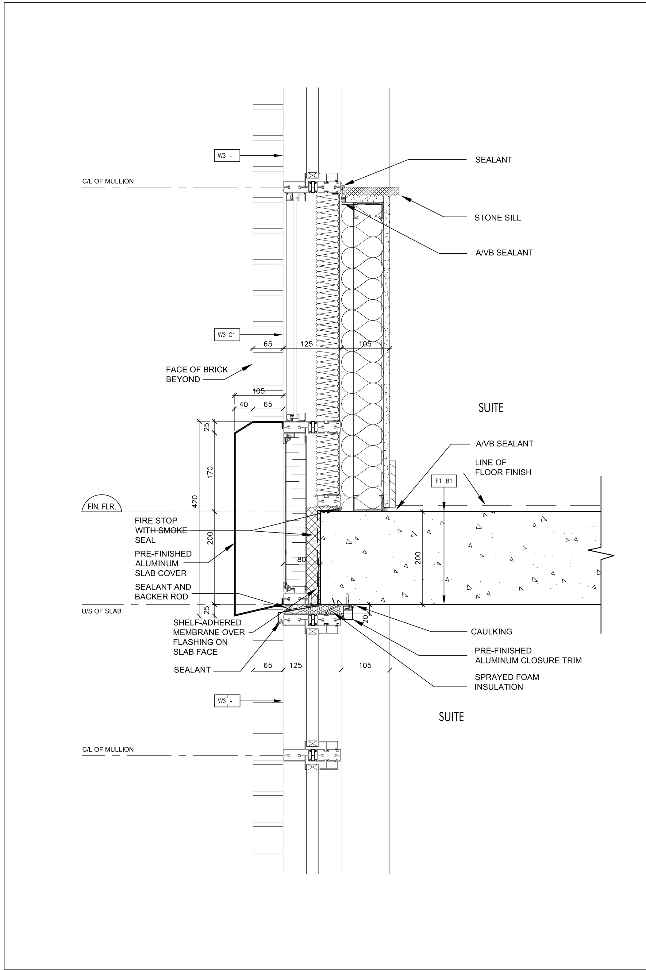
Pre-Finished Aluminum Slab Cover @ Window Wall 6 SCALE: 1:5 A7-12
