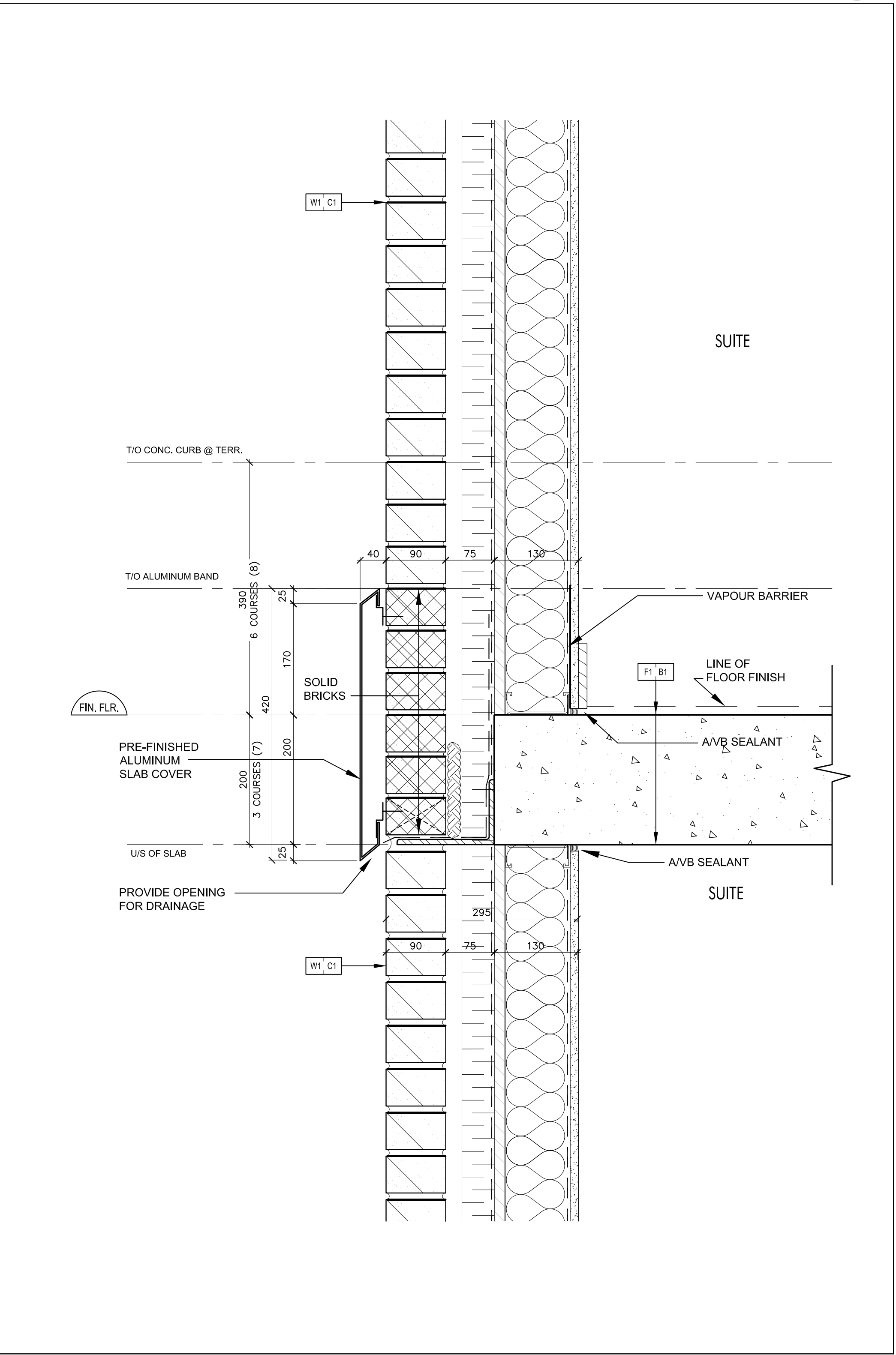
Pre-Finished Aluminum Slab Cover @ Brick Wall 3 SCALE: 1:5 A7-12
