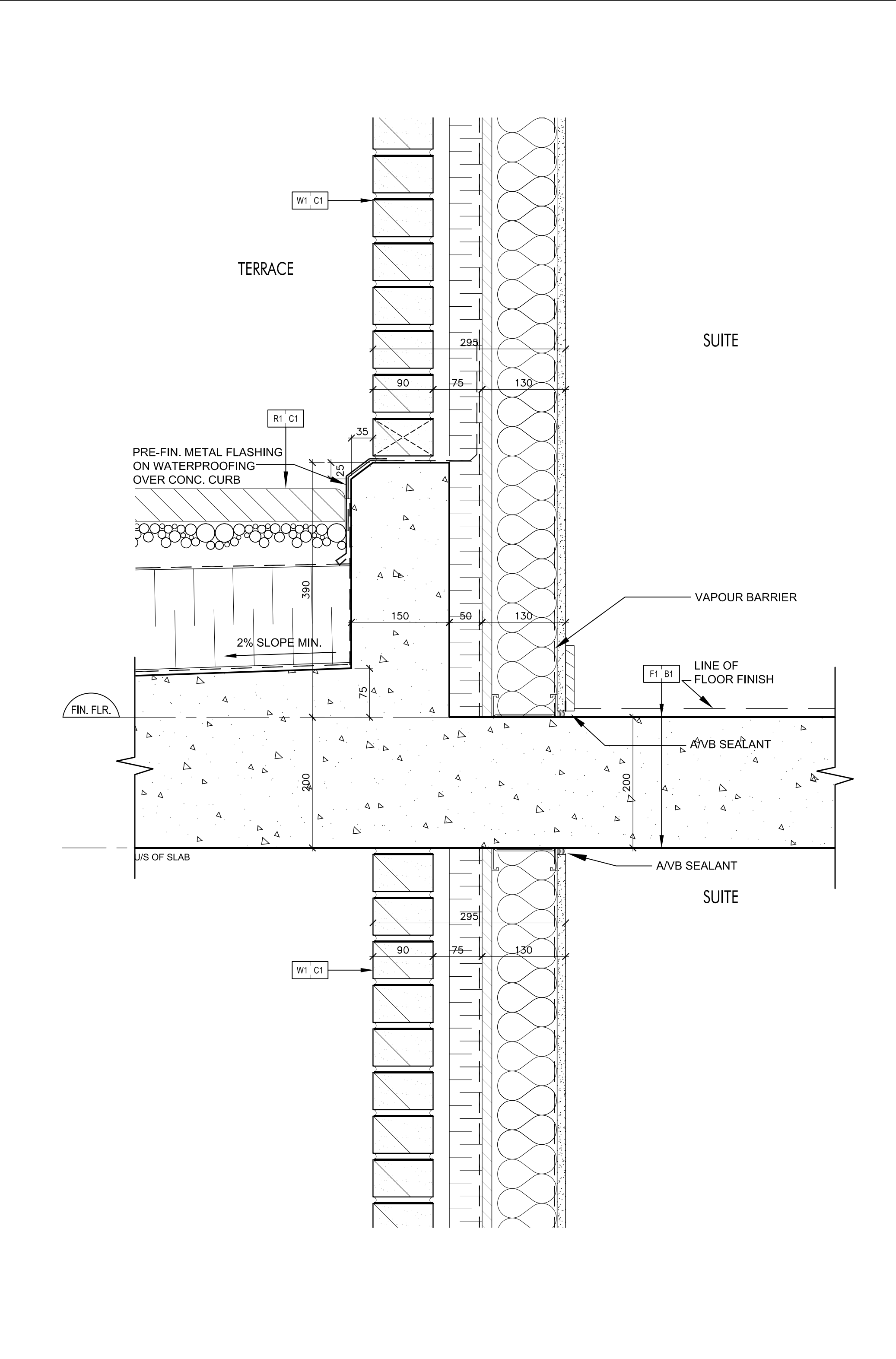
Brick Wall @ Terrace 3 SCALE 1:5 A7-11
