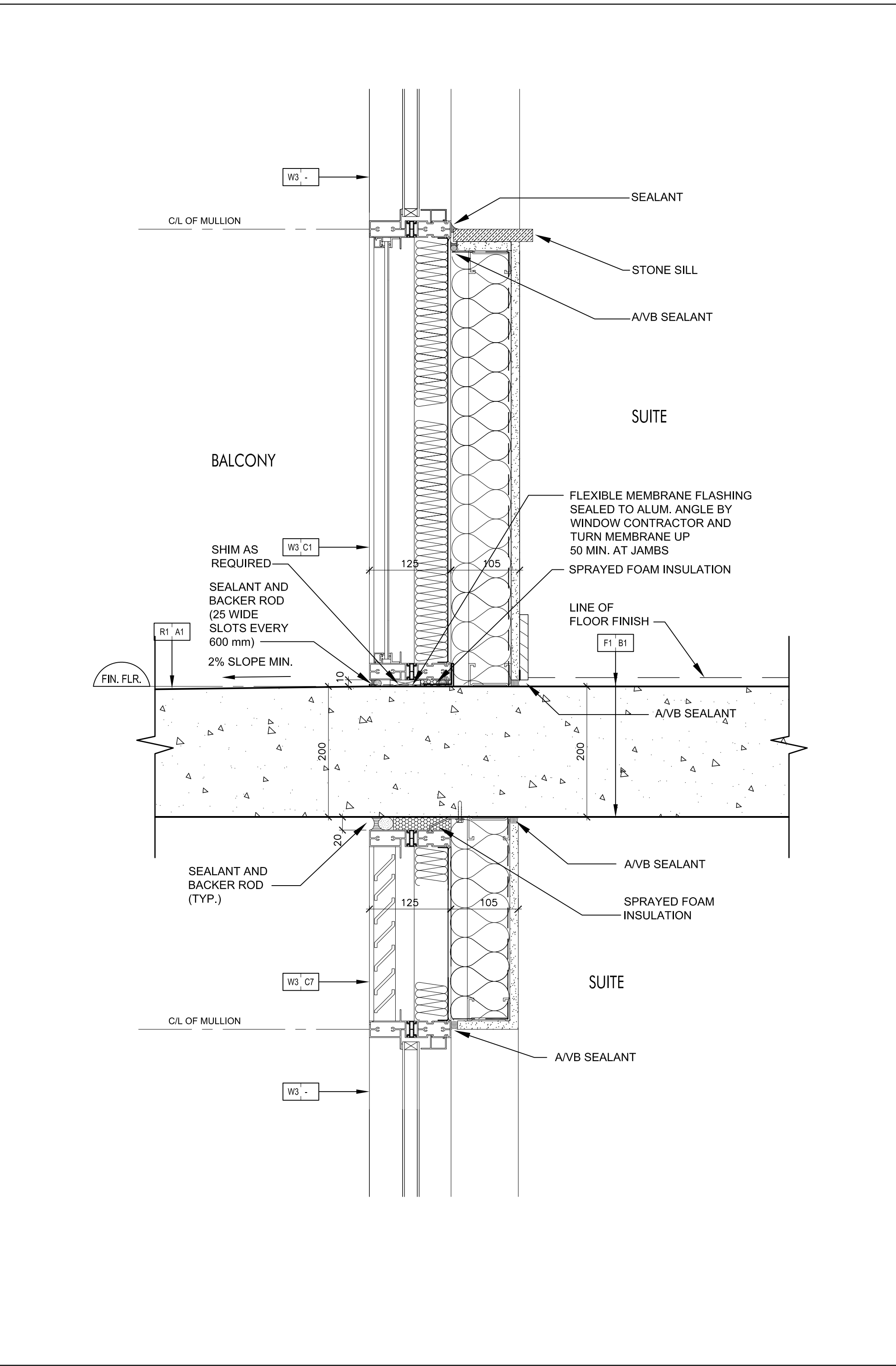
Window Wall @ Balcony 9 SCALE 1:5 A7-11
