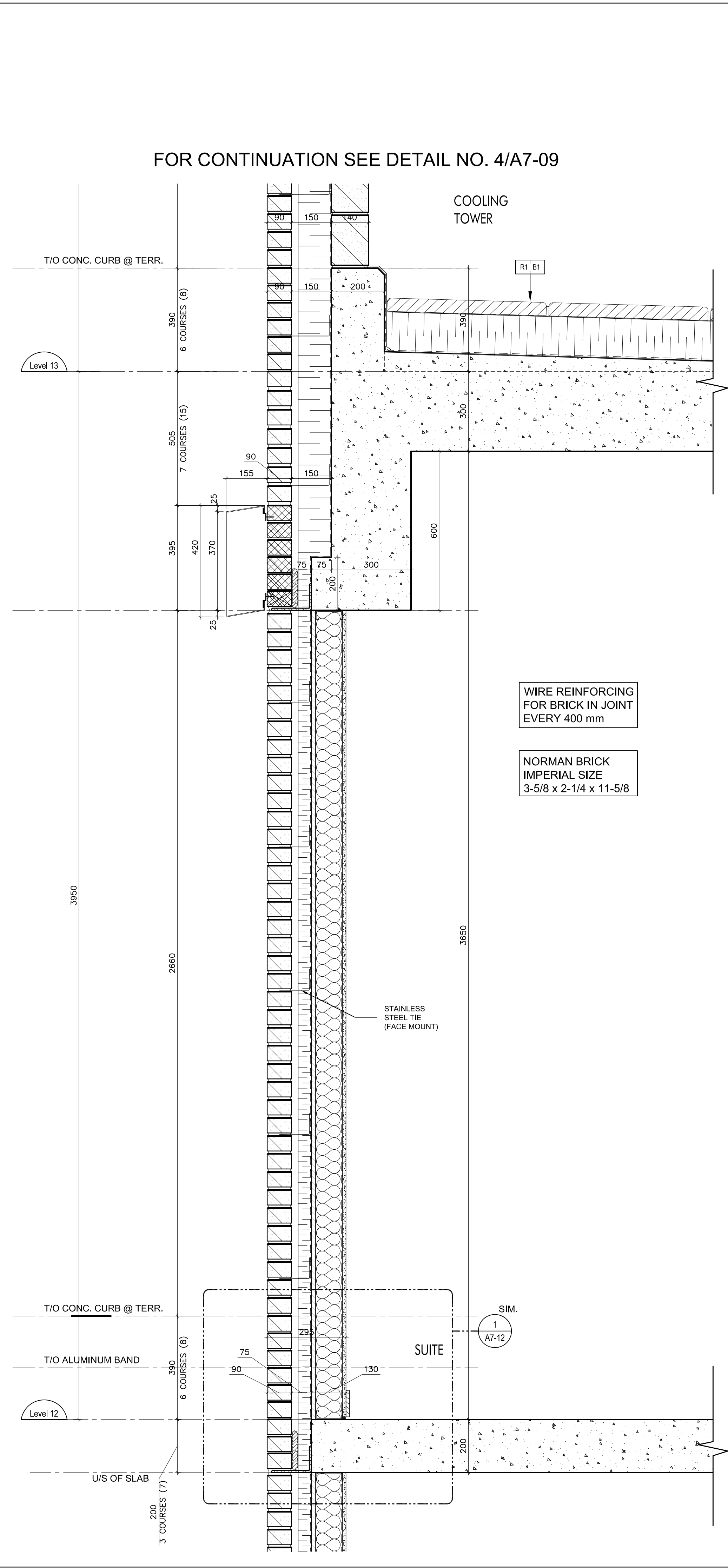
Brick Coursing @ Masonry Wall - Floor Height 3950 SCALE 1:10 3 A7-10
