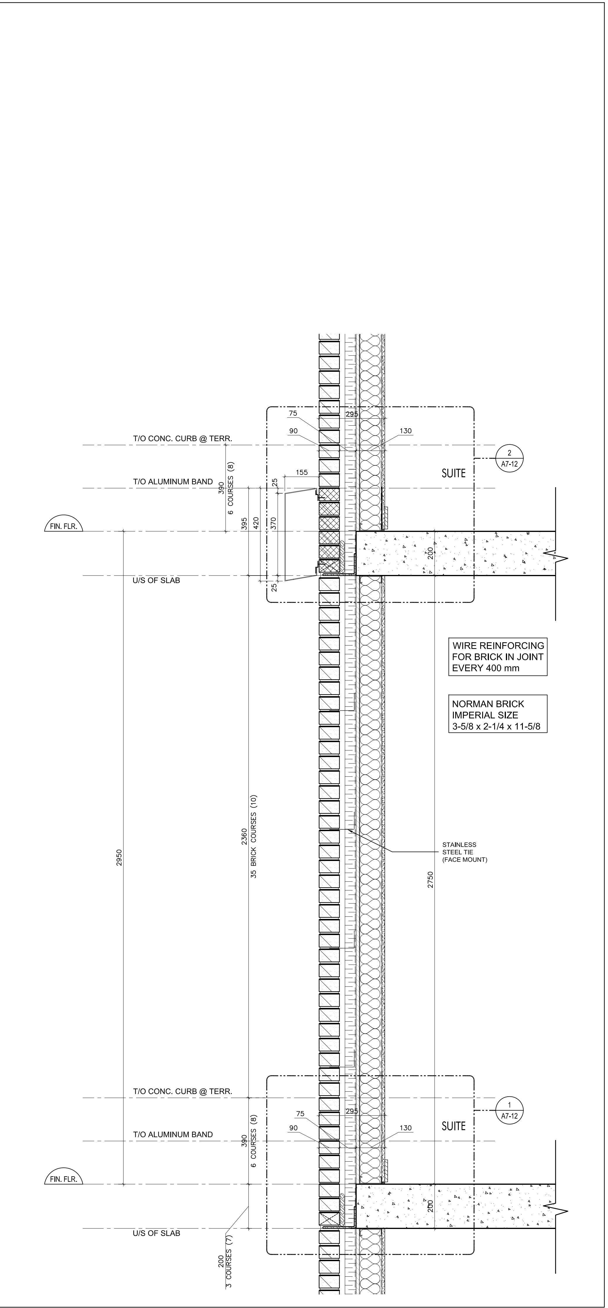
Brick Coursing @ Masonry Wall - Floor Height 2950 SCALE 1:10 1 A7-10
