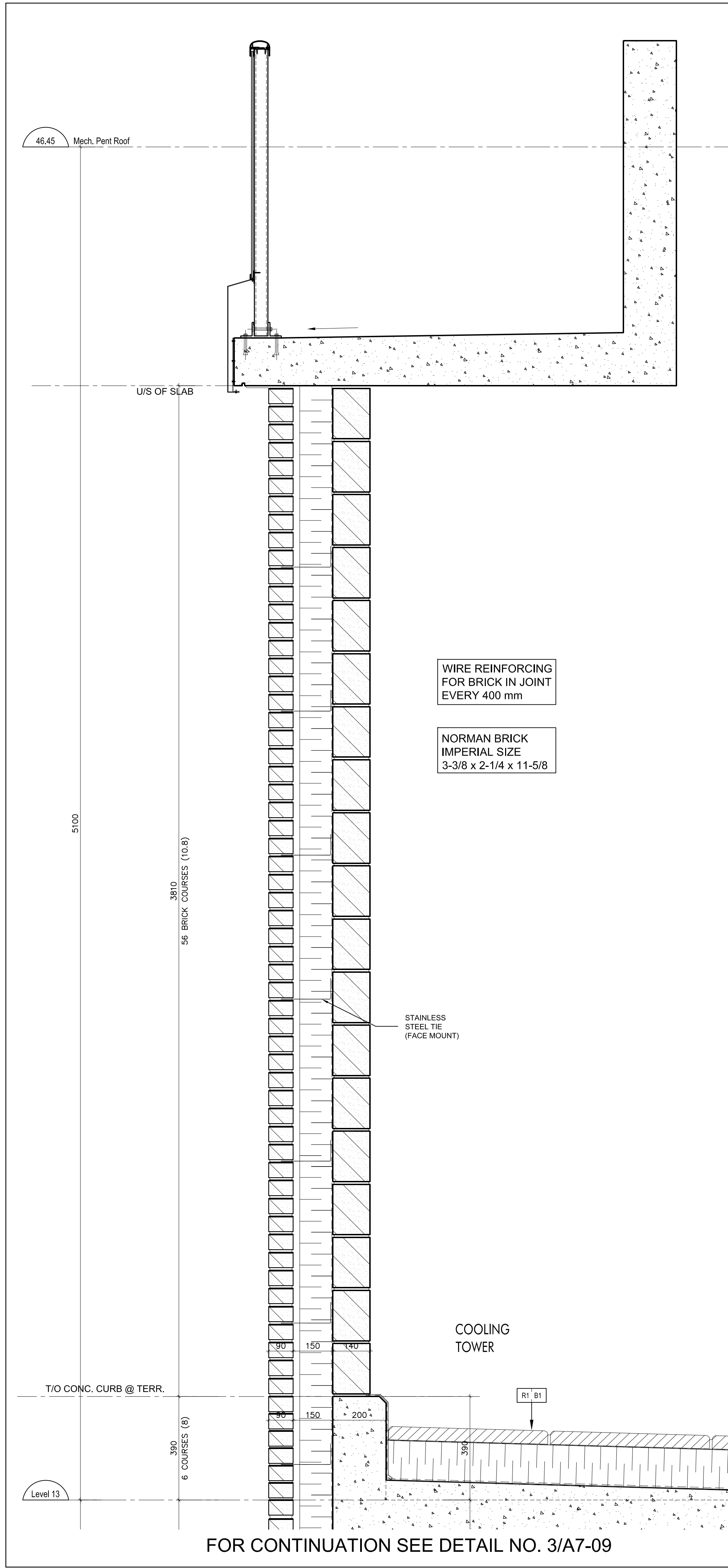
Brick Coursing @ Masonry Wall - Floor Height 5100 SCALE 1:10 4 A7-10
