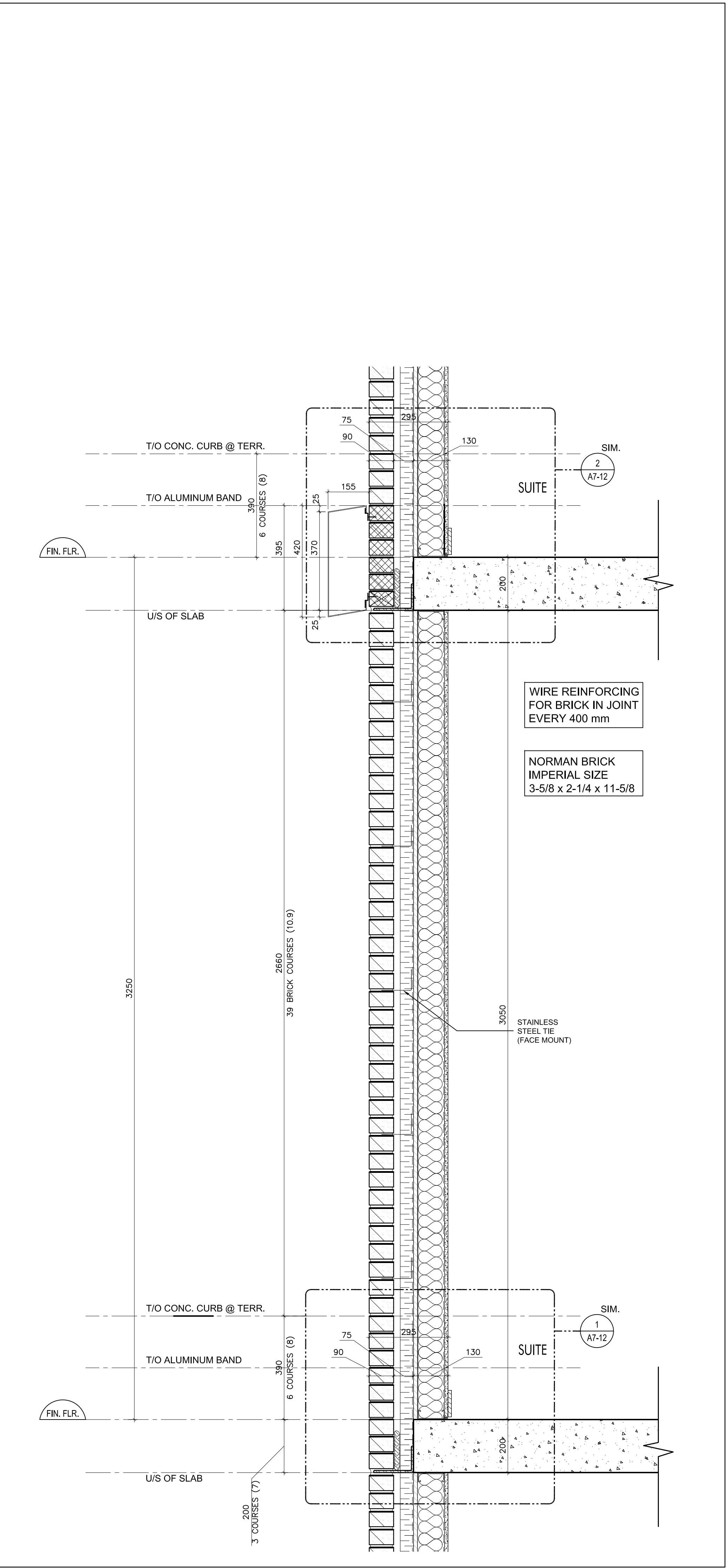
Brick Coursing @ Masonry Wall - Floor Height 3250 SCALE 1:10 2 A7-10
