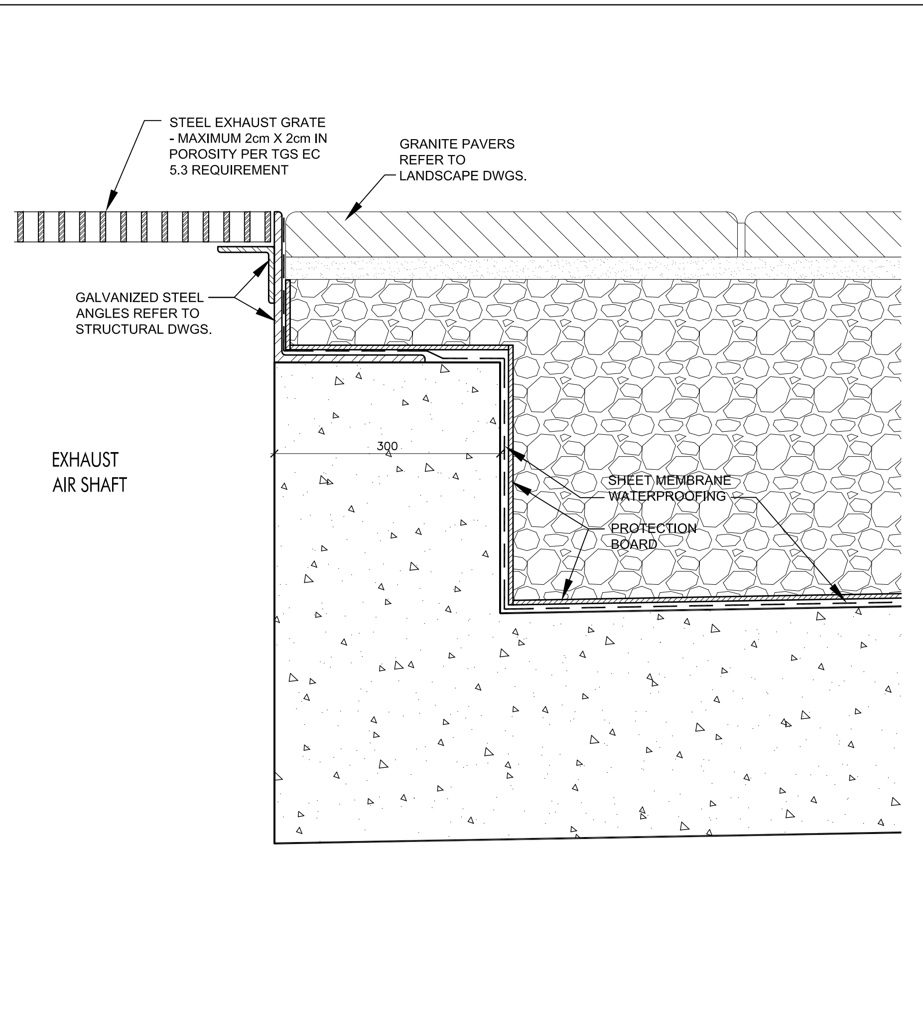
Section thru Exhaust Air Shaft Steel Grate @ Level 1 3 SCALE 1:5 A7-08
