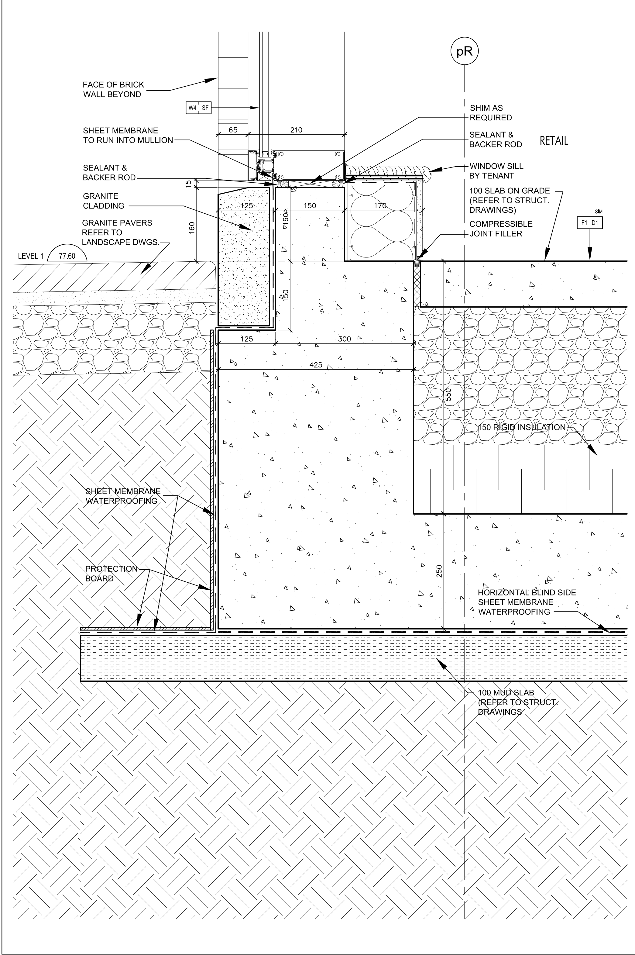
Curtain Wall Sill @ Retail 7 SCALE 1:5 A7-08
