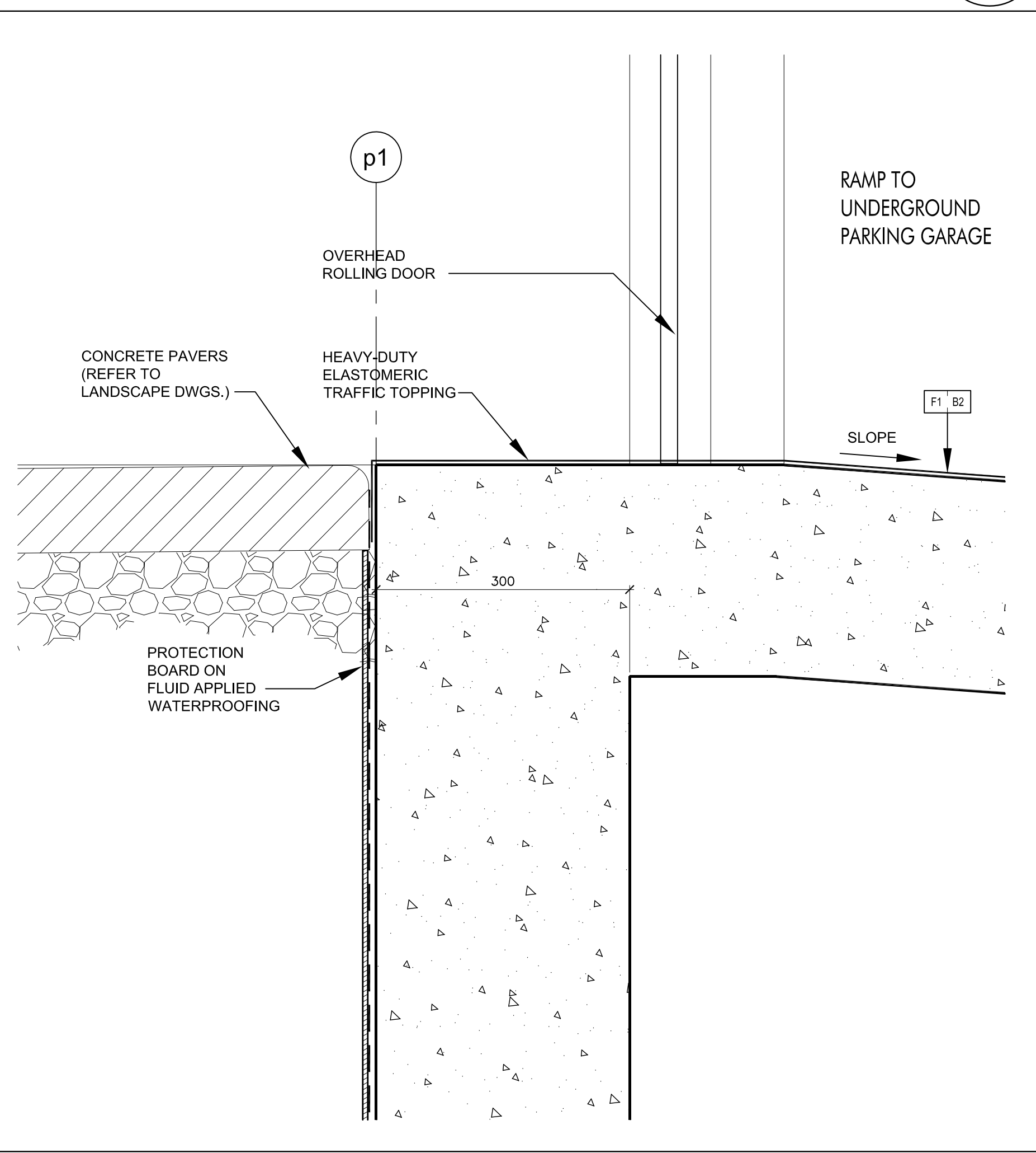
Entrance to Residential Parking 1 SCALE 1:5 A7-08
