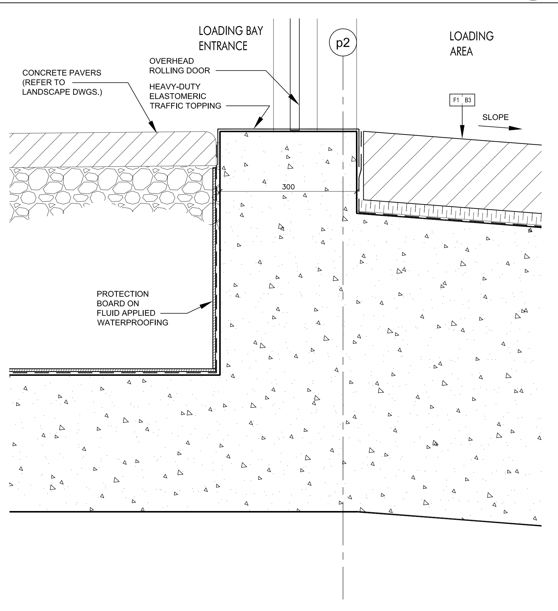
Entrance & O/H Door @ Loading Area 2 SCALE 1:5 A7-08
