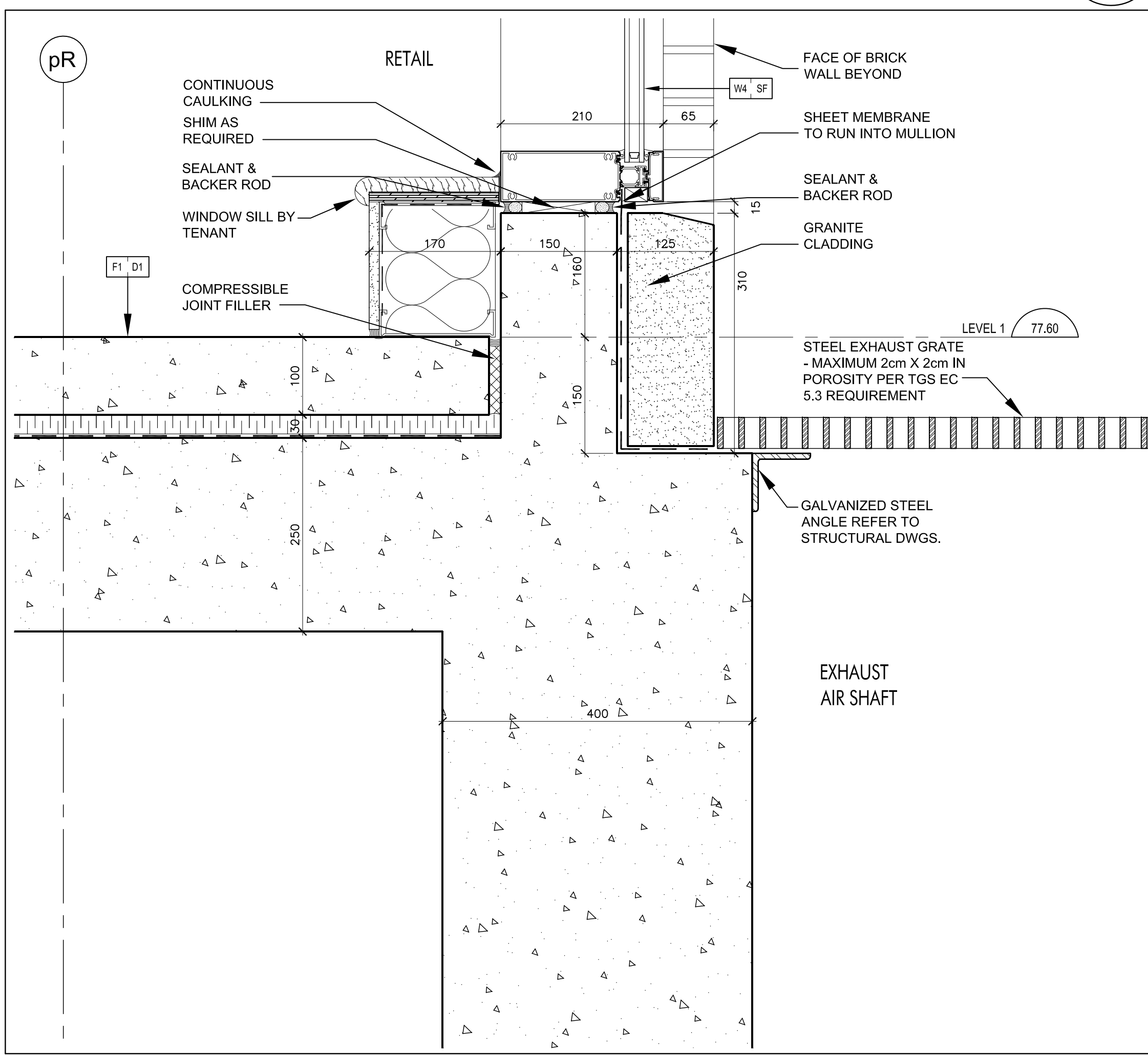
Curtain Wall Sill @ Retail & Steel Grate 4 SCALE 1:5 A7-08
