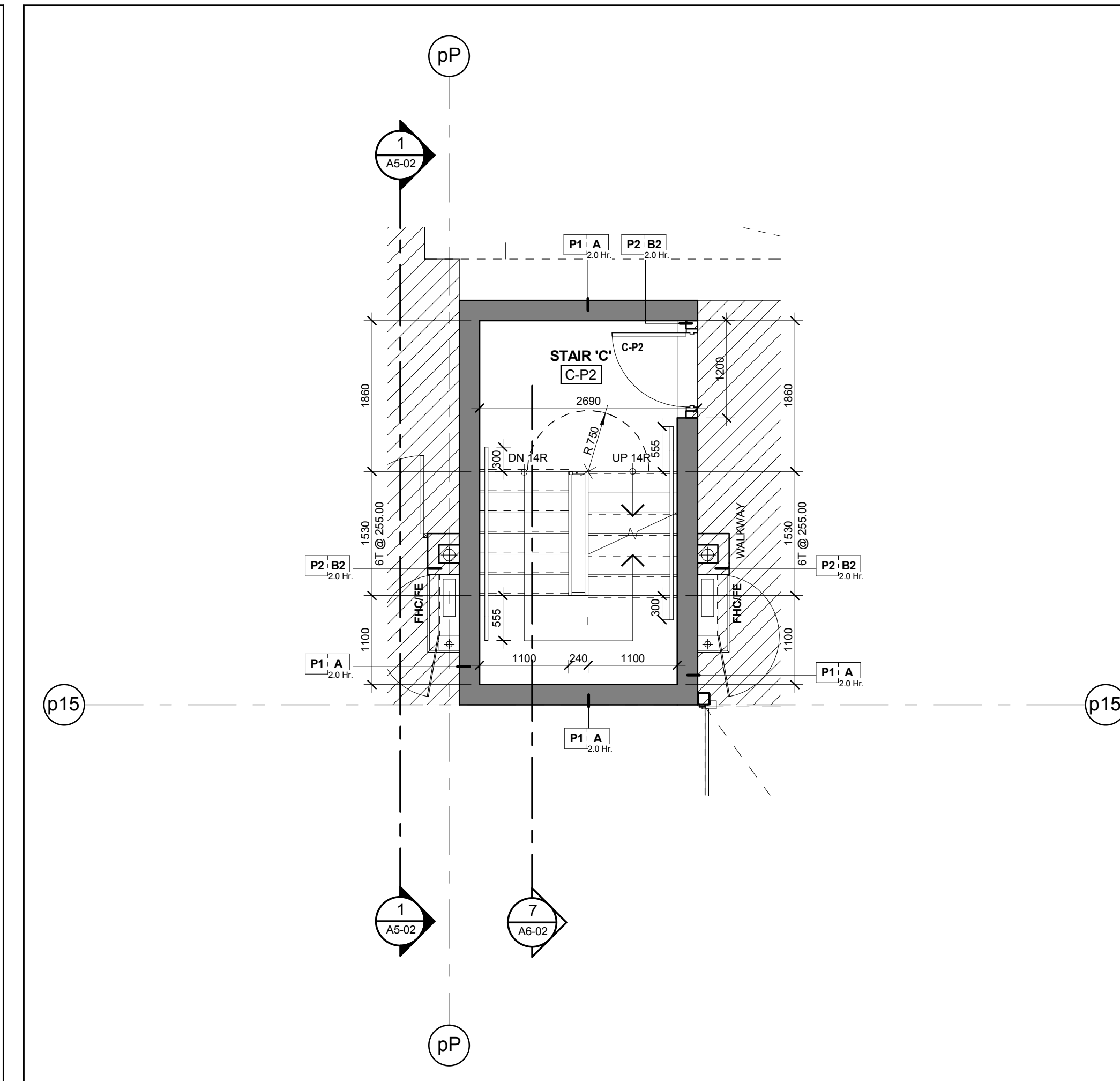
Stair 'C' - Stair Plan - Level P2 Scale: 1 : 50 A6-02
