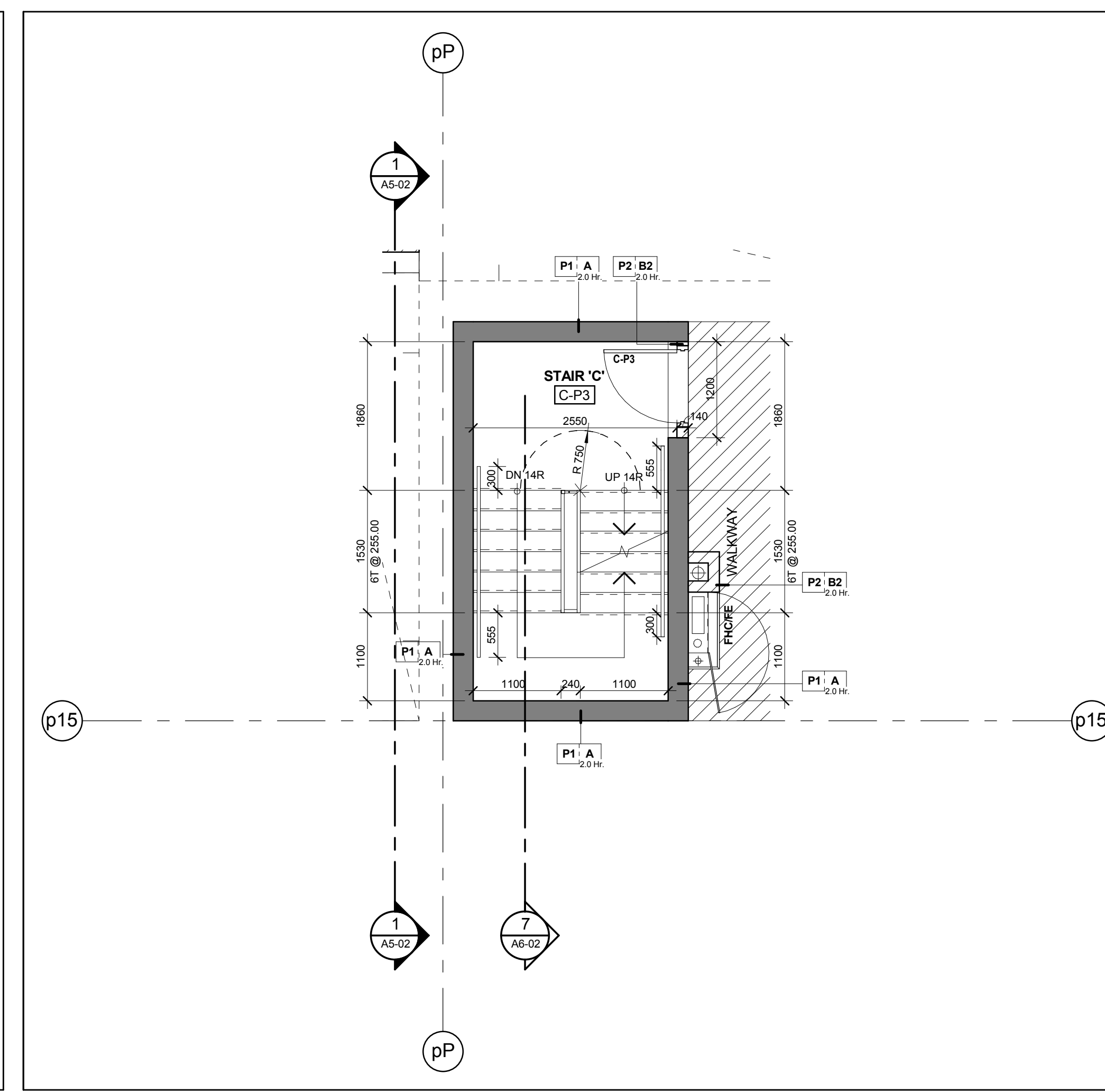
Stair 'C' - Stair Plan - Level P3 Scale: 1 : 50 A6-02
