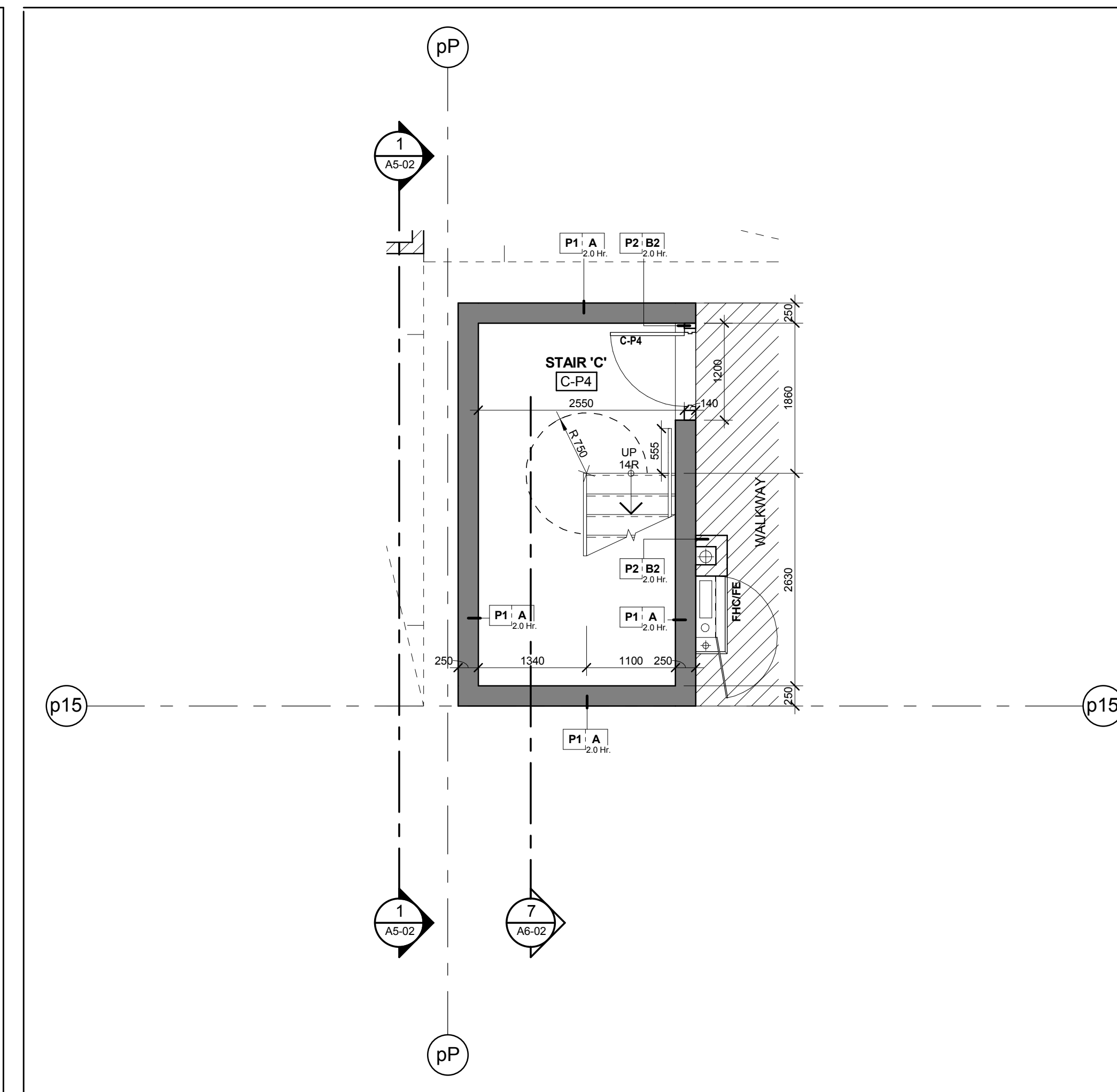
Stair 'C' - Stair Plan - Level P4 Scale: 1 : 50 A6-02
