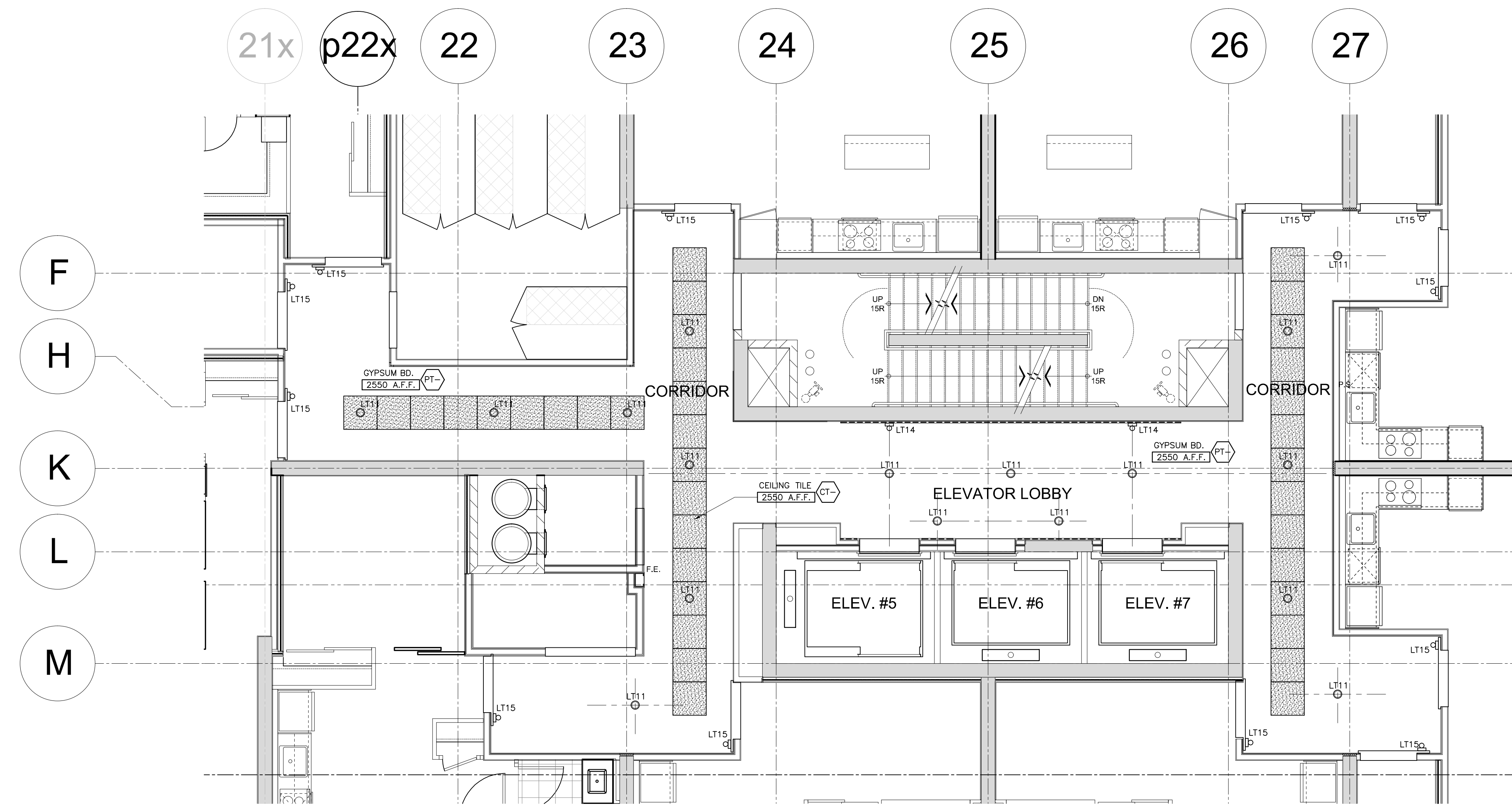
4 8th FLOOR CORRIDOR RCP (BUILDING-D) ID3.5 SCALE= 1:50
