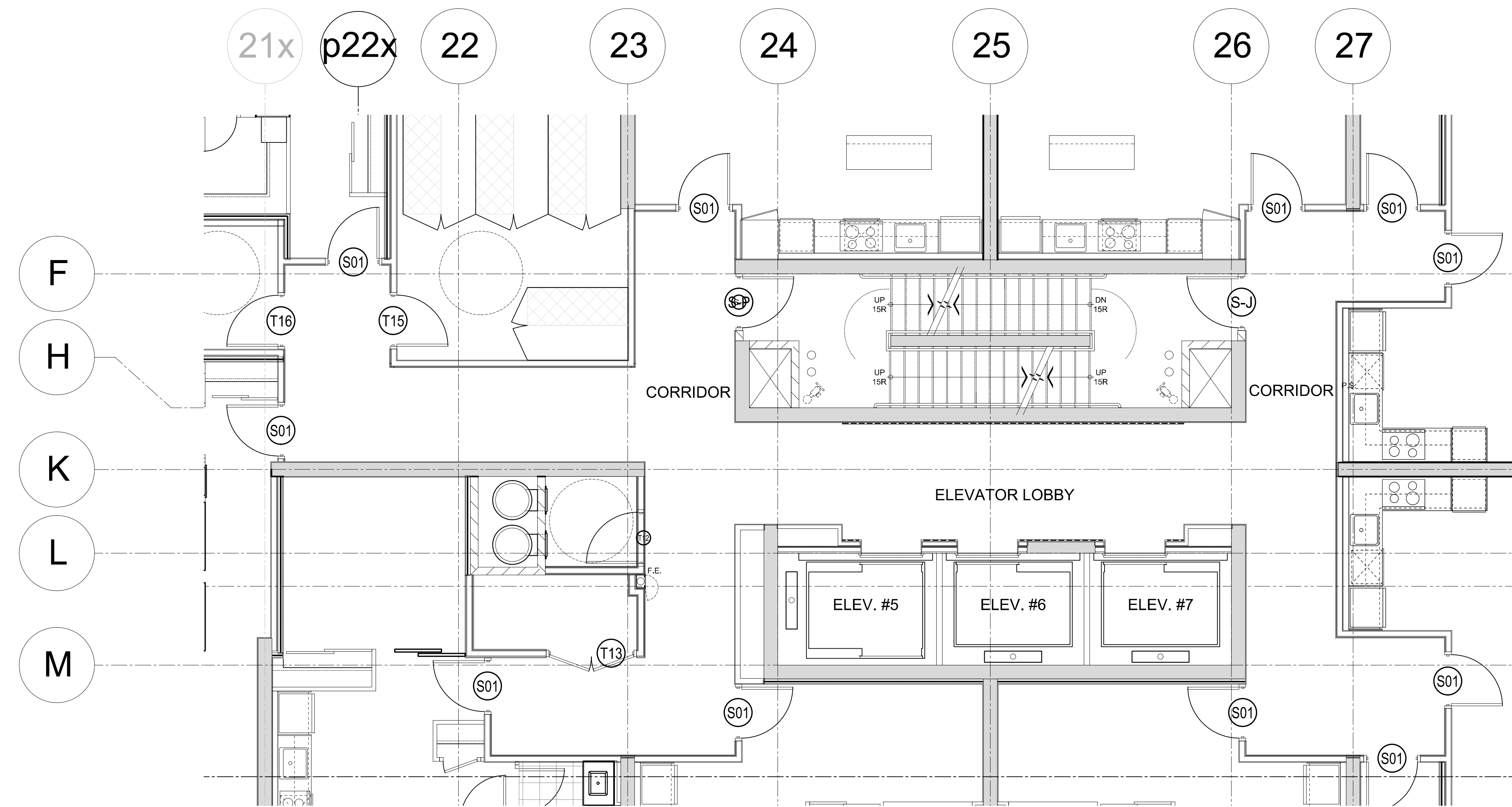
3 8th FLOOR CORRIDOR FLOOR FINISHES PLAN (BUILDING-D) ID3.5 SCALE= 1:50
