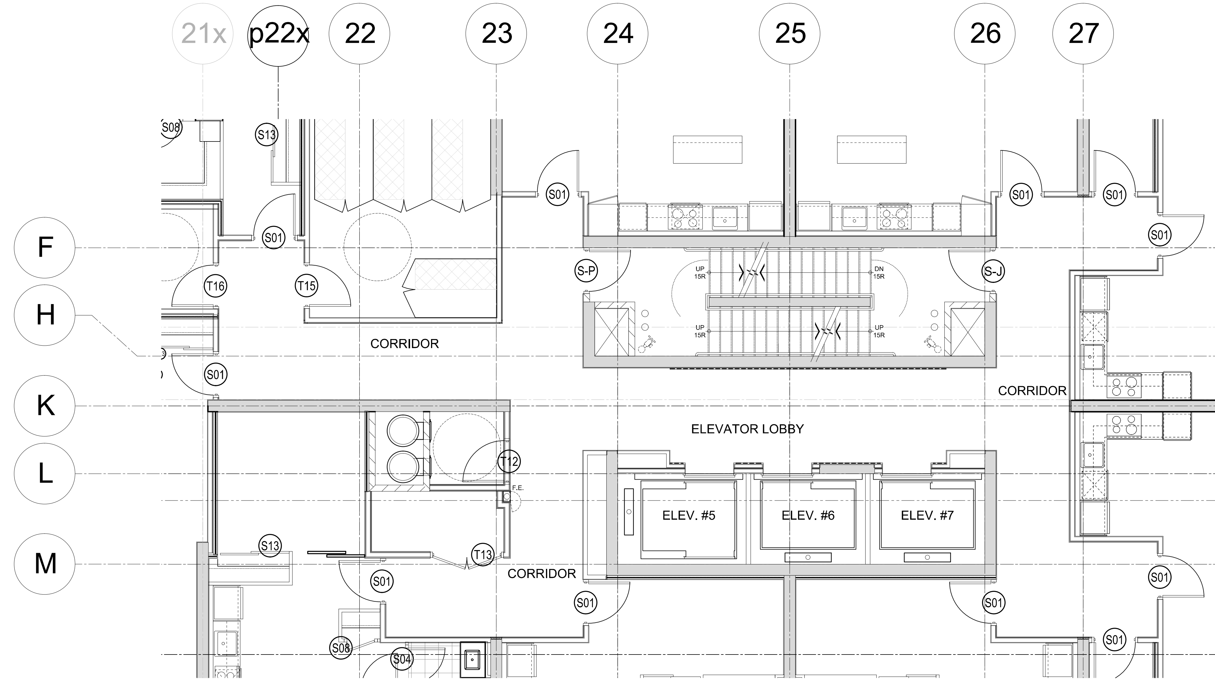
3 4-7th FLOOR CORRIDOR: FLOOR FINISHES PLAN (BUILDING-D) ID3.4 SCALE= 1:50
