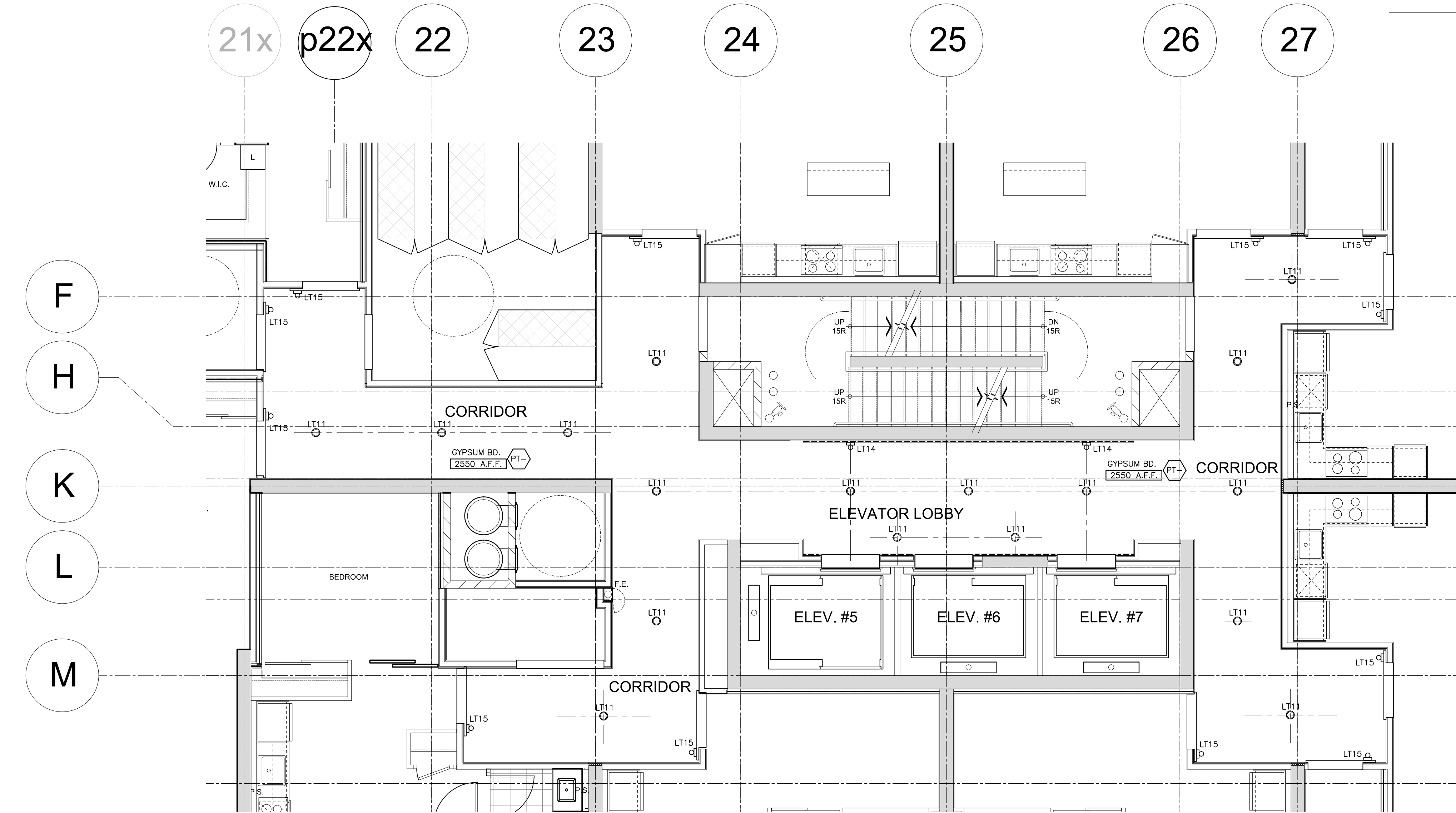
4 4-7th FLOOR CORRIDOR: RCP (BUILDING-D) ID3.4 SCALE= 1:50
