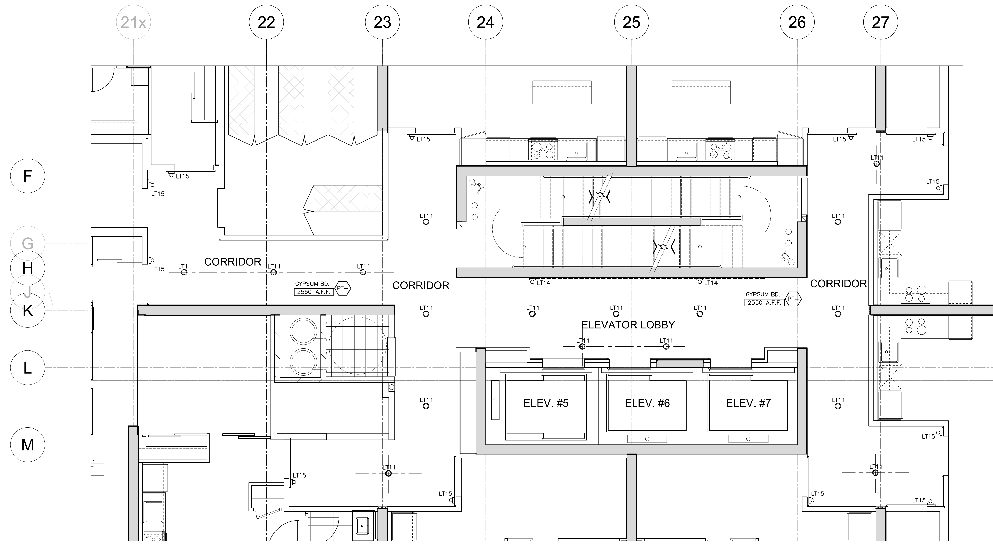
4 3rd FLOOR CORRIDOR: RCP (BUILDING-D) ID3.3 SCALE= 1:50
