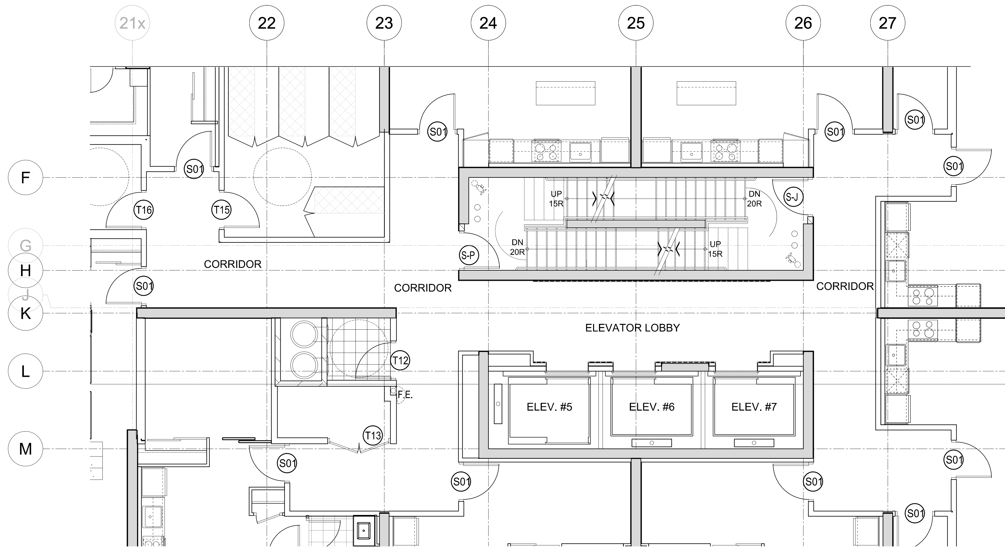
3 3rd FLOOR CORRIDOR: FLOOR FINISHES PLAN (BUILDING-D) ID3.3 SCALE= 1:50
