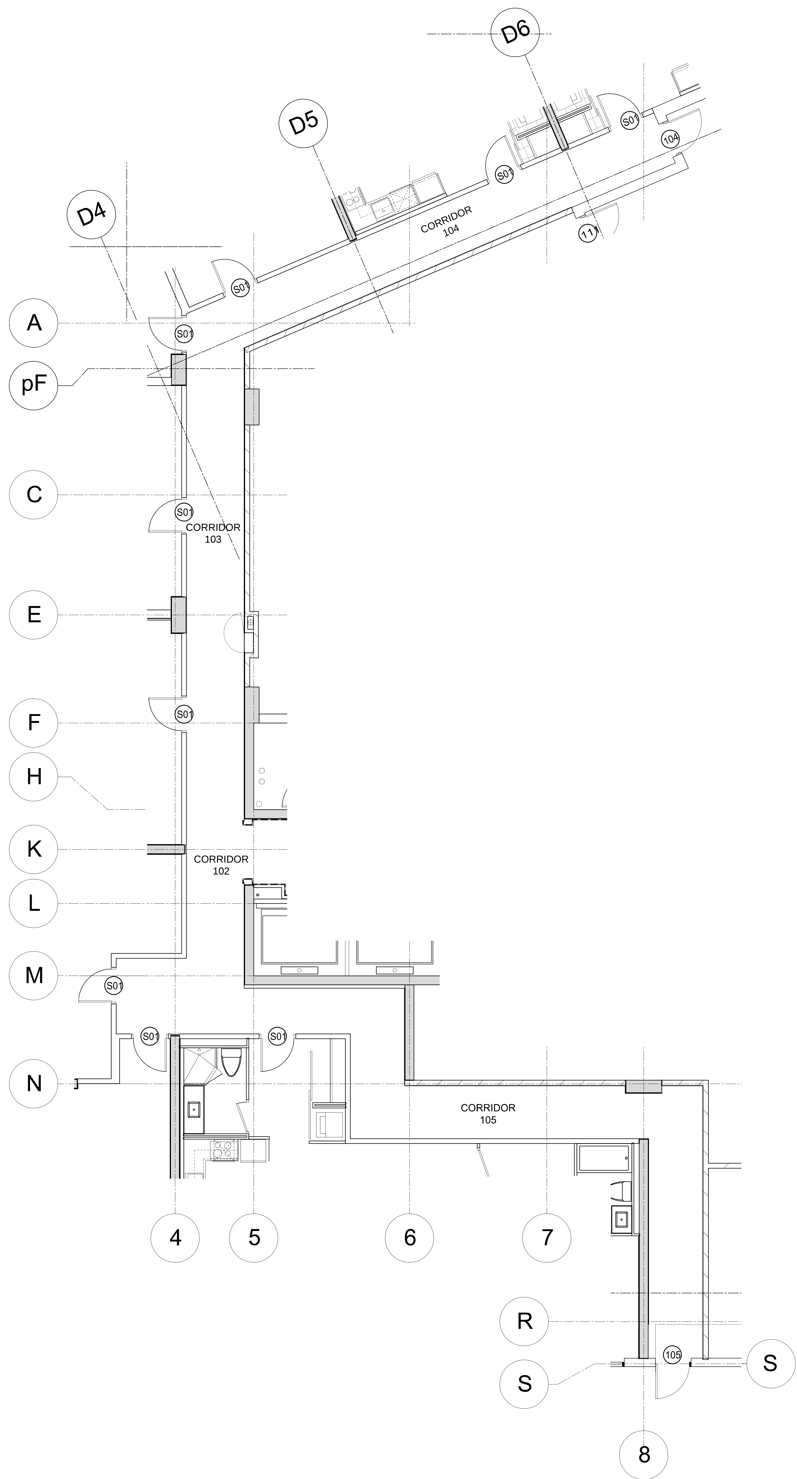
1 GROUND FLOOR CORRIDOR FLOOR FINISHES PLAN (BUILDING C) ID3.1.1 SCALE= 1:50
