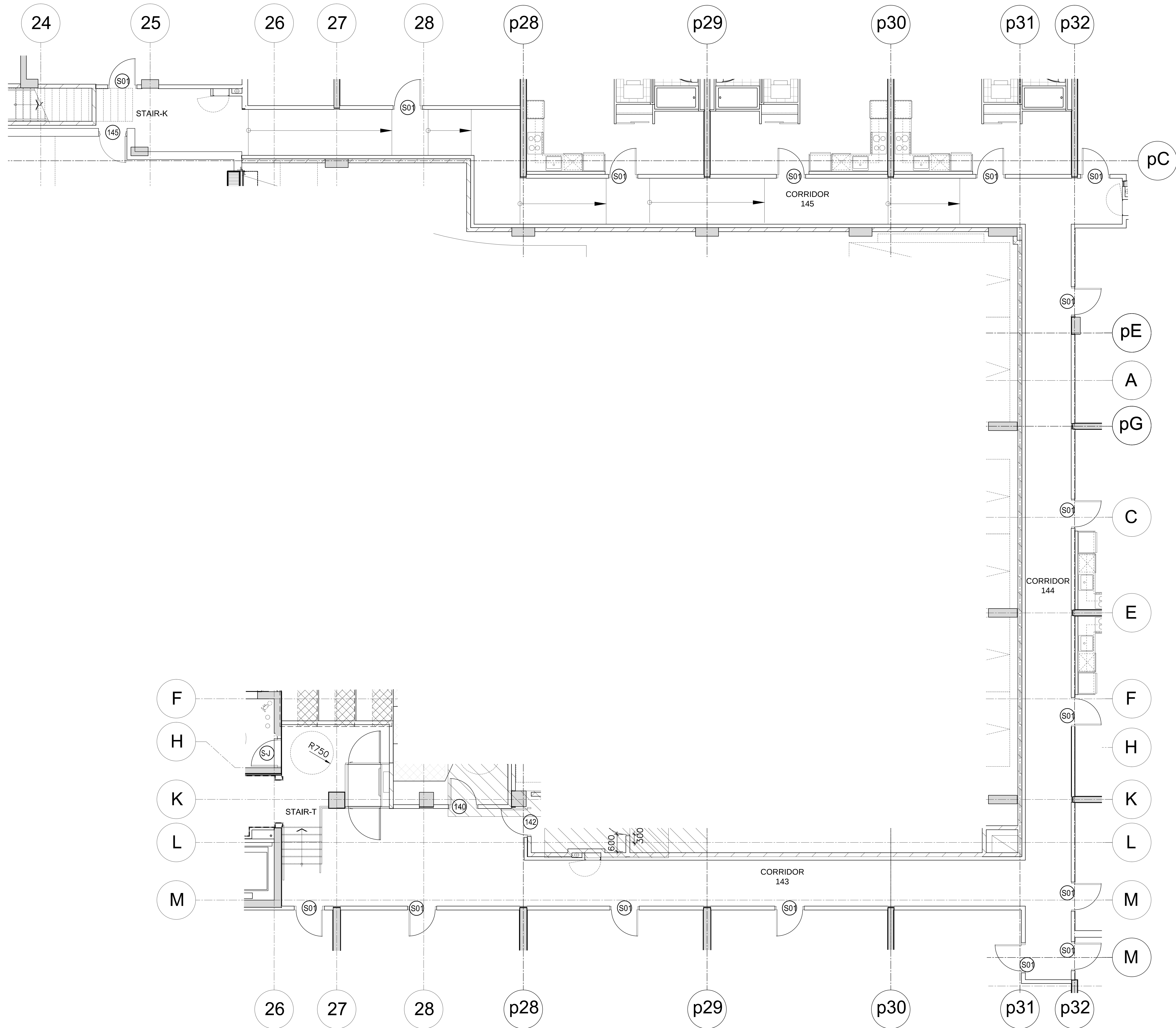
2 GROUND FLOOR CORRIDOR FLOOR FINISHES PLAN (BUILDING D) ID3.1.1 SCALE= 1:50
