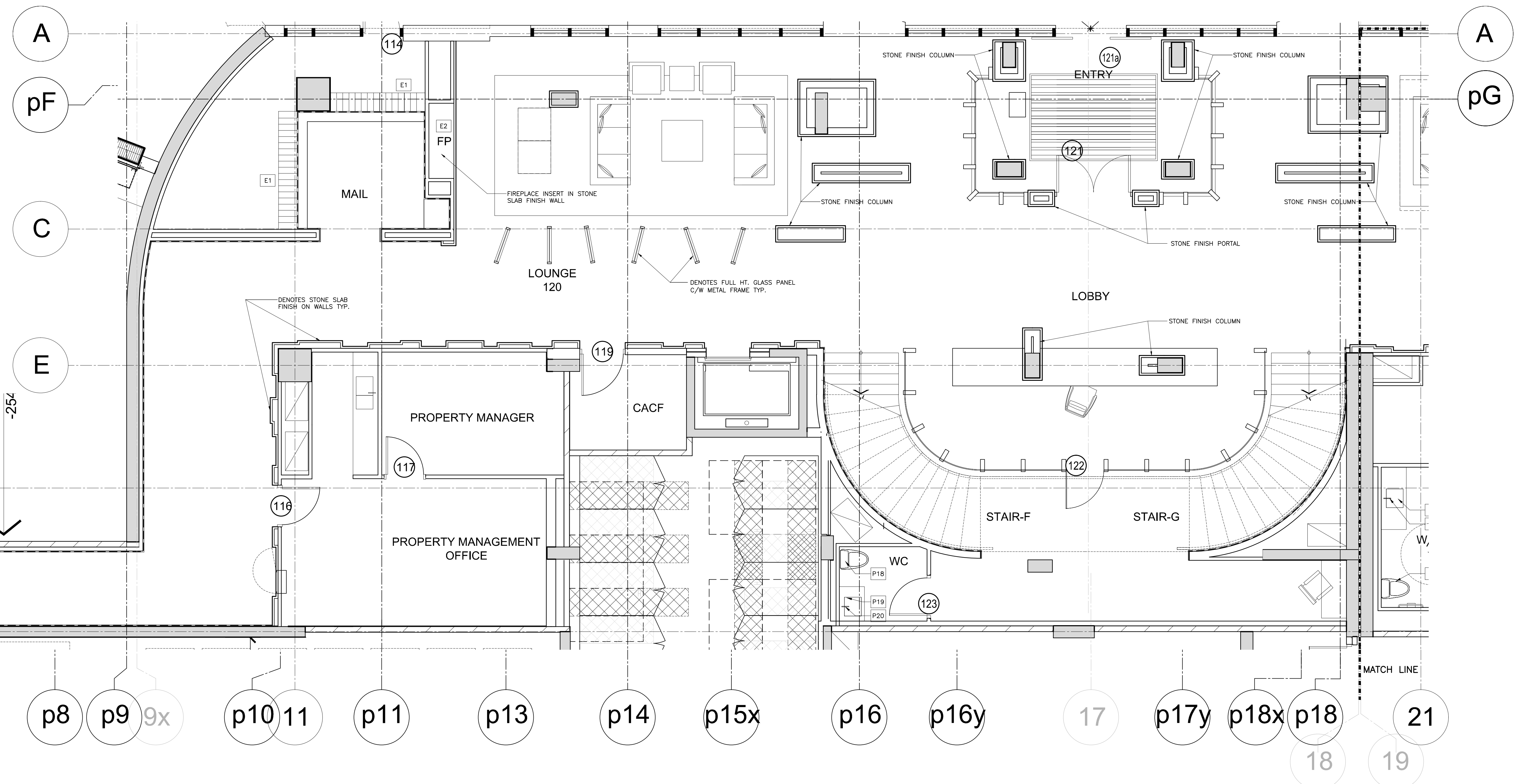
1 GROUND FLOOR PARTITION FURNITURE PLAN (BUILDING-C) ID1.1 SCALE= 1:50
