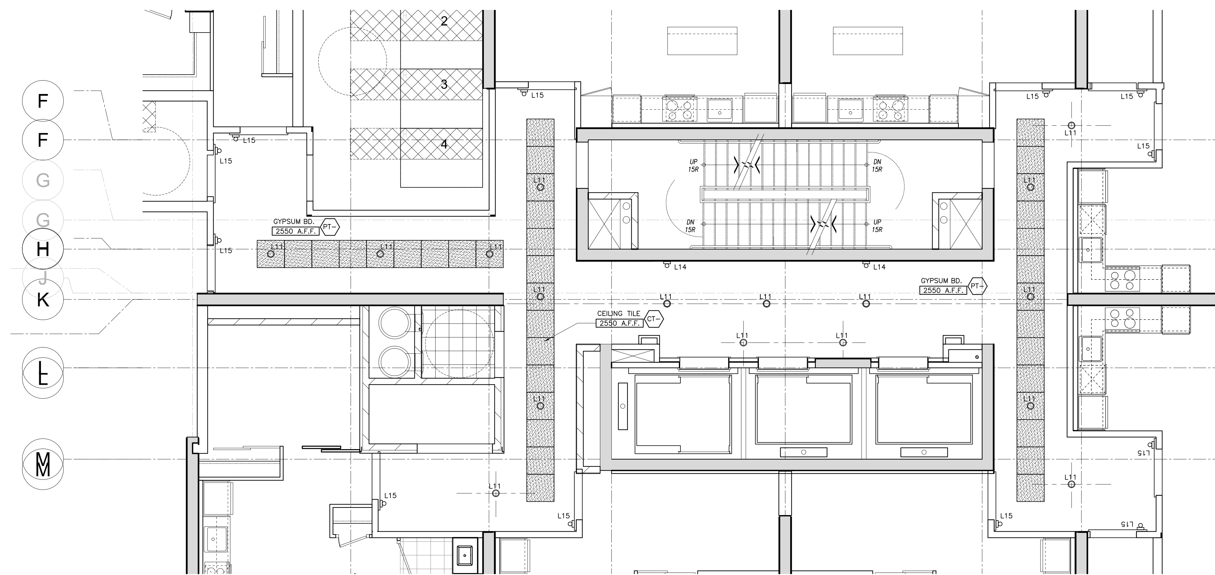
4 8th FLOOR CORRIDOR RCP (BUILDING-D) ID3.5 SCALE= 1:50
