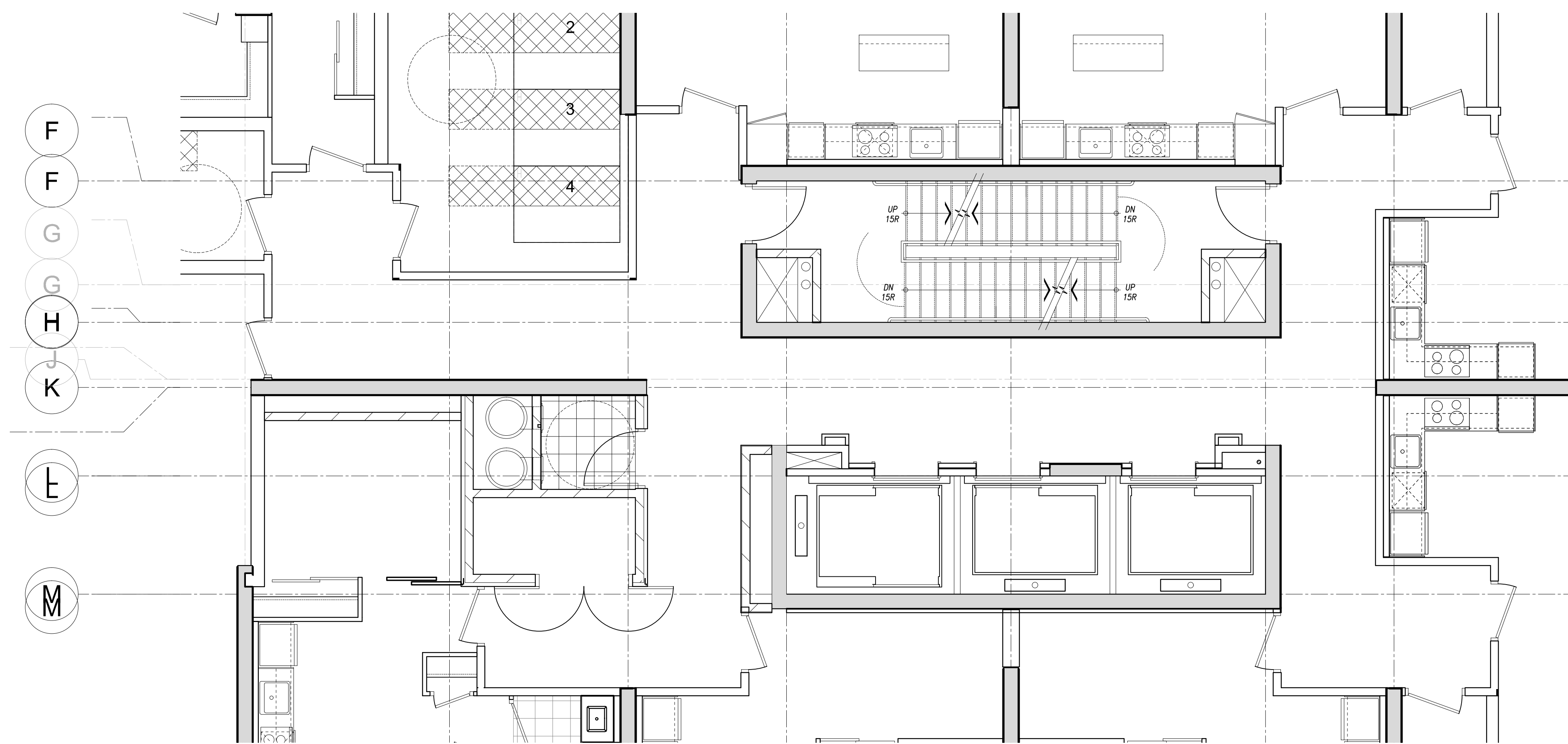
3 8th FLOOR CORRIDOR FINISHES & POWER PLAN (BUILDING-D) ID3.5 SCALE= 1:50
