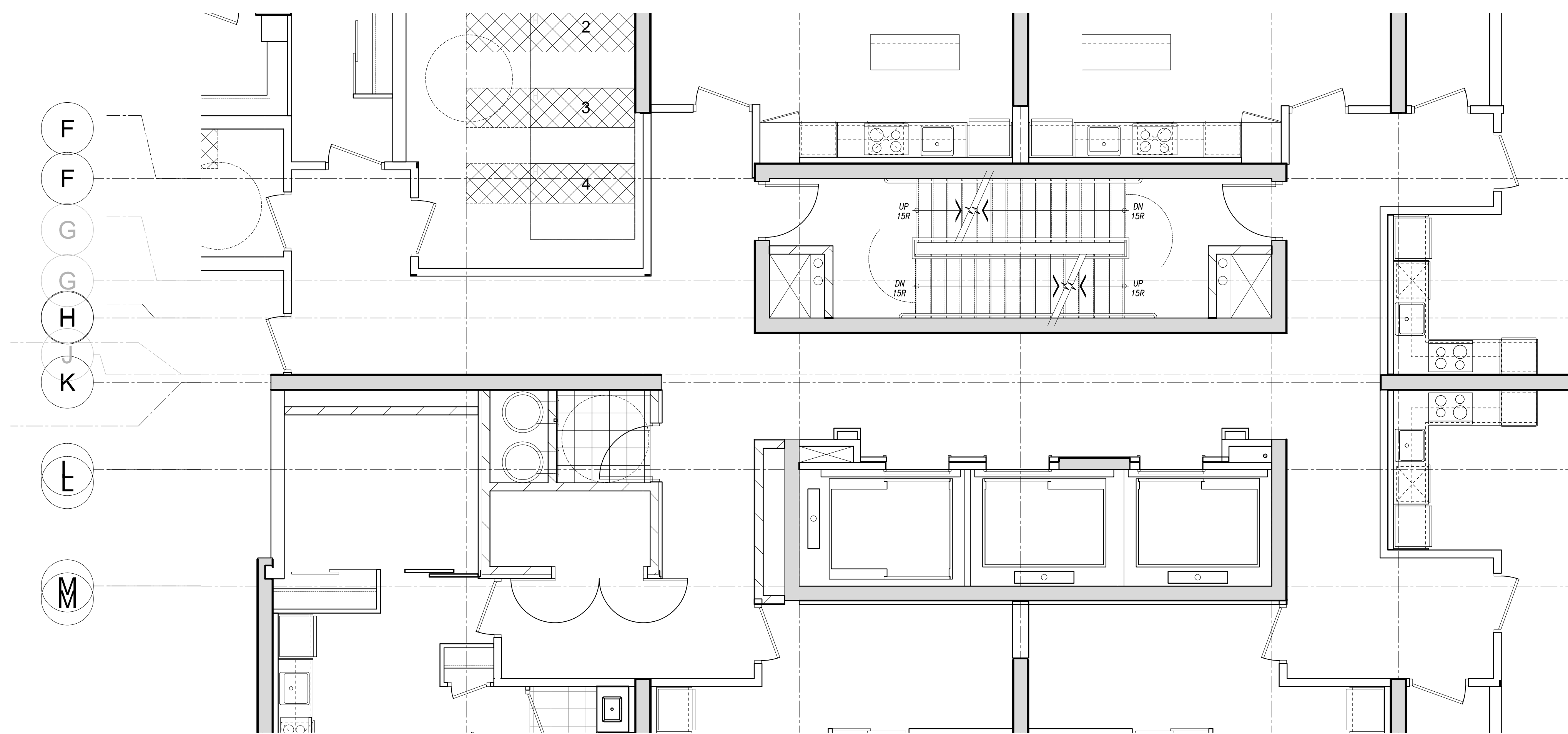
3 4th TO 7th FLOOR CORRIDOR FINISHES & POWER PLAN (BUILDING-D) ID3.4 SCALE= 1:50
