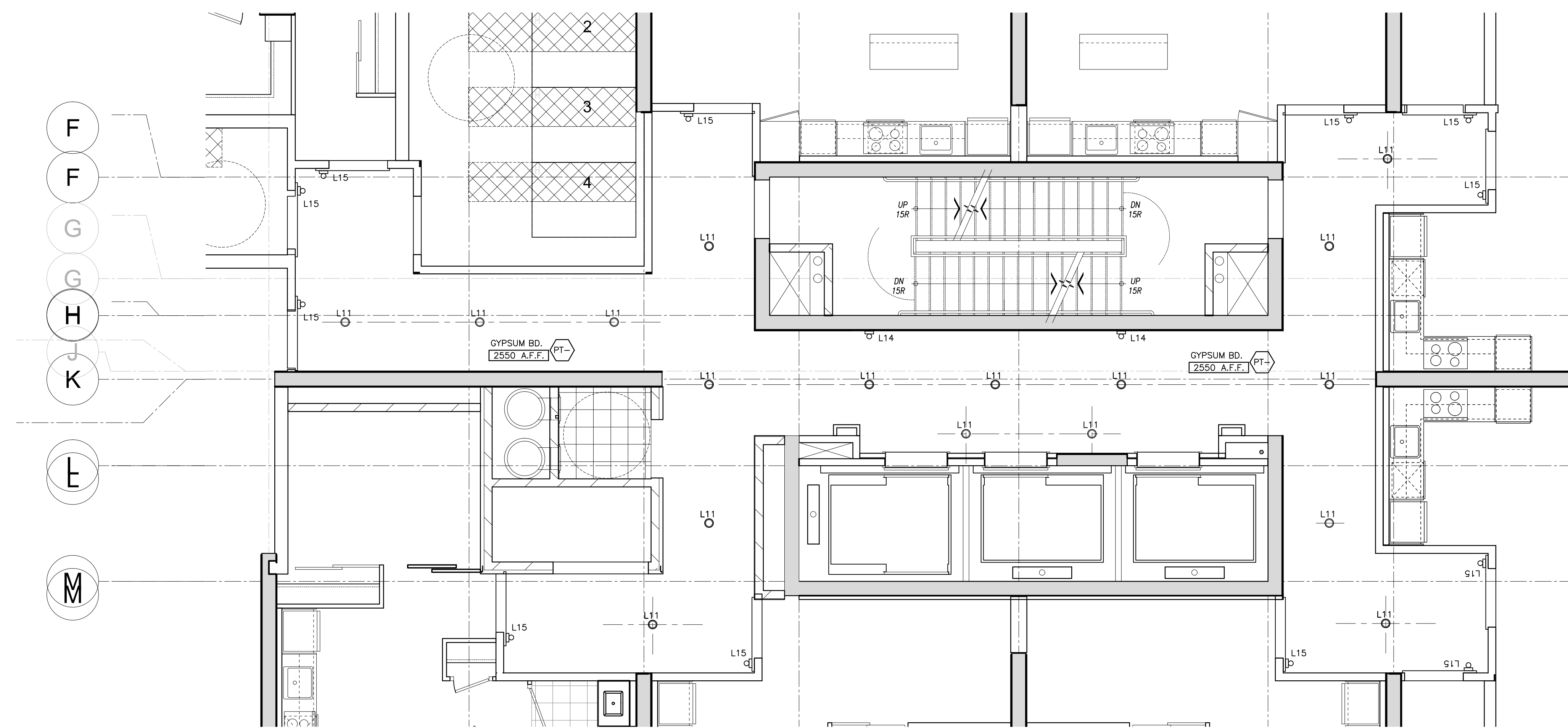
4 4th TO 7th FLOOR CORRIDOR RCP (BUILDING-D) ID3.4 SCALE= 1:50
