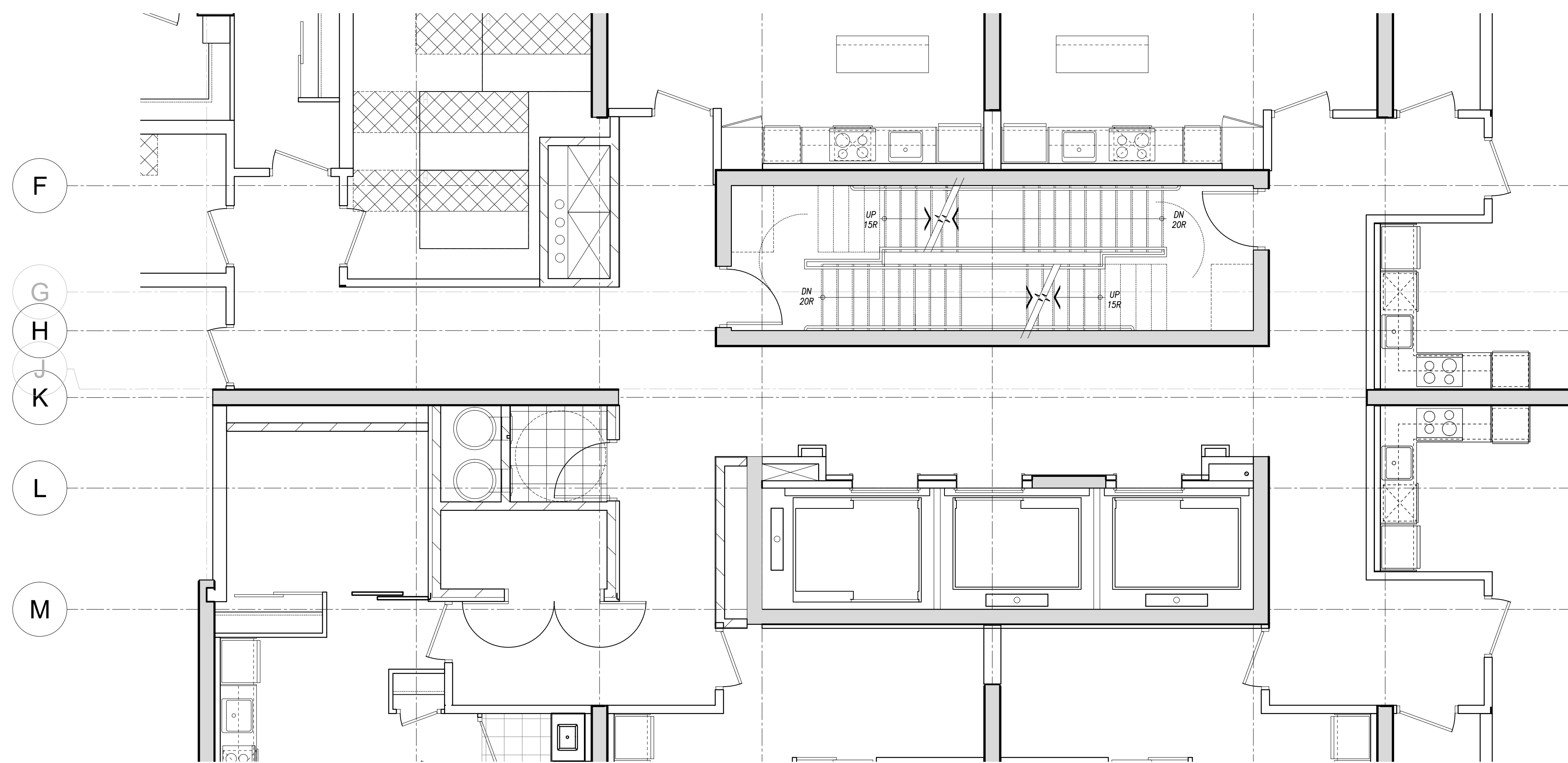
3 3rd FLOOR CORRIDOR FINISHES & POWER PLAN (BUILDING-D) ID3.3 SCALE= 1:50
