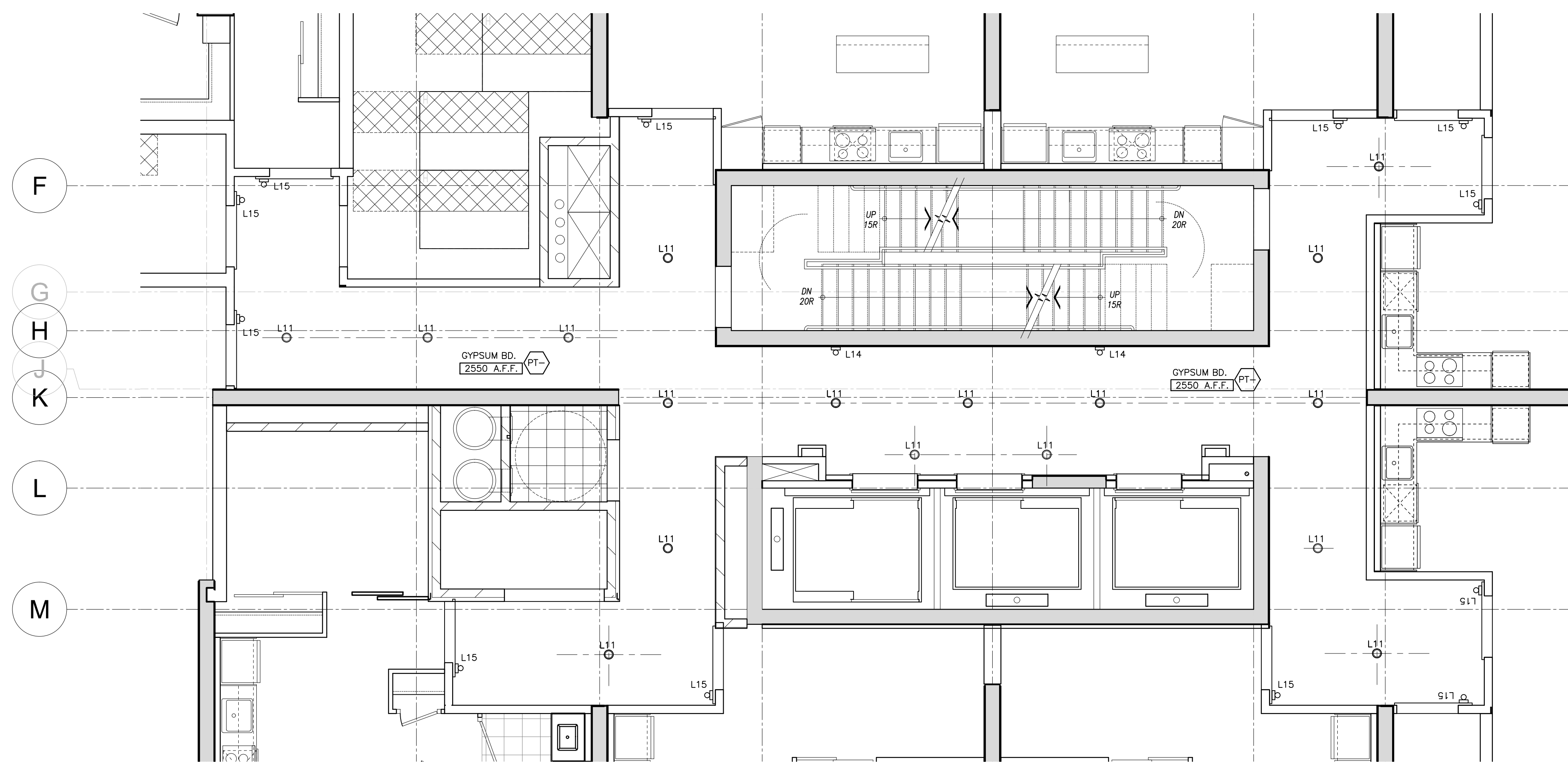
4 3rd FLOOR CORRIDOR RCP (BUILDING-D) ID3.3 SCALE= 1:50
