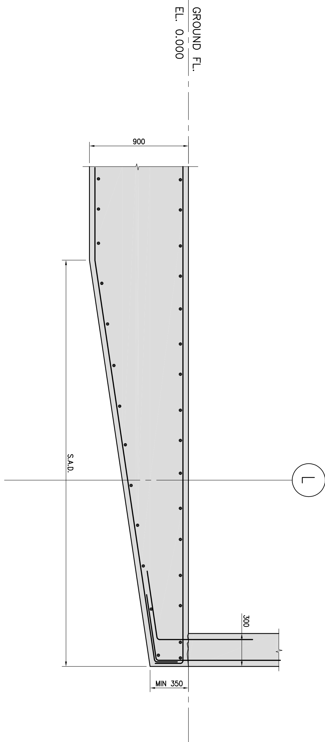
SECTION 5 SCALE 1:20 S-305
