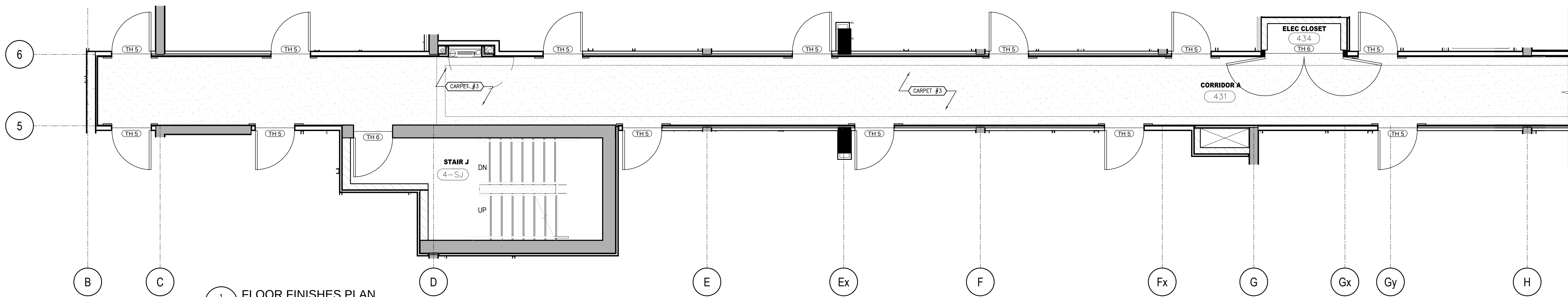
1 FLOOR FINISHES PLAN 4TH FLOOR SCALE 1:50
