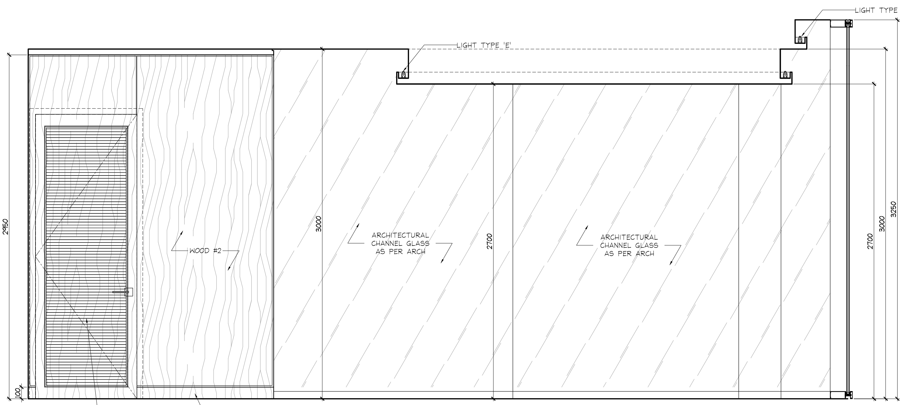
3 ELEVATION 102.1.6 GROUND FLOOR WEIGHT ROOM SCALE 1:20
