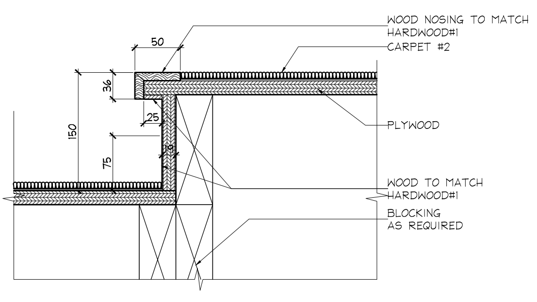
10 SECTION - STEP ID6.0.0 AMENITY - THEATRE ROOM GROUND FLOOR SCALE 1:5
