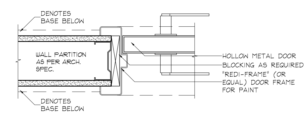
9 TYP. CASING HORIZONTAL SECTION - DETAIL ID6.0.0 SCALE 1:5
