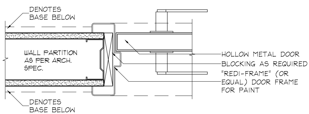
9 TYP. CASING HORIZONTAL SECTION - DETAIL SCALE 1:5
