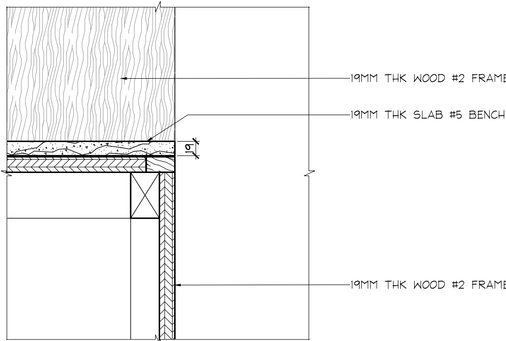
2 DETAIL BENCH CHANGE ROOMS
