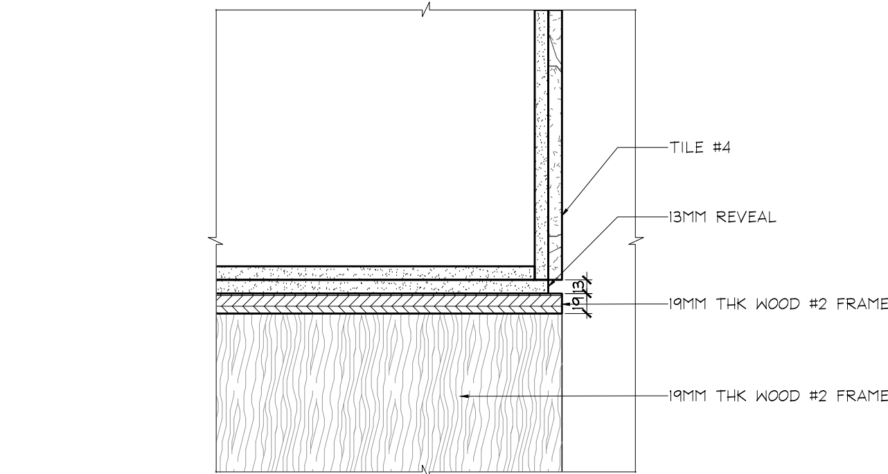
1 DETAIL BENCH CHANGE ROOMS
