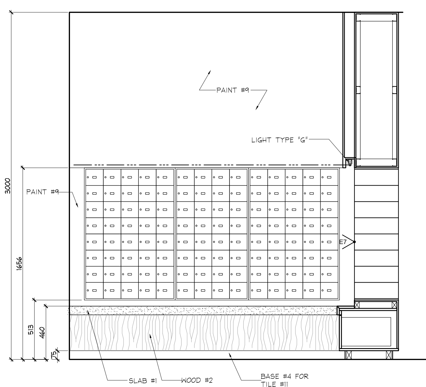
2 ELEVATION ID2.1.2 GROUND FLOOR MAILROOM SCALE 1:20
