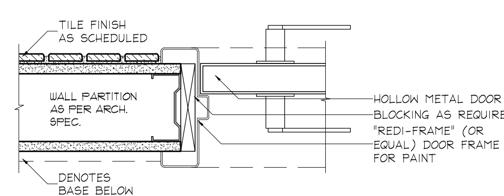
8 TYP. CASING @ TILE WALL HORIZONTAL SECTION - DETAIL ID6.0.0 SCALE 1:5
