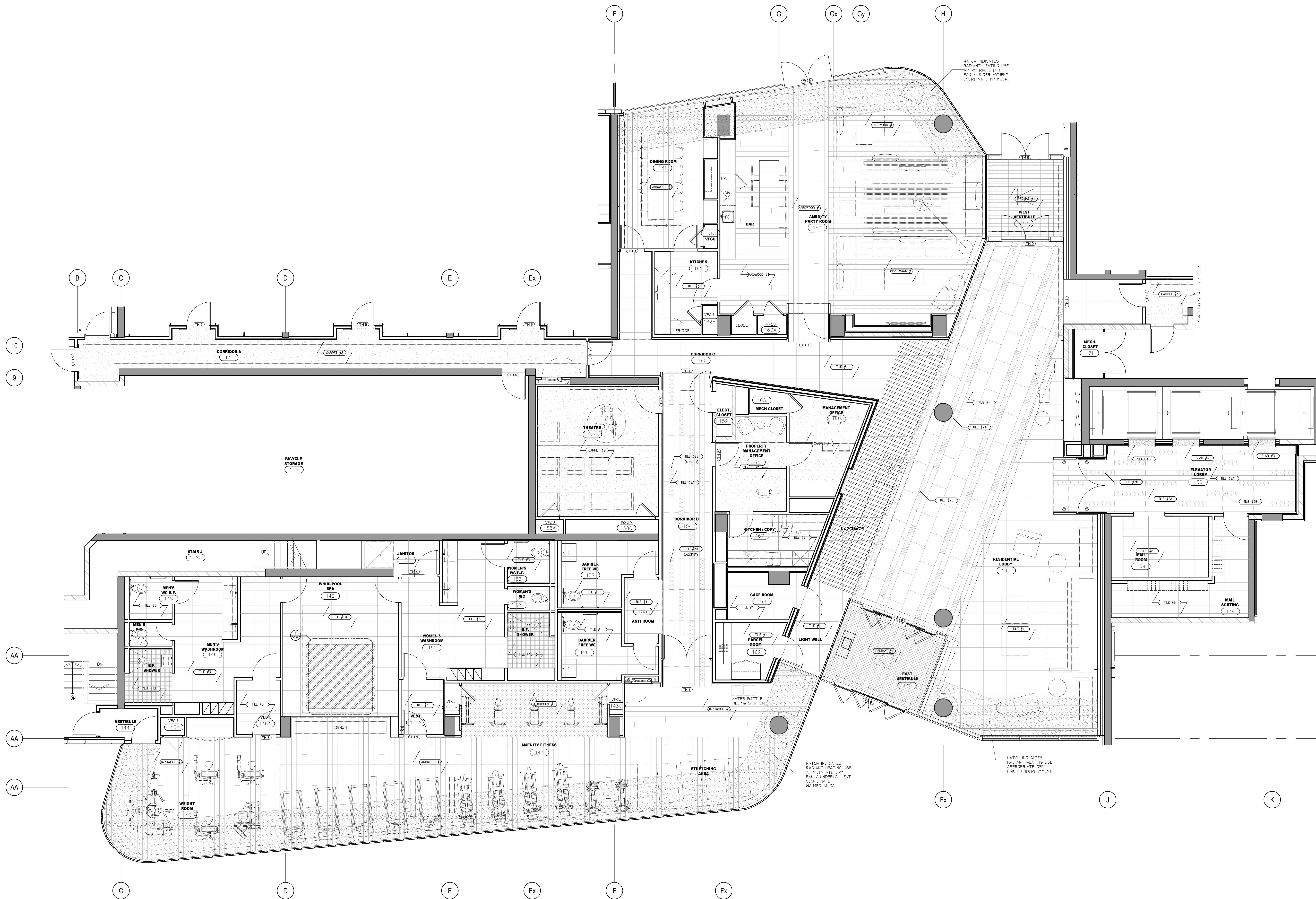
1 FLOOR FINISHES PLAN GROUND FLOOR SCALE: 1:50
