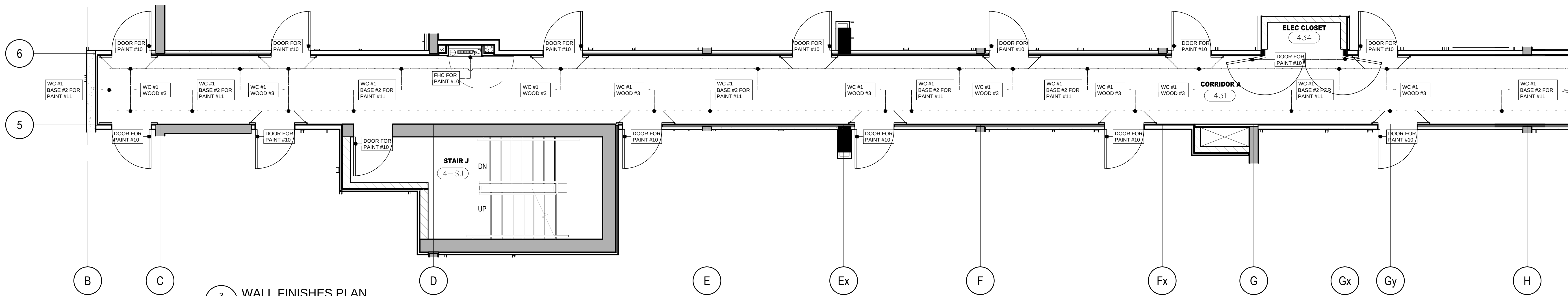
3 WALL FINISHES PLAN 4TH FLOOR SCALE 1:50 ID1.4.1
