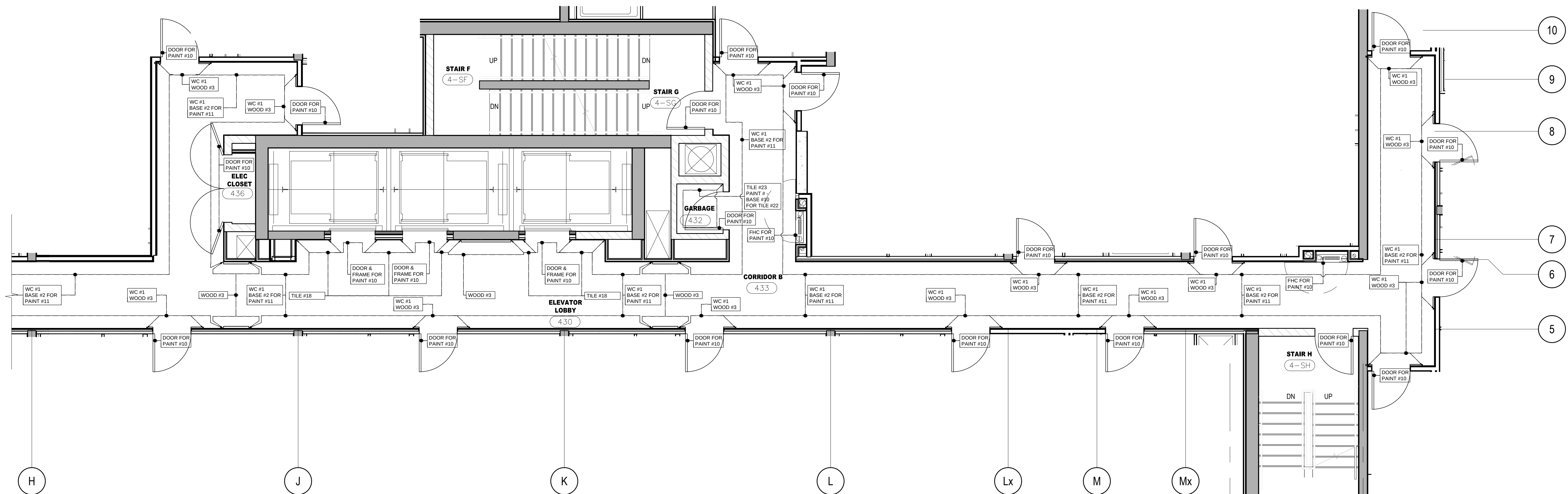
4 WALL FINISHES PLAN 4TH FLOOR SCALE 1:50 ID1.4.1
