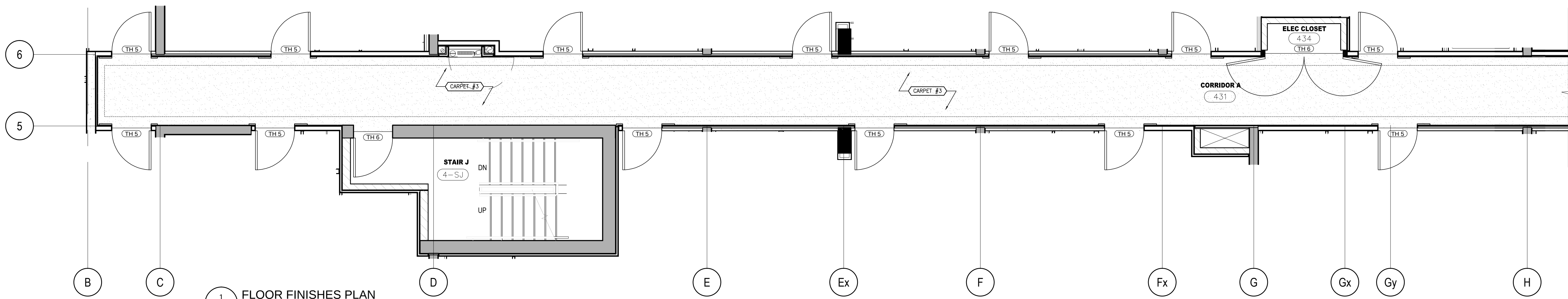
1 FLOOR FINISHES PLAN 4TH FLOOR SCALE 1:50 ID1.4.1
