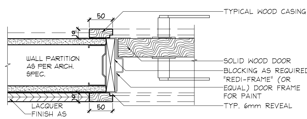
6 TYP. CASING @ TILE WALL HORIZONTAL SECTION - DETAIL SCALE 1:5
