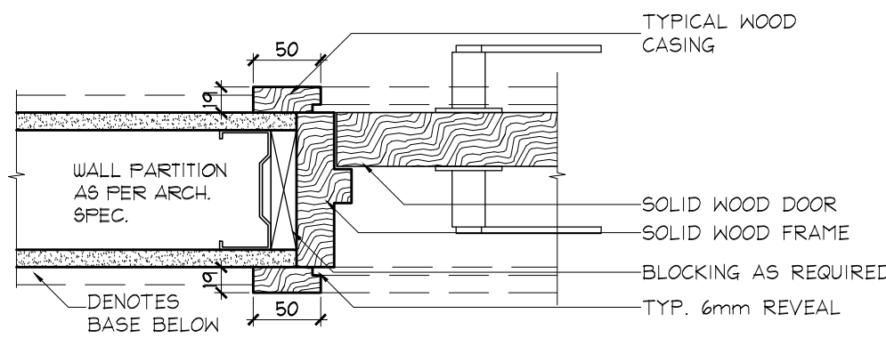
4 TYP. CASING HORIZONTAL SECTION - DETAIL SCALE 1:5
