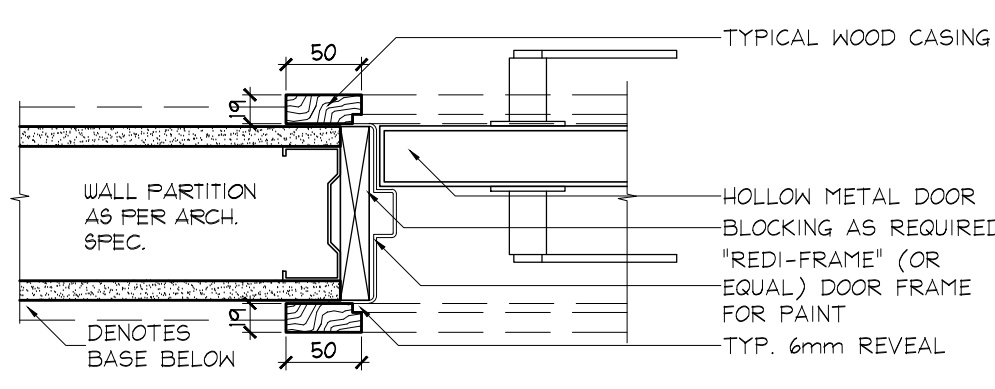
5 TYP. CASING HORIZONTAL SECTION - DETAIL SCALE 1:5
