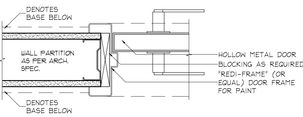
9 TYP. CASING HORIZONTAL SECTION - DETAIL SCALE 1:5
