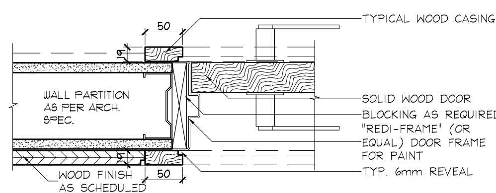
7 TYP. CASING @ WOOD HORIZONTAL SECTION - DETAIL SCALE 1:5
