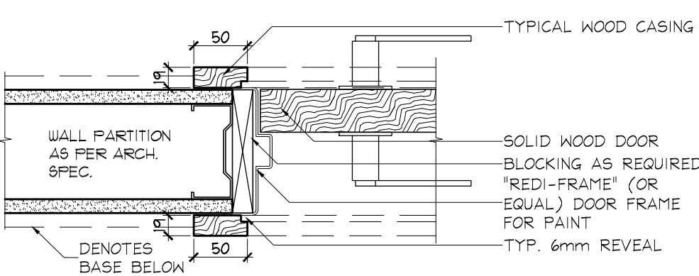
3 TYP. CASING HORIZONTAL SECTION - DETAIL SCALE 1:5
