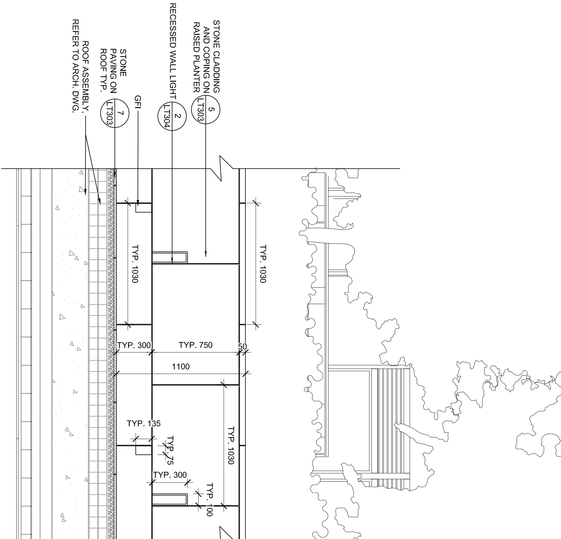
2 RAISED PLANTER - FRONT VIEW SCALE: 1:20
