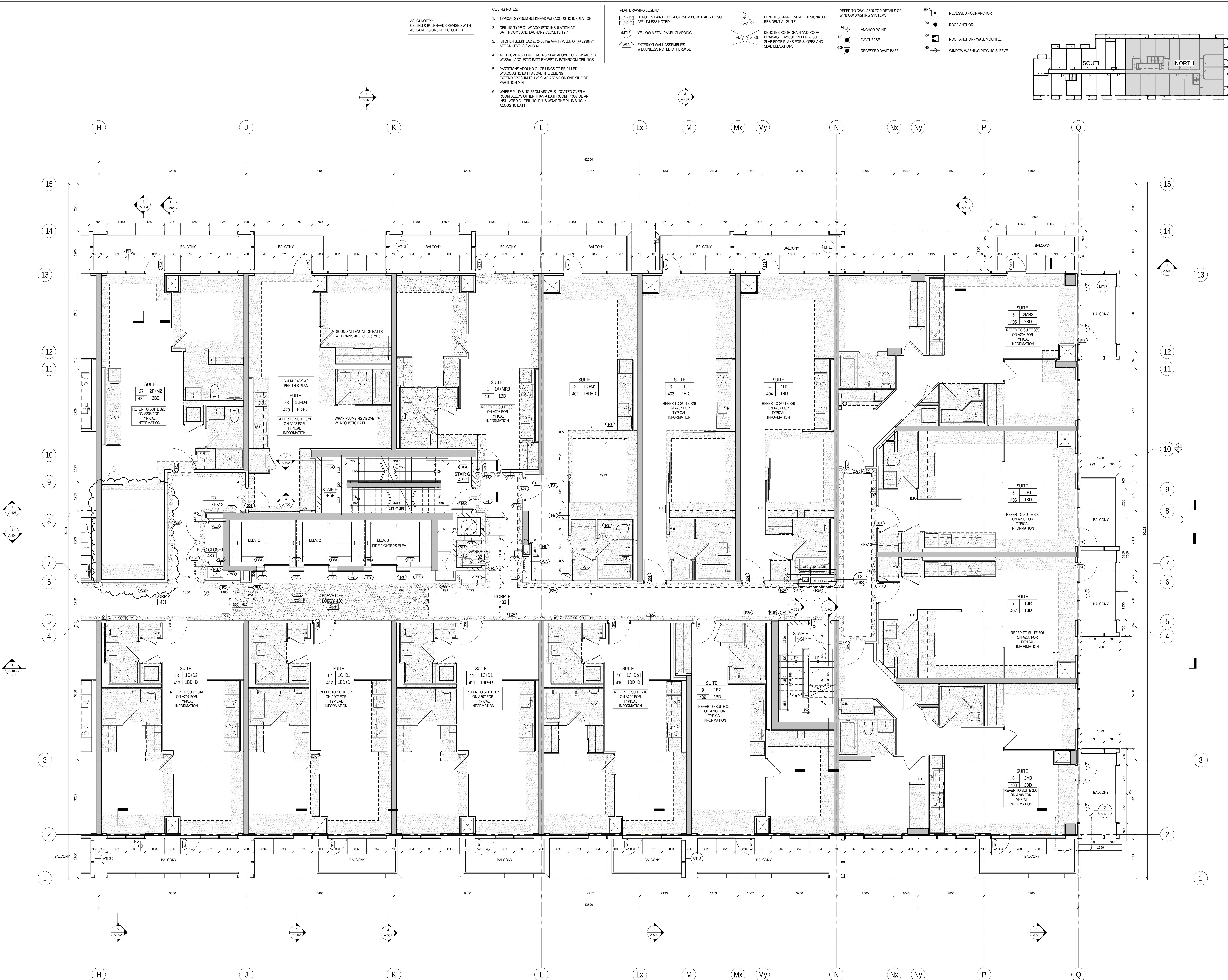
1 LEVEL 4 PLAN NORTH 1/A227 1:50
