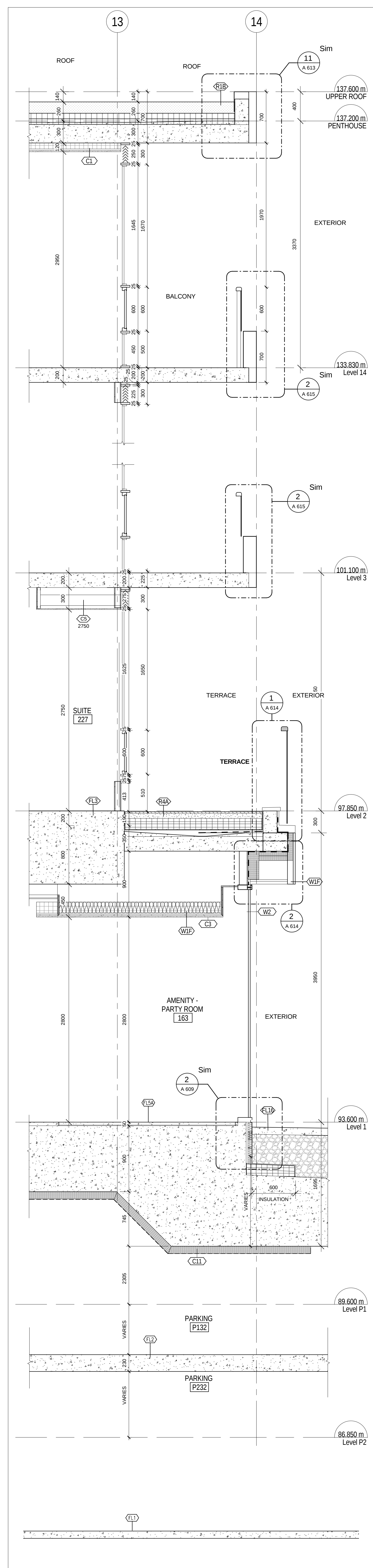
2 WEST WALL SECTION - AMENITY W/TERRACE ABOVE A 504 1:25
