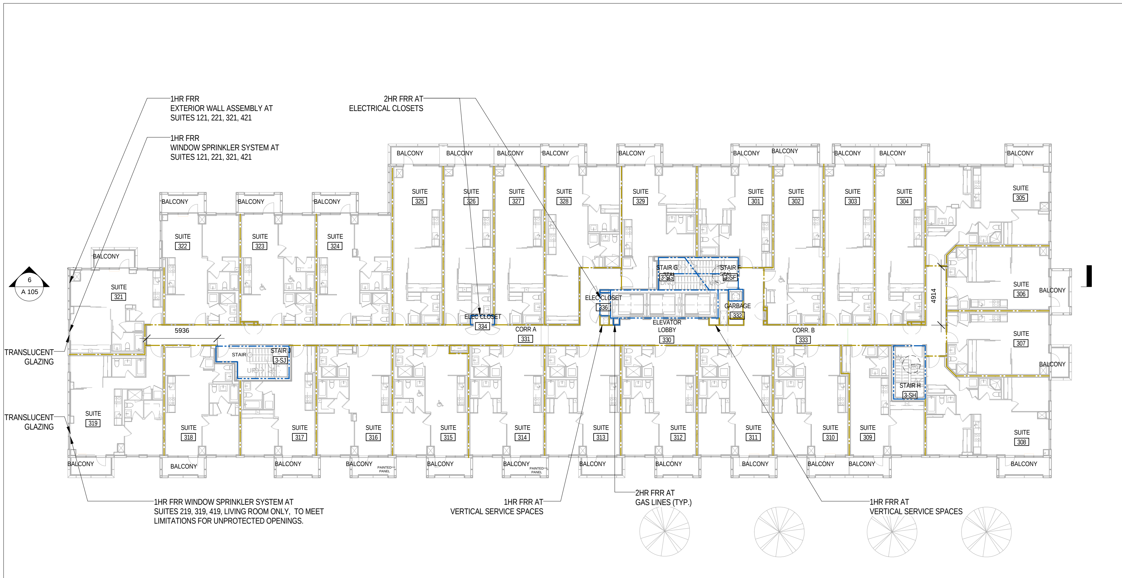
3 A 103 L3 - LIFE SAFETY PLAN 1:200
