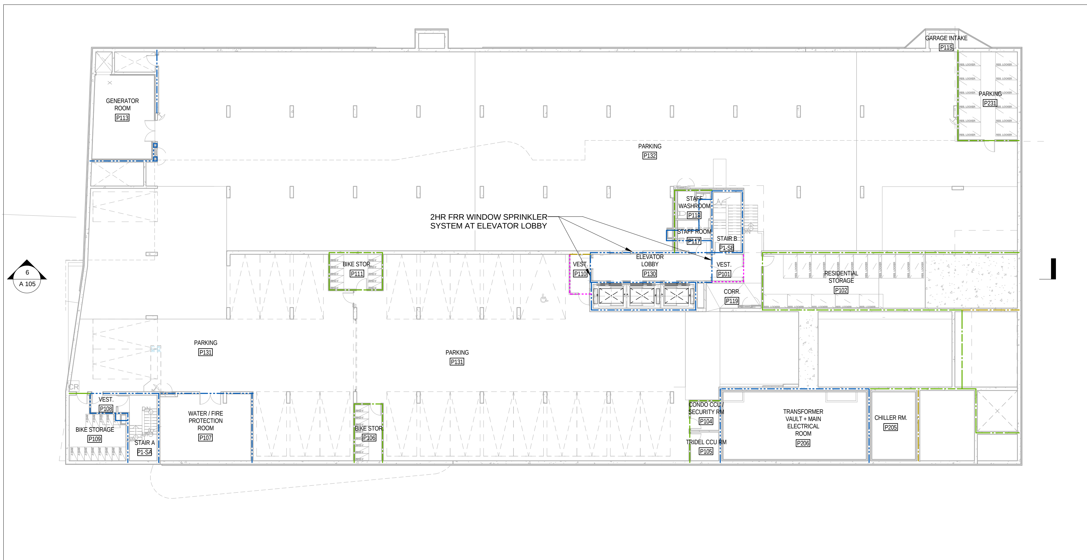
1 A 103 P1 - LIFE SAFETY PLAN 1:200
