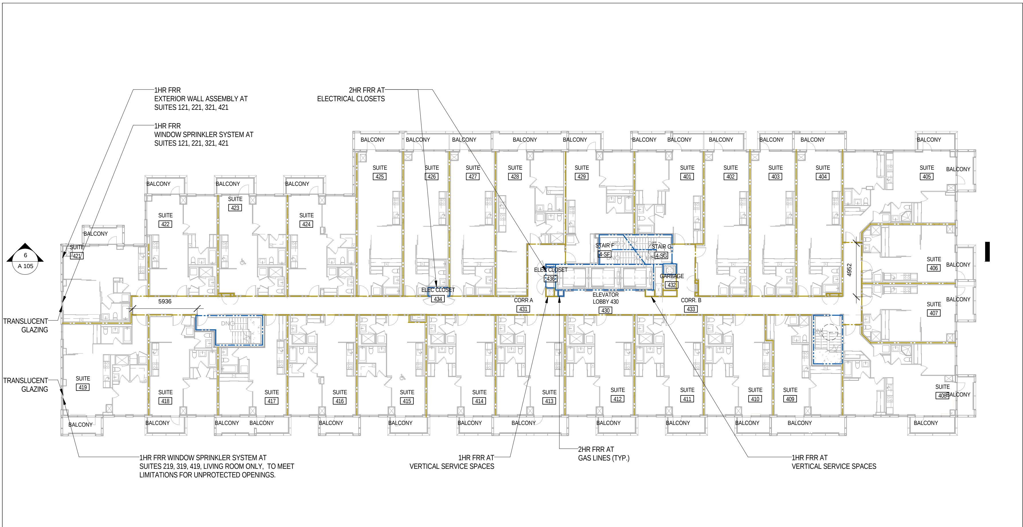
6 A 103 L4 - LIFE SAFETY PLAN 1:200
