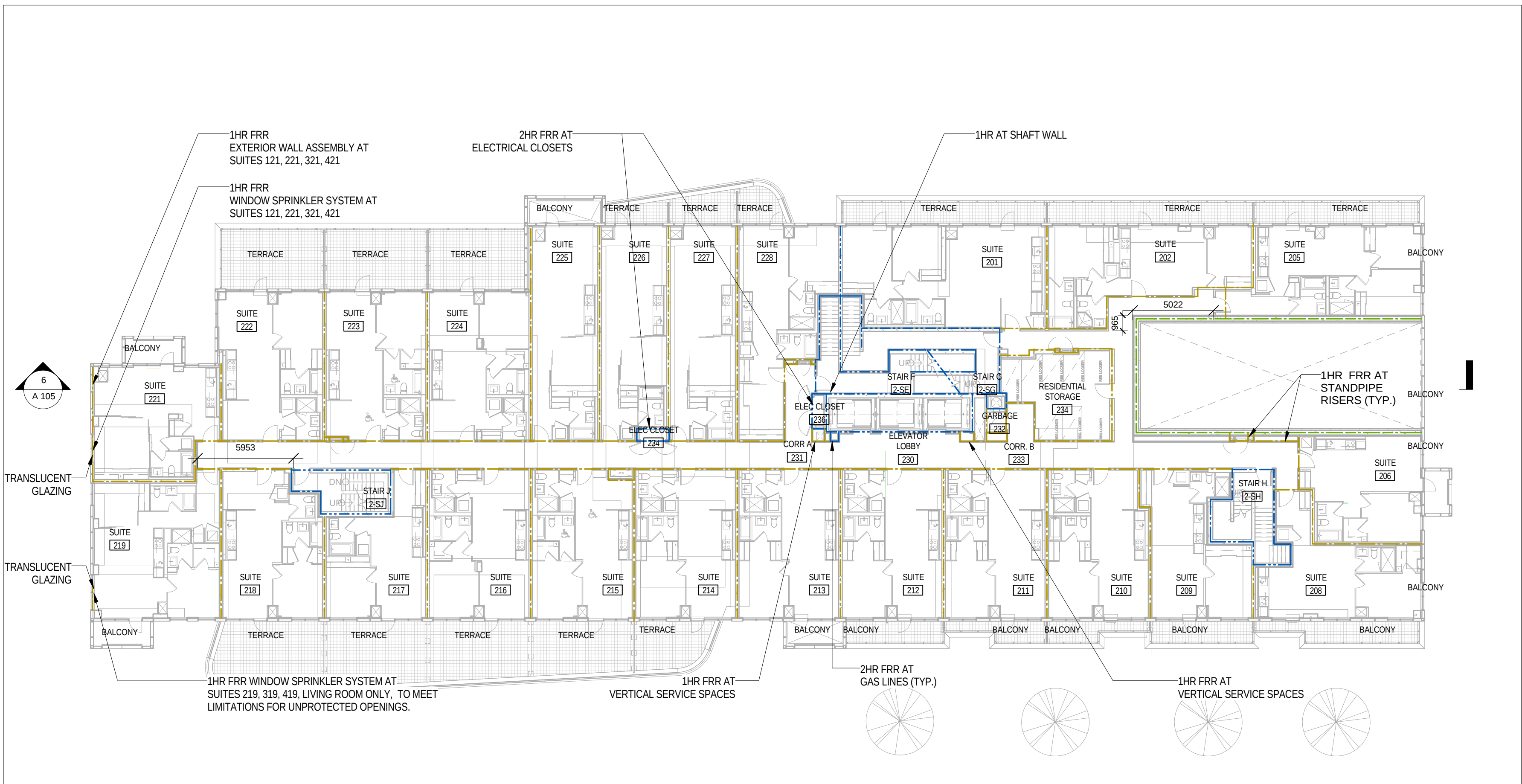
5 A 103 L2 - LIFE SAFETY PLAN 1:200
