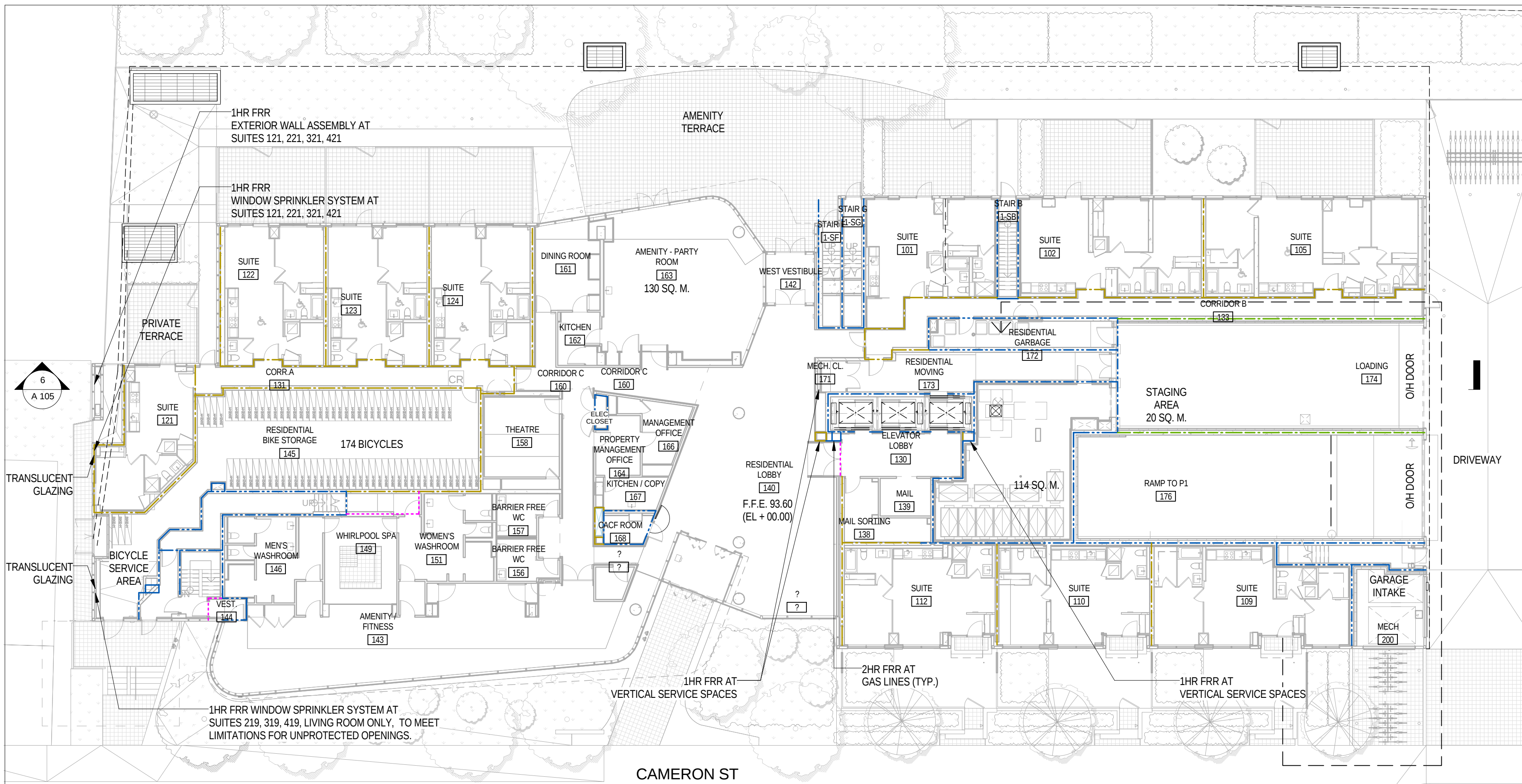
2 A 103 L1 - LIFE SAFETY PLAN 1:200
