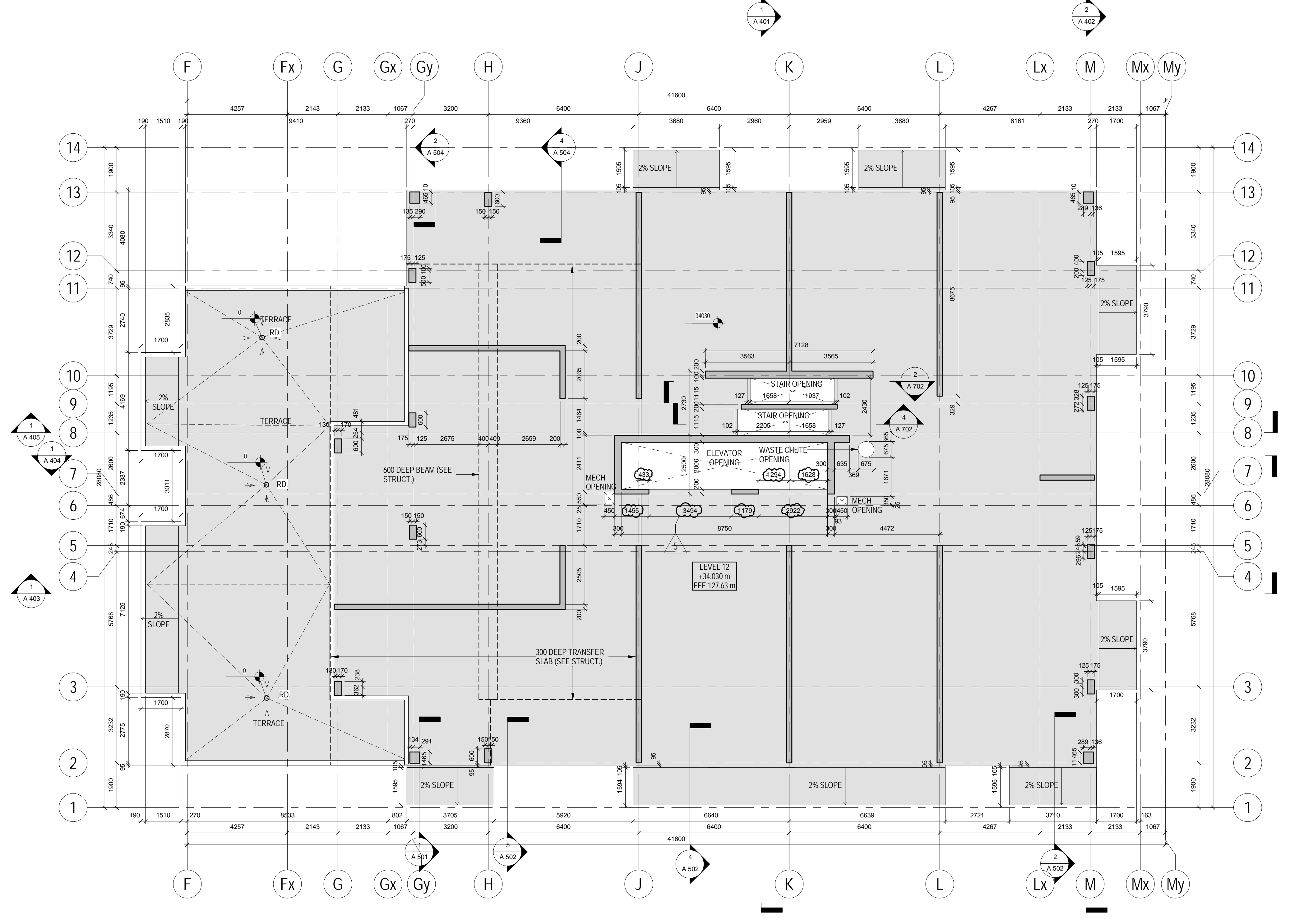
2 Level 12 EOS A 258 1:100
