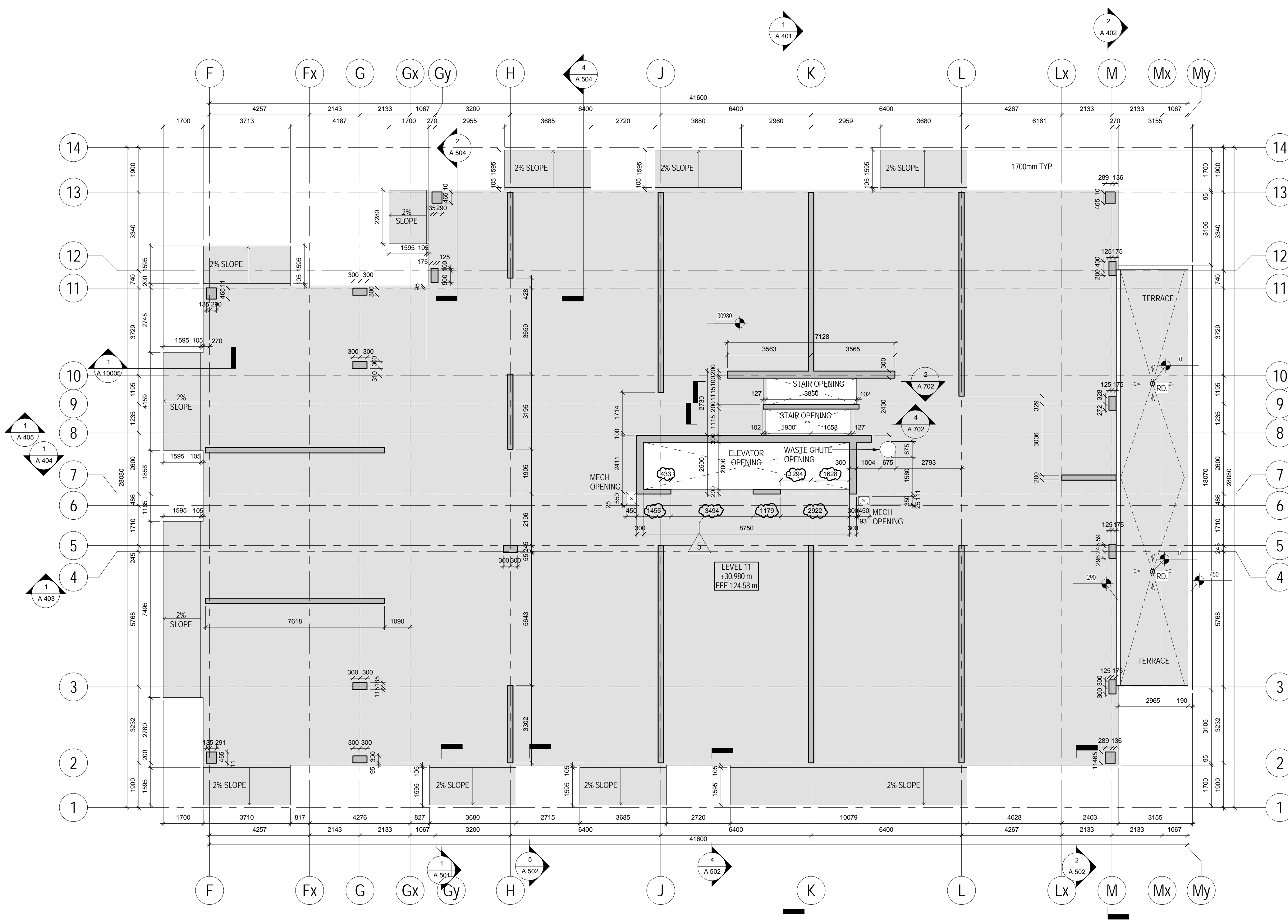
1 Level 11 EOS A 258 1:100
