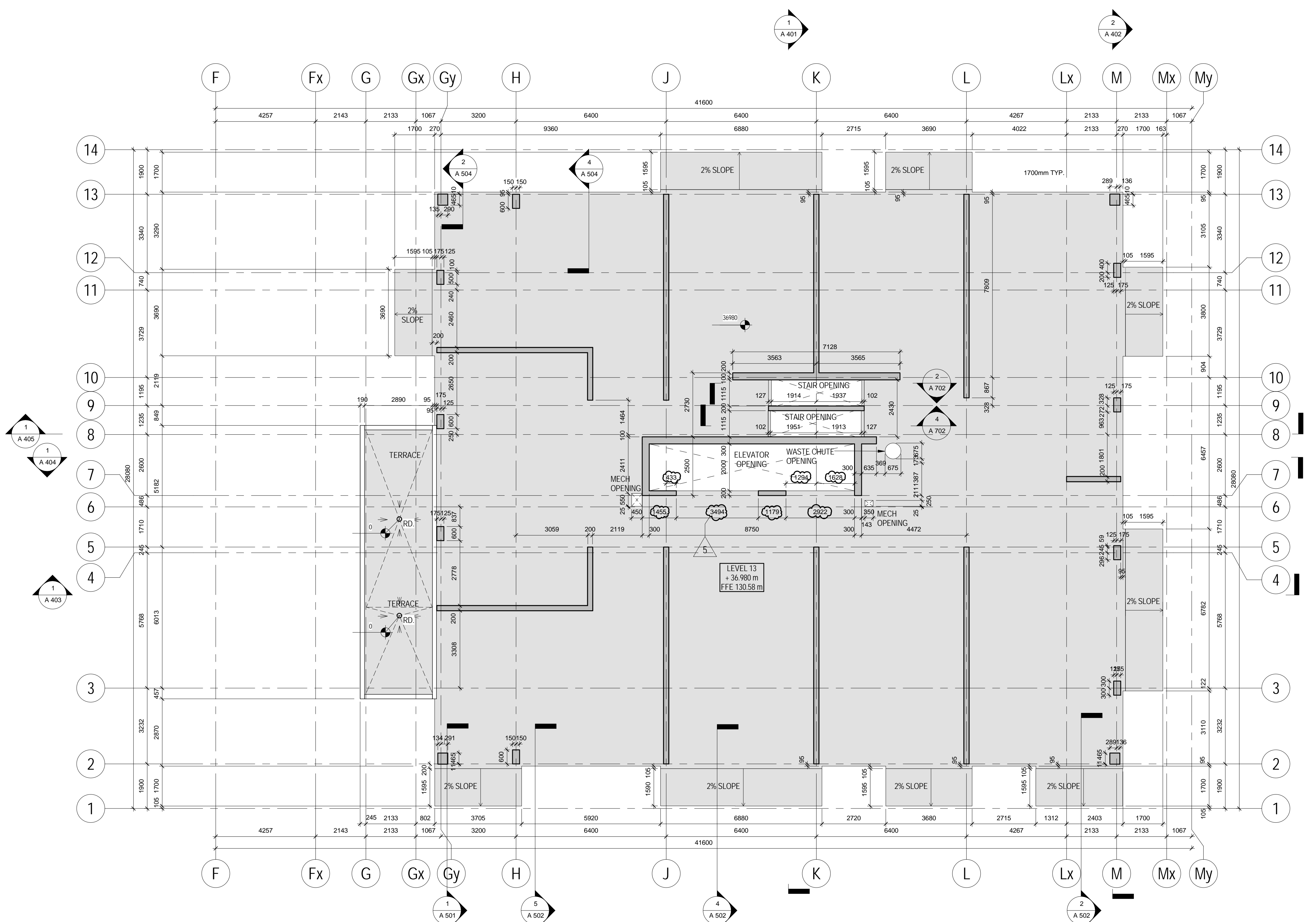
3 Level 13 EOS A 258 1:100
